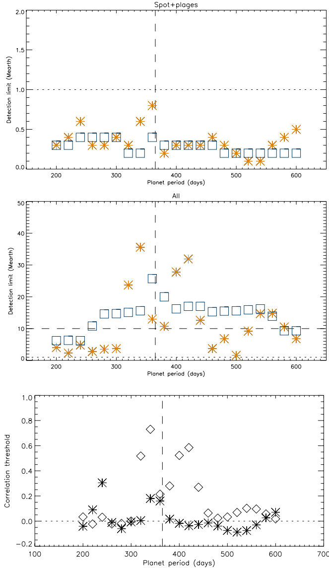
Fig. 8. Upper panel: detection limits versus planet period for RV_{\text{spl}} (Set 1, no RV noise, daily sampling). Detection limits are computed using the correlation-based method (stars, orange), and the LPA method (squares, blue). Middle panel: same for RV_{\text{tot}} . Lower threshold: correlation threshold for RV_{\text{spl}} (stars) and RV_{\text{tot}} (diamonds). The vertical dashed lines indicate the one-year period position.
