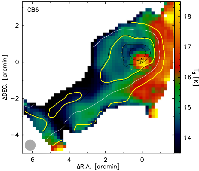
Fig. B.2. Dust temperature map of CB 6 (color scale), overlaid with contours of the hydrogen column density (white: 10^{21} cm ^{-2} , black: 2, 4, and 6 \times 10^{21} cm ^{-2} ). Yellow contours mark N_{\text{out}} (Eq. (3)) and N_{1'} (Eq. (10)). The dotted yellow ellipse marks the N_{1'} approximation described in Sect. 5.3. The asterisk marks the position of the embedded YSO.
