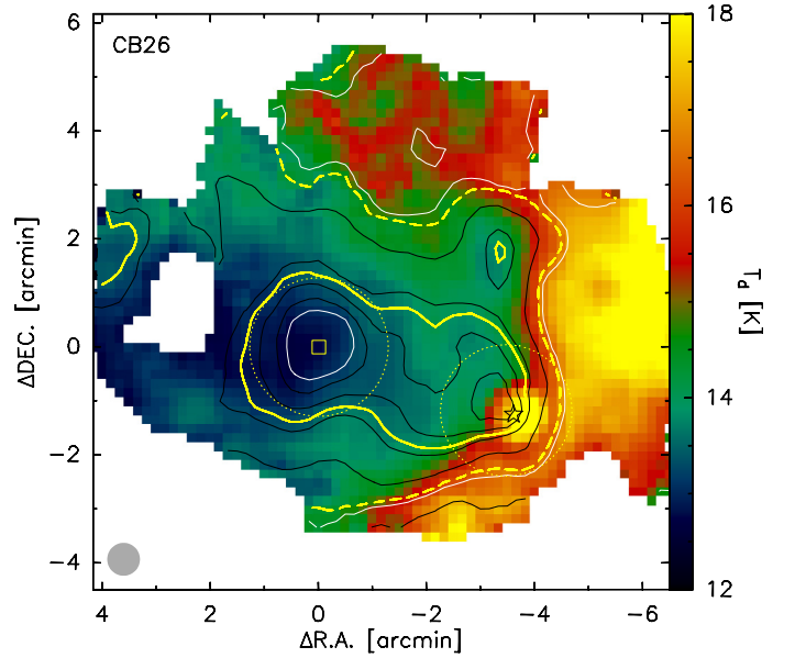
Fig. B.4. Dust temperature map of CB 26 (color scale), overlaid with contours of the hydrogen column density (white: 10^{21} and 10^{22} cm ^{-2} , black: 0.5, 2, 4, 6, and 8 \times 10^{21} cm ^{-2} ). Yellow contours mark N_{\text{out}} (Eq. (3)) and N_{1'} (Eq. (10), referring to the starless core SMM2). Dotted yellow ellipses mark the N_{1'} approximations for the two subcores described in Sect. 5.3. The yellow square marks the column density peak and position of CB 26-SMM2; the asterisk marks the position of CB 26-SMM1 (Table 5).
