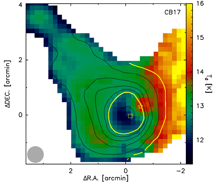
Fig. B.3. Dust temperature map of CB 17 (color scale), overlaid with contours of the hydrogen column density (white: 10^{21} – masked by the yellow N_{\text{out}} contour – and 10^{22} cm ^{-2} , black: 2, 4, 6, 8, and 20 \times 10^{21} cm ^{-2} ). Yellow contours mark N_{\text{out}} (Eq. (3)) and N_{1'} (Eq. (10)). The yellow square marks the column density peak and position of CB 17-SMM. The asterisk marks the position of CB 17-IRS (Table 5; see also Launhardt et al. 2010).
