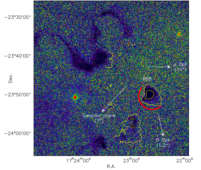
Fig. C.8. B 68: visual (red) DSS1 image with SPIRE 500 \mu\text{m} continuum contours overlaid. The red arc marks the warm rim of B 68. The B2IV star \Theta Oph is located at a distance from the Sun of 134 pc, i.e., its physical distance from B 68 is only \approx 2.8 pc.
