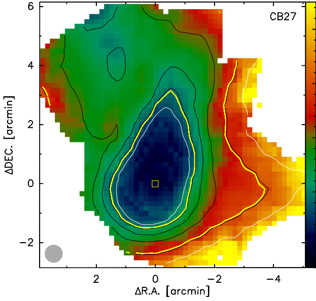
Fig. B.5. Dust temperature map of CB 27 (color scale), overlaid with contours of the hydrogen column density (white: 10^{21} and 10^{22} \text{cm}^{-2} , black: 2, 4, 6, and 8 \times 10^{21} \text{cm}^{-2} ). Yellow contours mark N_{\text{out}} (Eq. (3)) and N_{1'} (Eq. (10)). The yellow square marks the column density peak and the reference position listed in Table 5.
