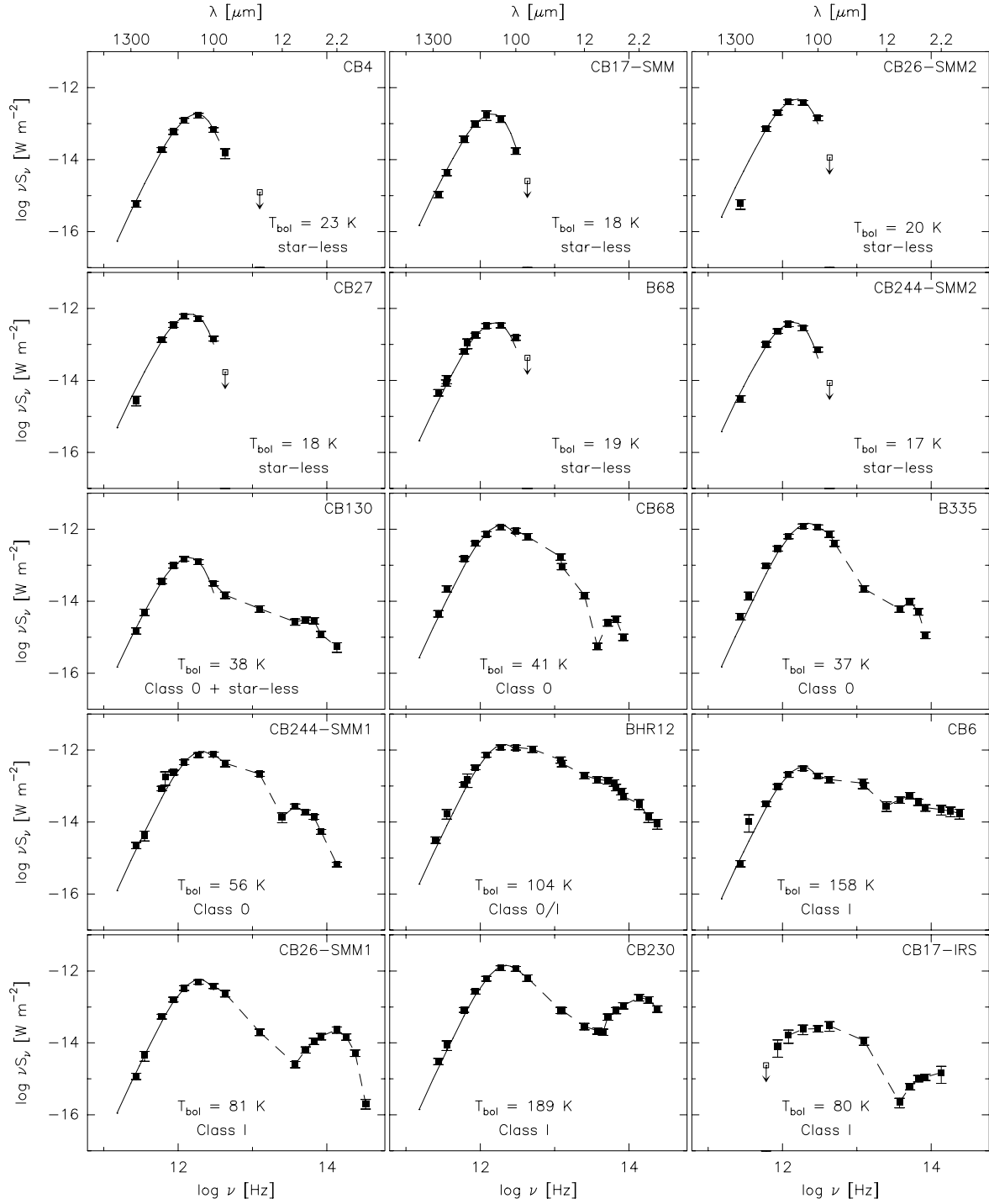
Fig. 4. Integrated spectral energy distributions of the dense cores and embedded sources listed in Table 6. Fluxes are integrated within the N_1 contour (Eq. (10)), as are the core masses and luminosities listed in Table 6. Solid lines between 3 mm and 100 \mu\text{m} mark the modified blackbody fits to the data points, while dashed lines only represent a logarithmic interpolation of the data points shortward of 100 \mu\text{m} (see Sect. 5.3).
