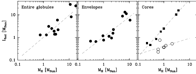
Fig. 7. Bolometric luminosity vs. total hydrogen mass of the entire globules ( left ), the envelopes only (without the dense cores; center ) and the dense cores only ( right ; see Table 6 and Sect. 5.6). Filled squares in the right-most panel mark protostellar cores, empty circles mark starless cores, and the open square marks the core of CB 130 with the embedded VeLLO.
