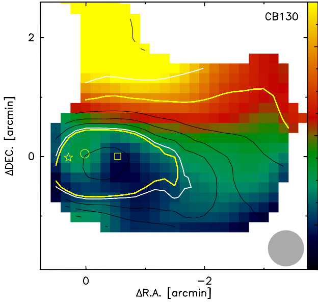
Fig. B.9. Dust temperature map of CB 130 (color scale), overlaid with contours of the hydrogen column density (white: 10^{21} and 10^{22} \text{cm}^{-2} , black: 0.5, 2 – masked by yellow N_{\text{out}} contour – 4, 6, 8, and 20 \times 10^{21} \text{cm}^{-2} ). Yellow contours mark N_{\text{out}} (Eq. (3)) and N_{1'} (Eq. (10)). The yellow circle marks the position of the protostellar core CB 130-SMM1 with the embedded Class 0 VeLLO. The yellow square marks the position of the secondary starless core CB 130-SMM2. The asterisk marks the position of the Class I-II YSO CB 130-IRS, which most likely associated with CB 130, but not embedded in its dense core (see Launhardt et al. 2010).
