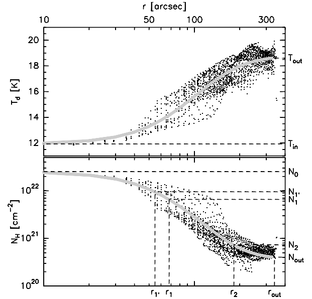
Fig. 3. Radial profiles of column density and LoS-averaged dust temperature of B 68 (cf. Fig. 9 of Nielbock et al. 2012 for the ray-tracing results of the same data). Small black dots show the data pixel values over radial distance from the column density peak (see Fig. B.8). Solid gray lines show best fits to these data with Eqs. (3) and (8) and the parameters listed in Table 5. The parameters are also labeled on the diagram axes to illustrate their meaning, with the following characteristic radii: r_1 = flat core profile radius (Eq. (3)), r_{1'} = radius to define consistent dense core boundary (Eqs. (10) and (11)), r_2 = cloud radius at transition to halo (Eq. (6)), and r_{\text{out}} = outer cloud boundary (Eq. (3)).
