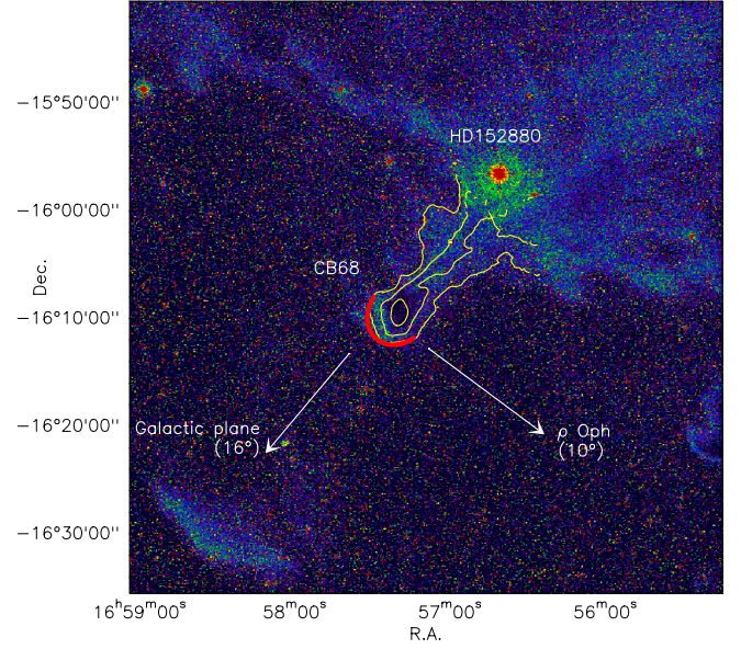
Fig. C.7. CB 68: visual (red) DSS2 image with SPIRE 500 \mu\text{m} continuum contours overlaid. The red arc marks the warm rim of CB 68.
