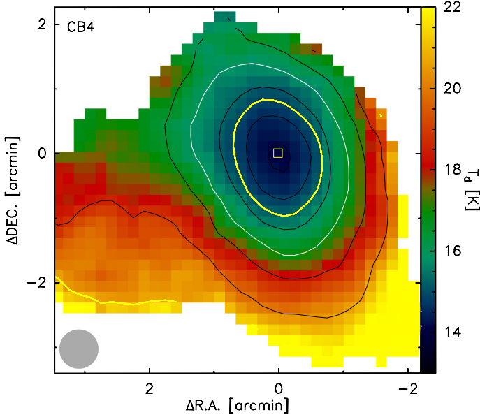
Fig. B.1. Dust temperature map of CB 4 (color scale), overlaid with contours of the hydrogen column density (white: 10^{21} cm ^{-2} , black: 0.2, 0.5, 2, and 4 \times 10^{21} cm ^{-2} ). Yellow contours mark N_{\text{out}} (Eq. (3)) and N_{1'} (Eq. (10)). The yellow square marks the column density peak and the reference position listed in Table 5.
