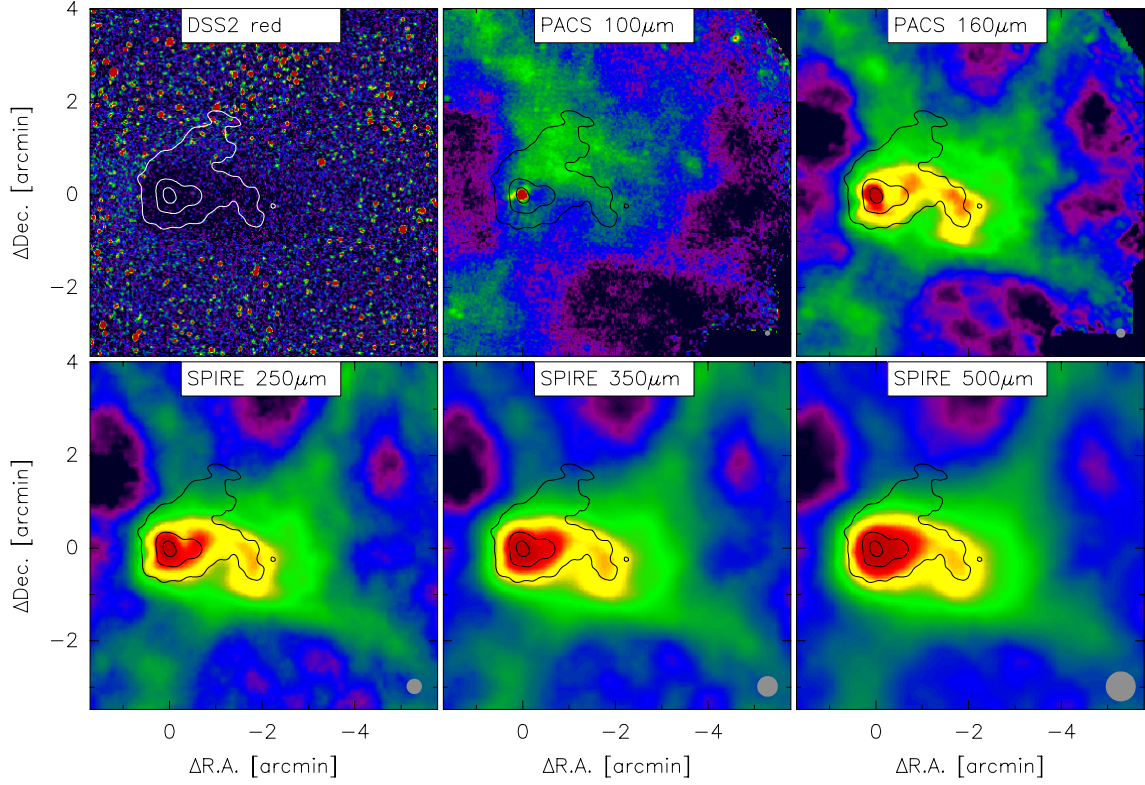
Fig. A.9. CB 130 (Class 0 protostar): visual (red) DSS2 image and Herschel FIR maps (color; log scale) at 100, 160, 250, 350, and 500 \mu\text{m} , with 1.2 mm continuum contours overlaid (20, 60, and 100 mJy/20'' beam). Herschel beam sizes are indicated as gray circles in the lower right corners.
