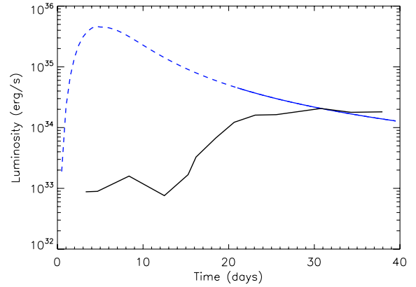
Fig. 10. Predicted thermal X-ray light curve for Run 3 (in blue), compared to that inferred from Swift /XRT (in black, reproduced from Orlando & Drake 2012). A comparison with the results of multi-dimensional hydrodynamical simulations showed that our model is unable to account for the complexity of the emission rise. Only the average luminosity past three weeks, the solid part of the curve, was therefore used as a constraint on the non-thermal processes.
