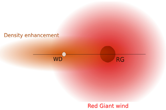
Fig. 1. Illustration of the density structure adopted for the medium through which the shock travels. It comprises a spherically-symmetric wind profile about the RG and possibly a Gaussian-shaped matter accumulation around the WD.
