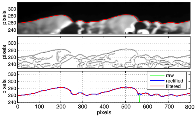
Figure 2. (a) Enlarged view of a typical image captured at 6 m fetch and 5.0 m/s wind speed in which is reported the wave profile as obtained ultimately after smoothing by a Gaussian filter ( \sigma = 5 ). (b) Contours extracted from this image by using a Canny edge detection method. (c) Wave profile as obtained immediately after a direct detection of the water surface contour (green line), after the correction of the small raw profile defects (blue bold line) and after smoothing by a Gaussian filter of standard deviation 5 (red line).
