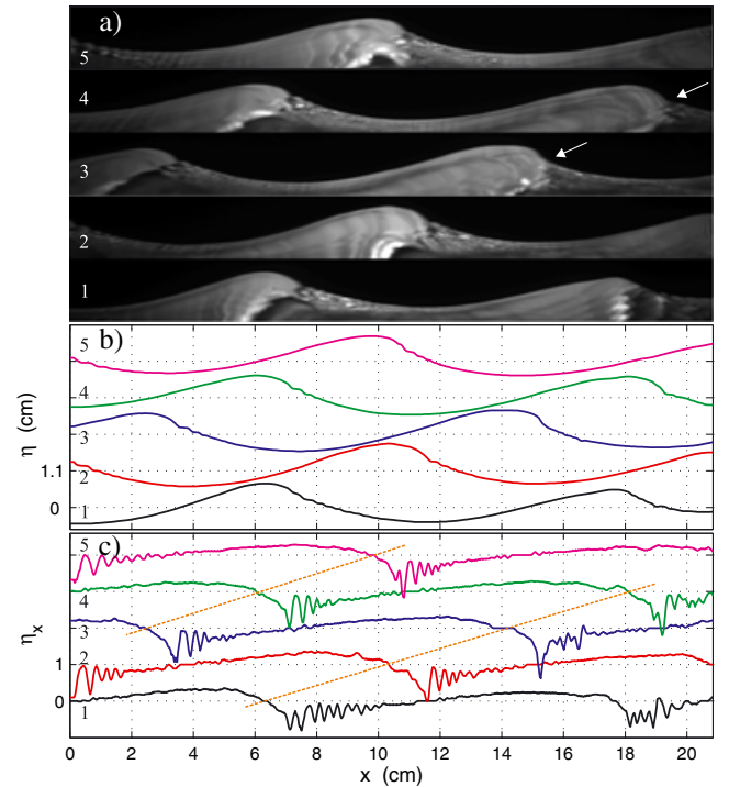
Figure 5. Longitudinal wave profiles observed at 6 m fetch and 7.0 m/s wind speed. The graph is organized as Figure 3 except that the five wave contours corresponding to the five wave contours given in Figure 5b are displayed in Figure 5a. The arrows indicate the microbreaking wave crest.
