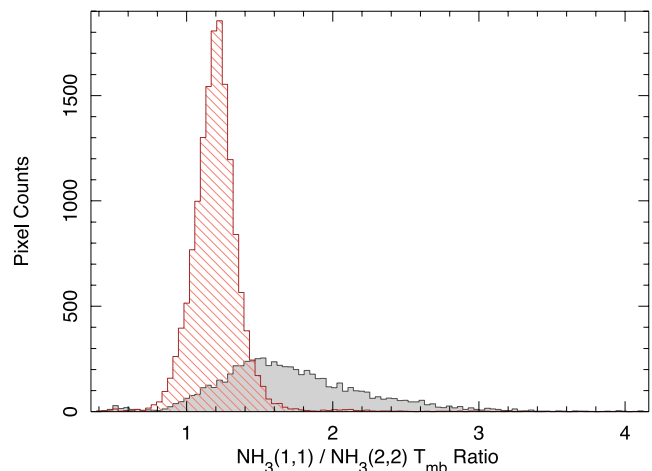
Figure 4. Plots of the brightness ratio T_{\text{mb},(1,1)}/T_{\text{mb},(2,2)} for every emitting voxel ( l - b - v data element) with T_{\text{mb}} > 3\sigma in both HOPS \text{NH}_3 data sets. The hatched histogram includes only voxels from the CMZ ( |l| < 2^\circ ) while the solid histogram includes the remaining emission from the outer Galaxy.
