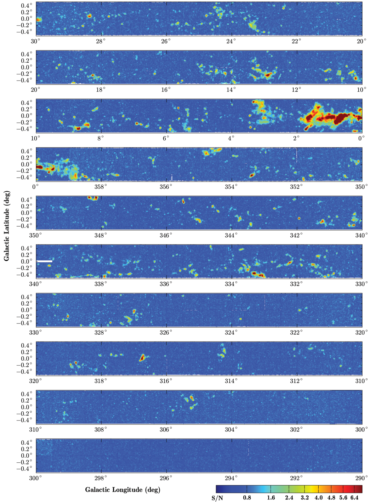
Figure 1. Map of the peak \text{NH}_3(1,1) signal-to-noise ( S/N ) across the HOPS survey area. The map was made by smoothing the S/N cube spatially (final beam \text{FWHM} = 2.5 arcmin) and in velocity (hanning window = 5) and measuring the peak brightness in each spectrum. An approximate brightness temperature scale may be found by multiplying by the average root-mean-squared (RMS) noise temperature ( \sigma_{\text{rms}} = 0.20 K).
