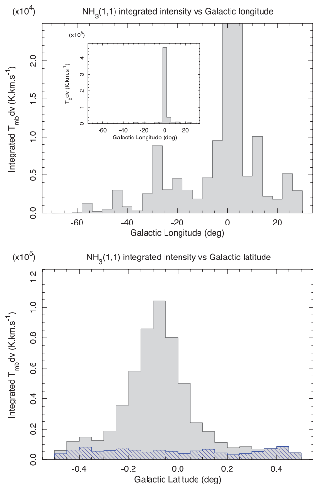
Figure 3. The top panel shows the sum of the \text{NH}_3(1,1) integrated intensity over the survey region as a function of Galactic longitude in 4^\circ bins. The longitude bin covering the central molecular zone (CMZ, -2^\circ < l < 2^\circ ) peaks at \int T_{\text{mb}} dv = 4.65 \times 10^5 \text{ K km s}^{-1} and the y axis scale has been truncated so as to show the remainder of the emission. The inset shows how the plot appears scaled to the full \int T_{\text{mb}} dv range. In the bottom panel is a similar plot of \int T_{\text{mb}} dv versus Galactic latitude. The filled grey histogram includes all emission, while the hatched histogram only includes emission outside the CMZ.
