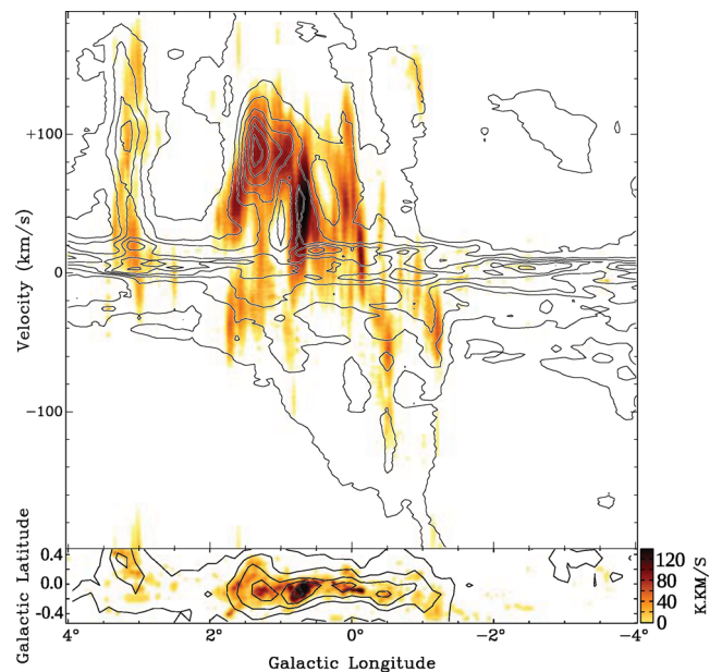
Figure 5. Details of the longitude–velocity diagram showing the Galactic Centre region (top). \text{NH}_3(1,1) emission is shown in colour scale and the Dame et al. (2001) \text{CO}(1-0) contours are overplotted. While the overall emission morphology of both molecules is similar, the brightest peaks are offset in l and v . The emission seen at v < -170 \text{ km s}^{-1} is due to a broad linewidth \text{NH}_3(2,2) emission encroaching on the \text{NH}_3(1,1) passband. The bottom panel shows the \text{NH}_3(1,1) integrated intensity map for the same l range.
