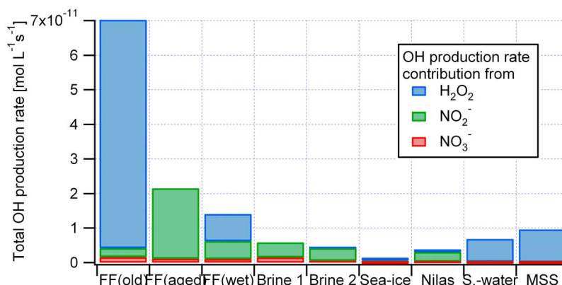
Figure 7. Mean calculated OH production rates by known chromophores, shown as stacked bars for H 2 O 2 (blue), NO 3 - (red), and NO 2 - (green). FF = frost flowers, MSS = marine surface snows, i.e., snow-pack on top of sea-ice. Data on individual samples, including collection dates, are listed in Table S1.
