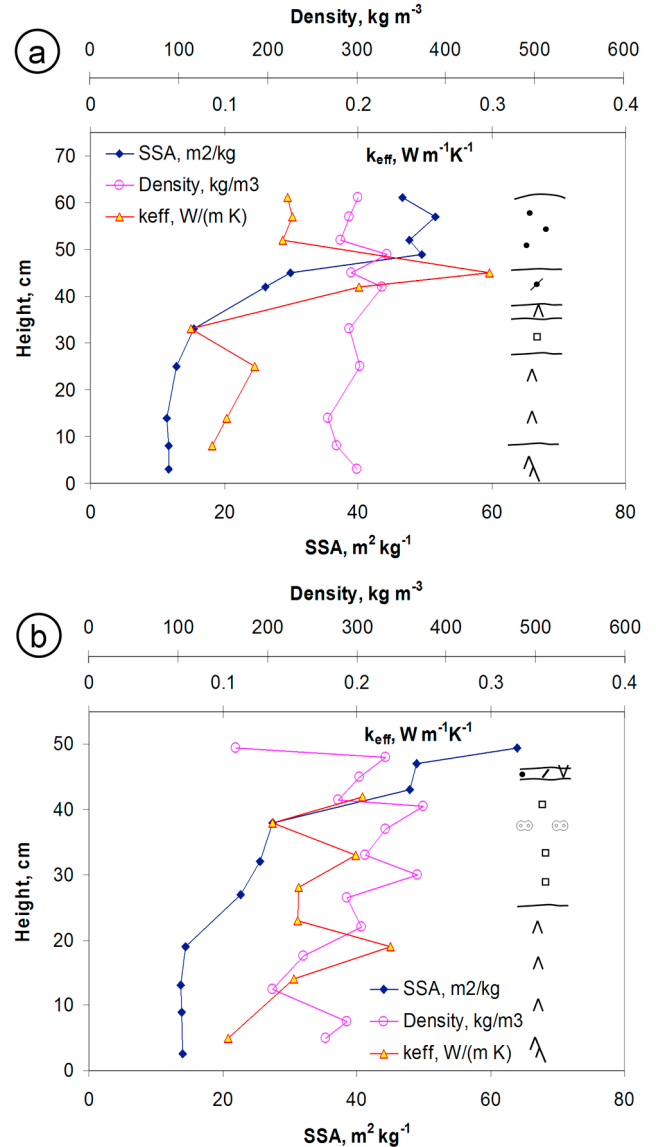
Figure 4. Profiles of specific surface area (SSA), density and thermal conductivity ( k_{\text{eff}} ) for snow on tundra. The stratigraphy is indicated on the side of the graphs, with the symbols of Figure 1. (a) On 27 March 2009 8 km South of Barrow, at 71^{\circ}18.059'N , 156^{\circ}46.042'W and (b) on 25 March 2009 near the trench of Figure 1. The top layer on Figure 4b is a mixture of decomposing particles, small rounded grains and surface hoar.
