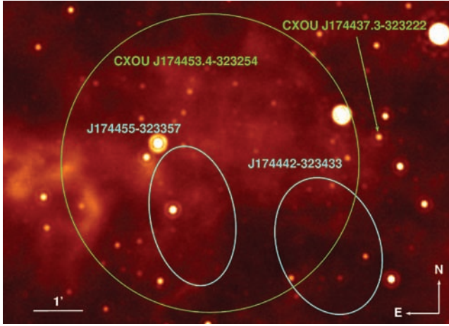
Figure 1. 24 \mu m MIPS GAL image of the field of IGR J17448–3232 showing the blazar candidate, CXOU J174437.3–323222, as well as the extent of the \sim 3 arcmin extended X-ray emission from the SNR and the extended MGPS-2 radio sources.
