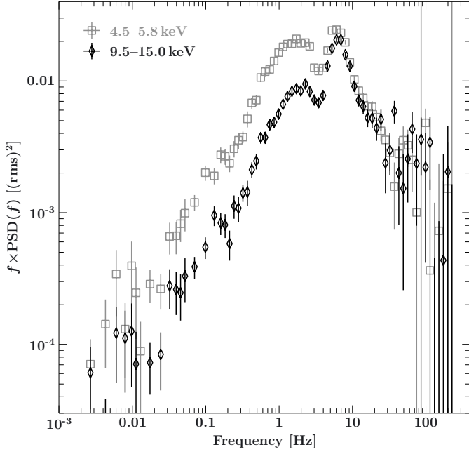
Fig. 9. PSDs of the observation 90127-01-01-05 in the low (open squares) and high (black diamonds) energy band. The photon index of this observation is \Gamma_1 = 2.33_{-0.01}^{+0.02} .
