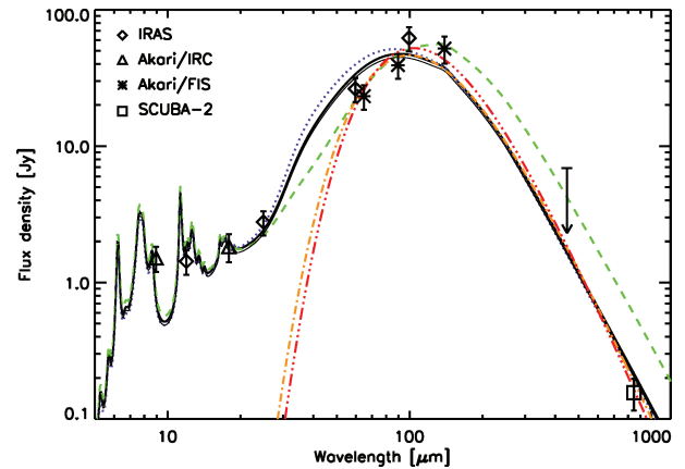
Figure 12. The observed FIR and submm SED of NGC 2559, together with dust model fits. An arrow marks the 3\sigma upper limit at 450 \mu\text{m} . The solid (black) line shows the best fit to all available data points. The dotted (blue) line is the best fit to the data set excluding the AKARI/FIS data. The thin solid (black) line is the best fit to the data set excluding the IRAS data. The dashed (green) line is the best-fitting model without the SCUBA-2 points. The dot-dashed (orange) line is the modified blackbody fit with \beta = 2 . The triple-dot-dashed (red) line is the modified blackbody fit with free \beta . Error bars include an uncorrelated 20 per cent uncertainty.
