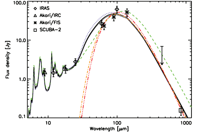
Figure 12. The observed FIR and submm SED of NGC 2559, together with dust model fits. An arrow marks the 3\sigma upper limit at 450 \mu m. The solid (black) line shows the best fit to all available data points. The dotted (blue) line is the best fit to the data set excluding the AKARI/FIS data. The thin solid (black) line is the best fit to the data set excluding the IRAS data. The dashed (green) line is the best-fitting model without the SCUBA-2 points. The dot-dashed (orange) line is the modified blackbody fit with \beta = 2 . The triple-dot-dashed (red) line is the modified blackbody fit with free \beta . Error bars include an uncorrelated 20 per cent uncertainty.
