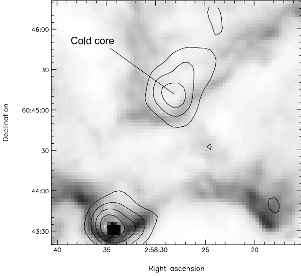
Figure 11. SCUBA-2 contours overlaid on Spitzer 24- \mu m image. The source labelled ‘cold core’ is circled and shows up clearly in the submm, yet within a dark region of the Spitzer image. It is, however, detected at 70 and 160 \mu m with Spitzer .
