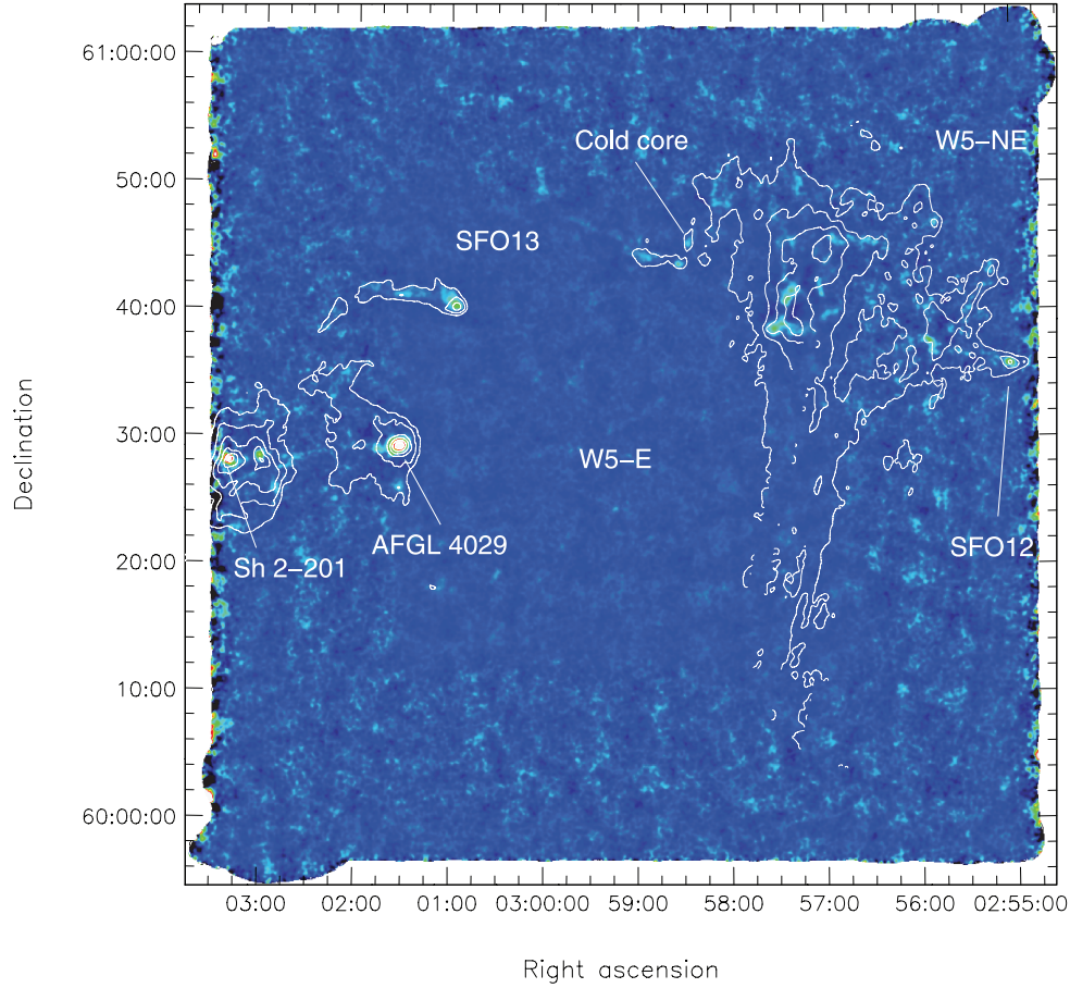
Figure 13. SCUBA-2 850- \mu m emission in colour with Spitzer 70- \mu m contours overlaid. Sources are labelled as in Fig. 4. The Spitzer contours do not close to the south of W5-NE due to a lack of coverage there.
