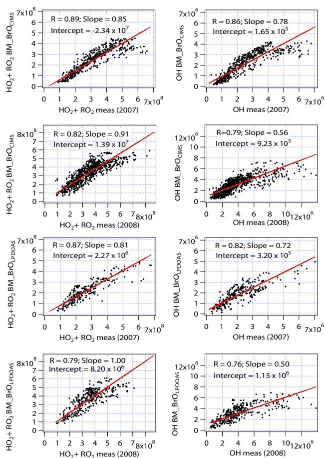
Fig. 6. \text{HO}_2 + \text{RO}_2 and OH predictions from the base model incorporating bromine chemistry constrained by BrO measurements by CIMS (BM.BrO CIMS ) and LPDOAS (BM.BrO LPDOAS ) plotted versus the observations in 2007 and 2008. The data are averaged on a 10 min time base. The correlation coefficient ( R ) and the slope and intercept from an equally weighted bivariate regression (red line) for each panel are also denoted in the figure. The units of OH and \text{HO}_2 + \text{RO}_2 concentrations are \text{molec cm}^{-3} .
