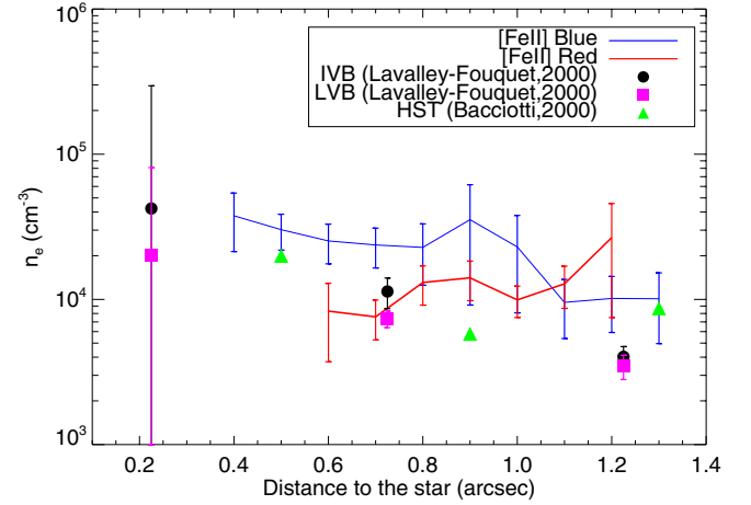
Fig. 6. Plot of n_e versus distance derived from the ratio of the [Fe II] 1.53 \text{ }\mu\text{m} to 1.64 \text{ }\mu\text{m} lines (averaged over \pm 0''.5 from the jet axis) for the blueshifted (blue points, top curve) and redshifted (red points, bottom curve) lobe. Also shown are previous determinations from the [S II] doublet ratio over similar velocity ranges: IVB and LVB from Lavalley-Fouquet et al. (2000) (black circle, purple square), MVB interval of Bacciotti et al. (2000) (green triangles).
