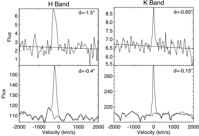
Fig. 1. Illustration of the continuum subtraction methods, close to the star ( bottom row ) and far from the star ( top row ), for the [Fe II] 1.64 \mu\text{m} ( left panels ) and the H 2 2.12 \mu\text{m} line ( right panels ). The raw spectra are plotted in thick lines and the fitted continua in thin lines. See text for details. The analysis and discussion of H 2 2.12 \mu\text{m} lines will be presented in a separate paper.
