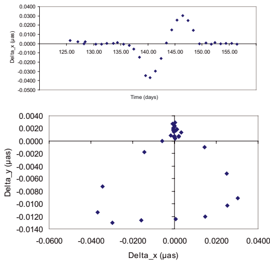
Fig. 2. Astrometric shift (deltax) as a function of time ( top ) and excursions of the photocenter during a low-activity period (JD 2450335 to JD 2450365).
