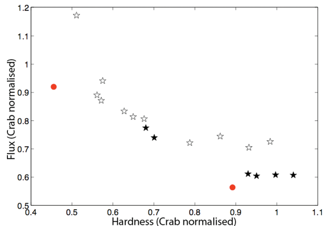
Figure 1. HID comparing our observations (filled circles) to the plateau states from Belloni et al. (2000) (data courtesy of T. Belloni; open stars are \chi_1 , closed stars are \chi_3 ). The soft, higher-luminosity red dot is ObsID 90105-07-02-00, the lower is ObsID 40403-01-09-00. The plot shows the hardness and flux, normalized to Crab units, calculated by taking the ratio and the sum of the RXTE PCU 2 rates in two bands: channel 0–35 ( \sim 2 – 15 keV) and 36–49 ( \sim 16 – 21 keV). Each band is divided by the Crab rate in the same band, on the same day, simulating a photon index of 2.1 and utilizing a normalization of 10 \text{ photons cm}^{-2} \text{ s}^{-1} \text{ keV}^{-1} at 1 keV.
