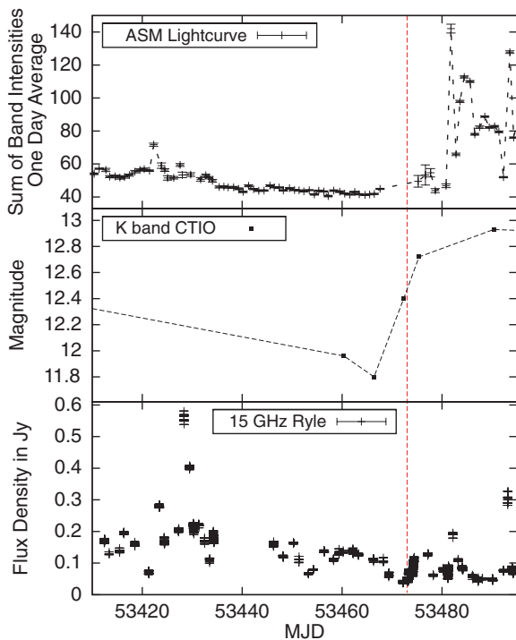
Figure 3. GRS 1915+105 X-ray and radio light curves for the 2005 data set. The radio light curve was measured by the Ryle Telescope (Pooley & Fender 1997). The red dashed line indicates the time of the RXTE observation.
