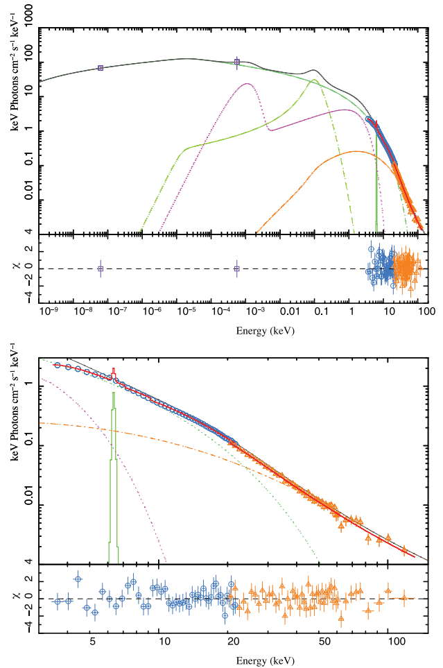
Figure 11. Multiwavelength (top) and X-ray band only (bottom) bestfitting result ( \chi_{\text{red}}^2 \sim 1.15 ) spectrum, for the 2005 data set, using the synchrotron cut-off to fit the X-ray (cf. Table 3, SYNCH column).
