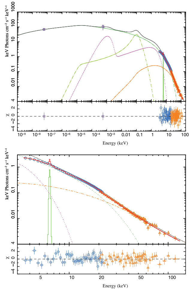
Figure 11. Multiwavelength (top) and X-ray band only (bottom) bestfitting result ( \chi^2_{\text{red}} \sim 1.15 ) spectrum, for the 2005 data set, using the synchrotron cut-off to fit the X-ray (cf. Table 3, SYNCH column).
