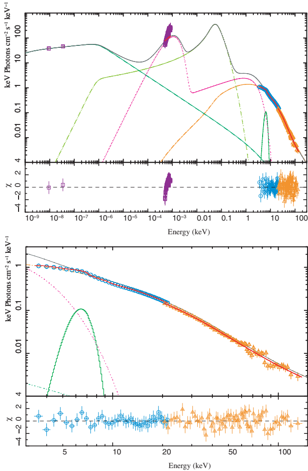
Figure 6. Multiwavelength (top) and X-ray band only (bottom) best-fitting ( \chi^2_{\text{red}} \sim 1.16 ) model spectrum (cf. Table 3, SMEDGE column), using MNW05+Gaussian+smedge. Individual contributions from the MNW05 model are also shown: The light-green dashed curve is the pre-shock synchrotron contribution. The dark-green dash-dotted curve is the post-shock synchrotron. The purple dotted curve represents the thermal contributions from the stellar blackbody (below \sim 10^{-2} keV) and the accretion disc. The orange dashed-dotted line above \sim 10^{-3} keV represent the Compton-upscattered stellar blackbody and accretion disc seed photons and the Synchrotron Self-Comptonization (SSC) of the pre-shock synchrotron. The solid grey line is the total MNW05 model spectrum originating from the jet, the accretion disc and the companion; however, it is not forward-folded through the detector response matrices and without iron line or reflection contributions or absorption due to the interstellar hydrogen column density or the smedge model. The red solid lines through the data points show the model flux including all these features. The iron line complex, modelled by a Gaussian, is shown by the thick green curve near 6.4 keV.
