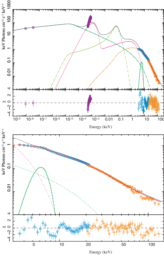
Figure 8. Multiwavelength (top) and X-ray band only (bottom) best-fitting ( \chi^2_{\text{red}} \sim 1.44 ) model spectrum (cf. Table 3, SMEDGE2 column), also employing MNW05+Gaussian+smedge, but with a reduced magnetic dominance ( k \sim 30 in stead of \sim 550 , see Table 3).
