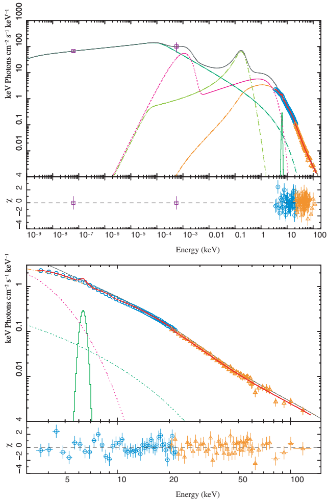
Figure 10. Multiwavelength (top) and X-ray band only (bottom) bestfitting result ( \chi_{\text{red}}^2 \sim 1.0 ) spectrum, for the 2005 data set, using a reduced low electron temperature T_e \sim 4 \times 10^9 K (cf. Table 3, ELTEMP column).
