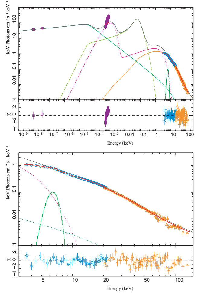
Figure 9. Multiwavelength (top) and X-ray band only (bottom) best-fitting result ( \chi^2_{\text{red}} \sim 1.01 ) spectrum (cf. Table 3, 6KPC column), for the 1999 data set, using MNW05+Gaussian+smedge and employing a fixed distance of 6 kpc.
