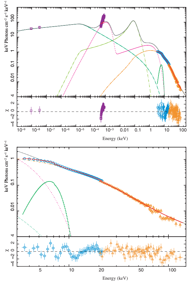
Figure 7. Multiwavelength (top) and X-ray band only (bottom) best-fitting ( \chi^2_{\text{red}} \sim 1.48 ) model spectrum (cf. Table 3, REFLECT column), using MNW05+Gaussian+reflect.
