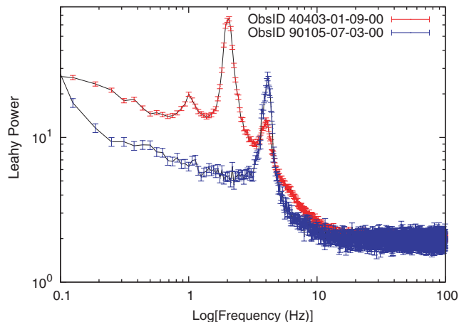
Figure 4. Normalized (following Leahy et al. 1983) power density spectra showing the type-C QPOs in the X-rays for both data sets, indicating the observations are plateau state. (Courtesy of P. Soleri).
