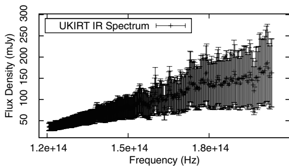
Figure 5. NIR spectrum of the 1999 data set.
