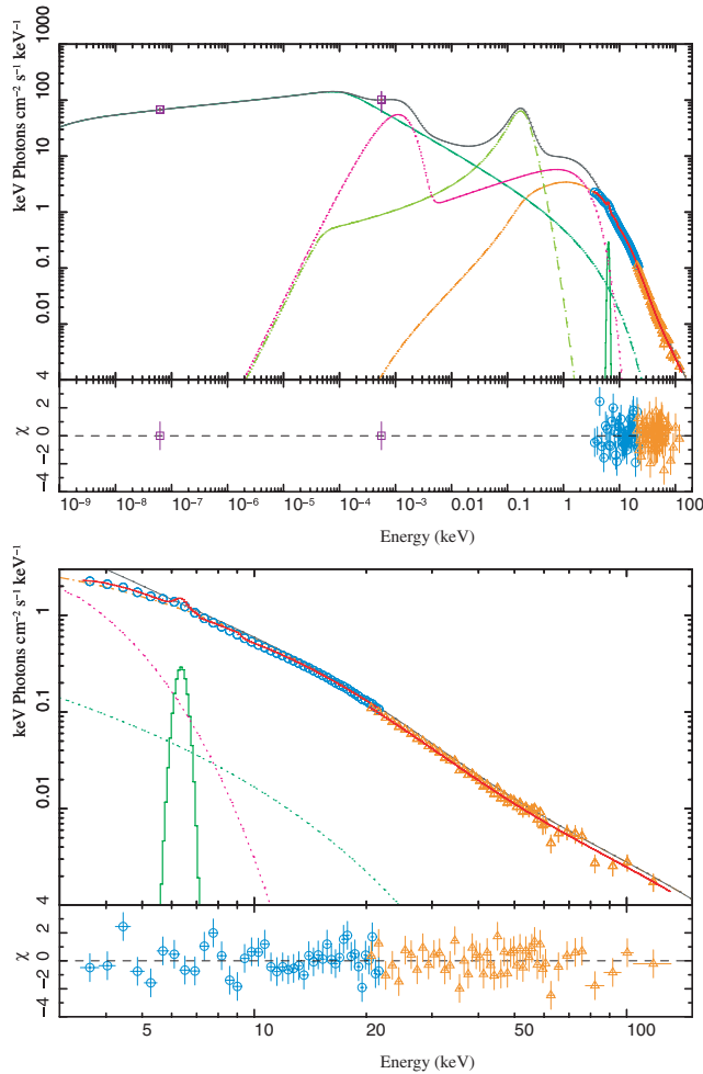
Figure 10. Multiwavelength (top) and X-ray band only (bottom) bestfitting result ( \chi^2_{\text{red}} \sim 1.0 ) spectrum, for the 2005 data set, using a reduced low electron temperature T_e \sim 4 \times 10^9 K (cf. Table 3, ELTEMP column).
