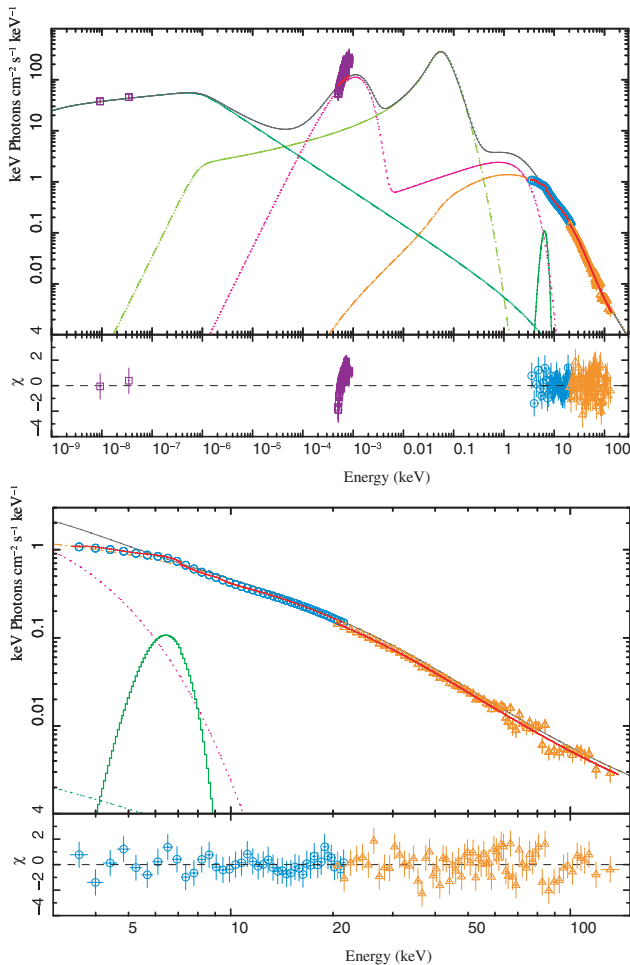
Figure 6. Multiwavelength (top) and X-ray band only (bottom) best-fitting ( \chi^2_{\text{red}} \sim 1.16 ) model spectrum (cf. Table 3, SMEDGE column), using MNW05+Gaussian+smedge. Individual contributions from the MNW05 model are also shown: The light-green dashed curve is the pre-shock synchrotron contribution. The dark-green dash-dotted curve is the post-shock synchrotron. The purple dotted curve represents the thermal contributions from the stellar blackbody (below \sim 10^{-2} keV) and the accretion disc. The orange dashed-dotted line above \sim 10^{-3} keV represent the Compton-upscattered stellar blackbody and accretion disc seed photons and the Synchrotron Self-Comptonization (SSC) of the pre-shock synchrotron. The solid grey line is the total MNW05 model spectrum originating from the jet, the accretion disc and the companion; however, it is not forward-folded through the detector response matrices and without iron line or reflection contributions or absorption due to the interstellar hydrogen column density or the smedge model. The red solid lines through the data points show the model flux including all these features. The iron line complex, modelled by a Gaussian, is shown by the thick green curve near 6.4 keV.
