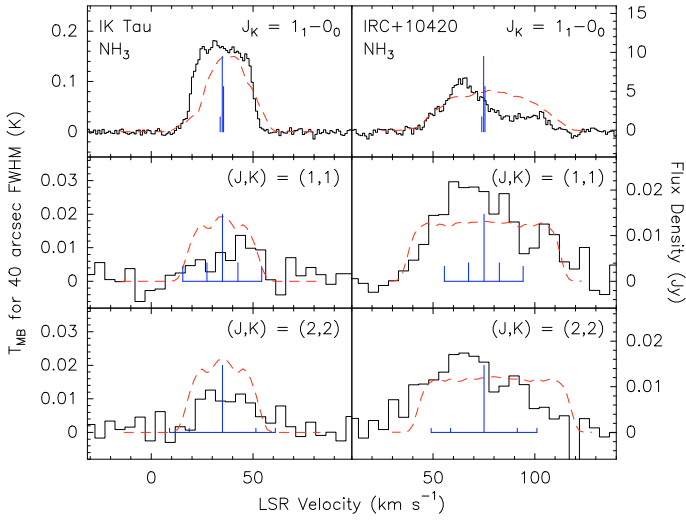
Fig. A.1. Spectra of NH 3 transitions for IK Tau ( left column ) and IRC+10420 ( right column ). Top row : HIFI spectra of the J_K = 1_0-0_0 ortho-NH 3 line. Middle row : VLA spectra of the (J, K) = (1, 1) para-NH 3 line. Bottom row : VLA spectra of the (J, K) = (2, 2) para-NH 3 line. The intensity scales apply for both sources. The lefthand ordinate gives main-beam brightness temperature in a 40'' FWHM beam, while the righthand ordinate gives flux density in Jy units. In all panels the red dashed line represents our best-fit model prediction. The blue bars give the spacings and theoretical relative intensities of the main groups of hfs components determined by Cazzoli et al. (2009) for the 1_0-0_0 transition and by Kukolich (1967) for the (1, 1) and (2, 2) inversion lines, respectively.
