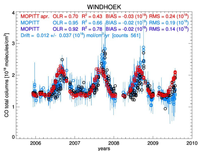
Figure 3. Time series of CO total columns at Windhoek, Namibia, for MOZAIC/IAGOS (black) as well as the MOPITT measurements (blue) and the MOPITT a priori (red). The MOPITT measurements show the mean (circle) and the range of MOPITT measurements (line) that coincide with a single MOZAIC/IAGOS measurement. The statistics represent the Ordinary Linear Regression (OLR) coefficient, the explained variance (square of correlation coefficient: R^2 ), the bias and the root-mean-square (RMS) differences. For the dark blue statistics (so-called “range”), we assume that if the MOZAIC/IAGOS column falls within the range of MOPITT total column measurements along the MOZAIC/IAGOS flight path, the MOPITT column equals the MOZAIC/IAGOS column. The drift statistics are calculated for the basic MOZAIC/IAGOS–MOPITT comparison without consideration of the MOPITT range along the MOZAIC/IAGOS flight path.
