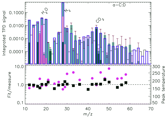
Fig. 2. Same as Fig. 1 for an irradiated a-C:D film with the expected mass separation peak pattern every two m/z due to the deuterium substitution. The data peaks at uneven m/z are due to eventual pollution and hydrogen contamination in the film.
