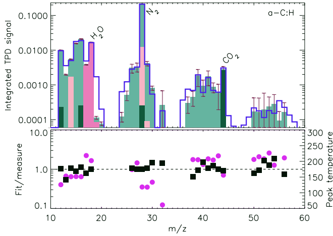
Fig. 1. Top: QMS integrated signal recorded during the TPD of an irradiated a-C:H film (blue histogram). The synthetic mass spectrum obtained by a matrix analysis is shown with filled bar graphs; the associated error bars come from the minimization procedure. Bottom: ratio of the fitted versus measured individual mass spectra for the main peaks (left axis, squares), and peak temperature associated with the TPD for the considered mass (right axis, circles).
