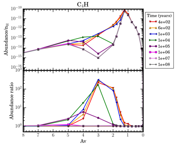
Fig. B.3. Same as Fig. B.1 with a low sulfur abundance in the initial conditions for C_4H : abundance of C_4H (top) and abundance ratio of C_4H with the addition of photolytic reactions divided by the abundances without the addition of photolytic reactions (bottom) for different times.
