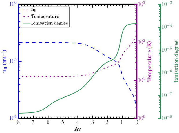
Fig. A.1. Temperature (purple dotted line), total hydrogen density (blue dashed line), and ionization degree (green solid line) as a function of visual extinction.
