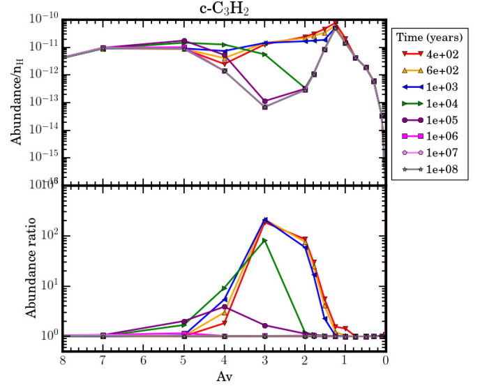
Fig. B.2. Same as Fig. B.1 with a low sulfur abundance in the initial conditions for C_3H_2 : abundance of C_3H_2 (top) and abundance ratio of C_3H_2 with the addition of photolytic reactions divided by the abundances without the addition of photolytic reactions (bottom) for different times.
