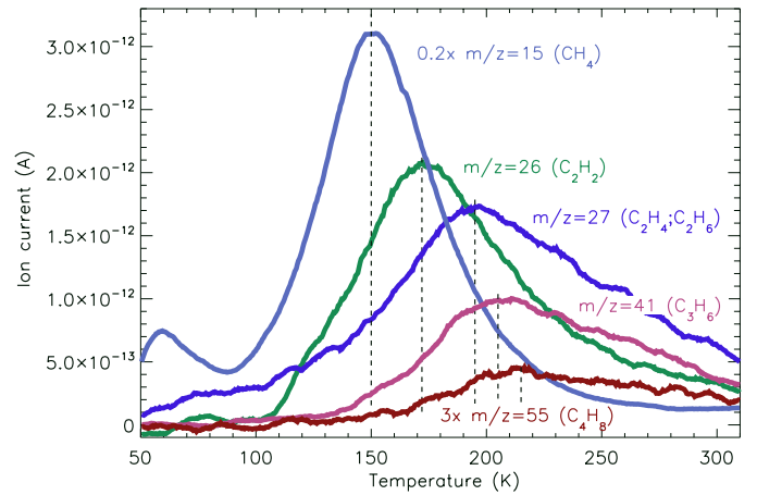
Fig. 3. TPD spectra recorded for selected m/z for the a-C:H experiment. The chosen masses are dominated by a small amount of fragments contributing to the signal. The corresponding parent species are given in brackets, as obtained from the minimization. The desorption temperature peaks are indicated by vertical dashed lines.
