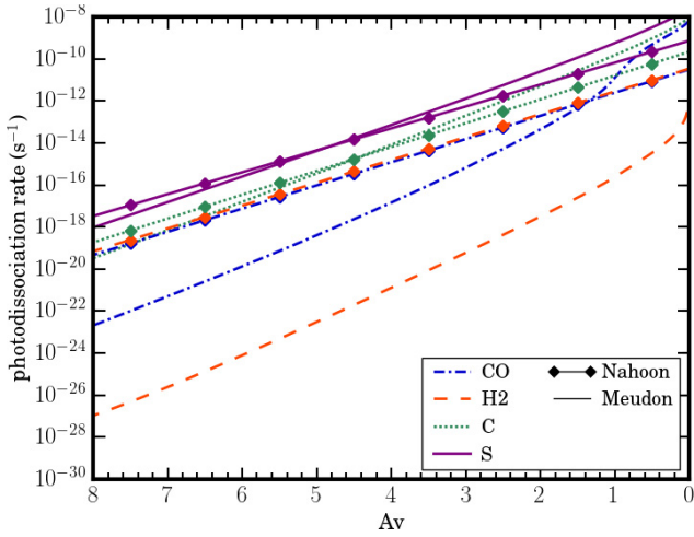
Fig. A.2. Photodissociation rates of CO (blue dashed dotted lines) and H 2 (red dashed lines) and photoionization rates of C (green dotted lines) and S (purple solid lines) as a function of the visual extinction in the Meudon code (no symbols) and in Nahoo (diamond lines).
