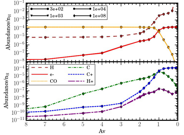
Fig. A.3. Abundance of H (brown long dashed line), electrons (red solid line), CO (yellow dotted lines), C (green dash-dotted line), C + (blue short dotted line), and H + (purple short and long dashed line) for times of 300 yr (circle), 1000 yr (triangle), 10 4 yr (pentagon), and 10 8 yr (diamond) as a function of the visual extinction.
