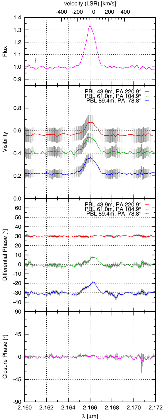
Fig. 4. AMBER observation of HD 98922 at spectral resolution of R = 12\,000 (28 Feb. 2013). From top to bottom: wavelength dependence of flux, visibilities, wavelength-differential phases, and closure phase observed at three different projected baselines (see labels in figure). For clarity, the differential phases of the first and last baselines are shifted by +30^\circ and -30^\circ , respectively.
