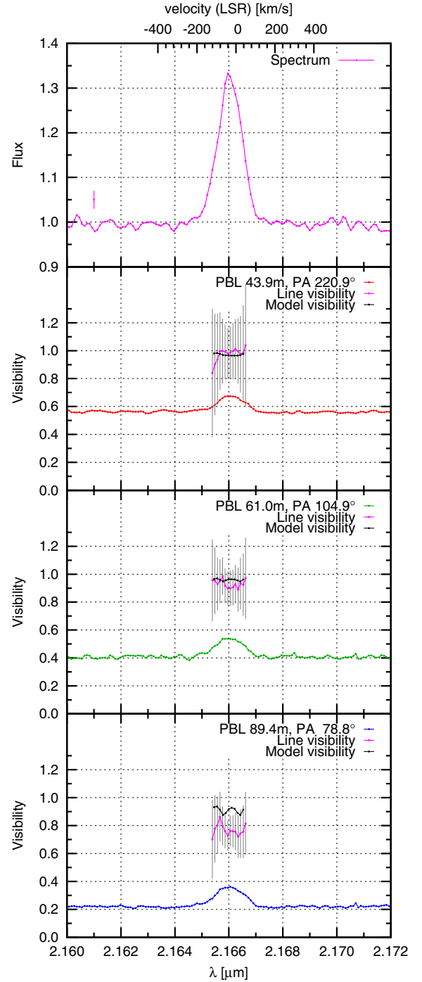
Fig. 5. Comparison of the observed (pink solid lines) and modelled (black solid lines) continuum-corrected (pure) Bry line visibilities of our AMBER observation of HD 98922. From top to bottom: wavelength dependence of flux and visibilities of the first, second, and third baseline. In each visibility panel the observed total visibilities (red, green, blue, as in Fig. 4), the observed pure Bry line visibilities (pink), and the modelled pure Bry line visibilities (black) are shown.
