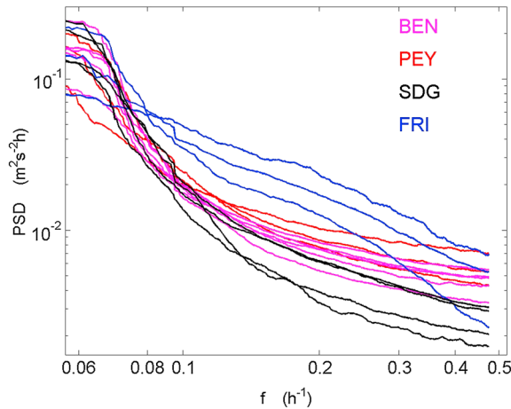
Figure 5. Smoothed averaged experimental spectra. Averaging is performed for each sequence of the set of valid radar cells. Smoothing is done on averaged spectra. The number of summation is the value of n_{tot} in Table 2.
