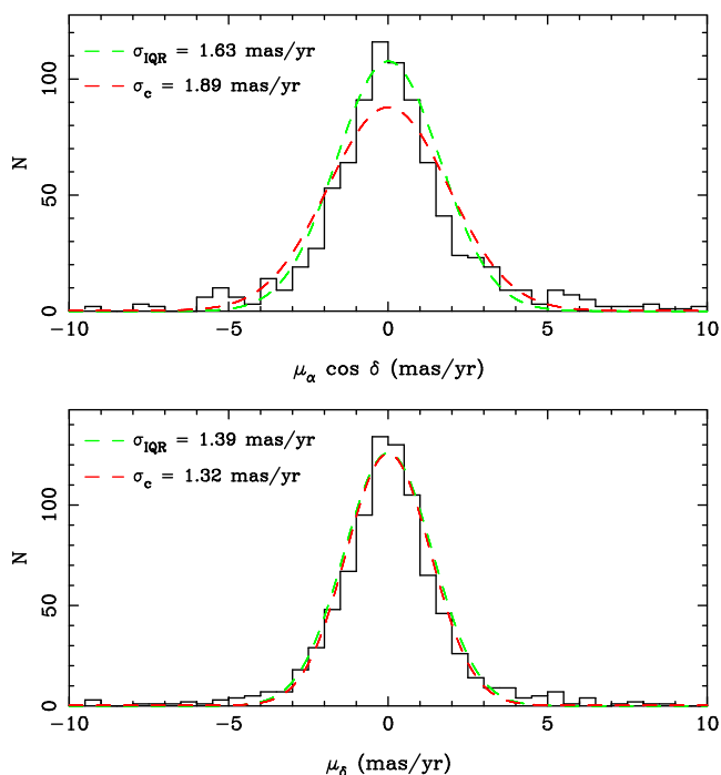
Figure 6. PM velocity distributions along both axes (black histogram) showing the interquartile range velocity dispersions (green dashed lines) and the two-component Gaussian mixture model for the velocity dispersion (red dashed lines). The best-fitting velocity dispersions are listed in each case, which for the Gaussian mixture model is the dominant Cyg OB2 component.
