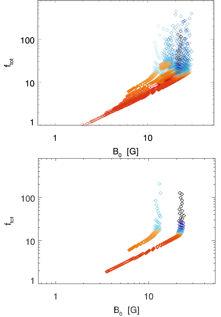
Fig. 7. Scatter-plots of the total flux-tube expansion rate as a function of the magnetic field strength at the surface. The top panel represents these quantities calculated from our simulations for an 11 yr period. The points are colour-coded according to the speed attained by the wind flow in each flux-tube (orange represents fast wind, blue represents slow wind). The bottom panel represents only the simulation data points relative to the minimum and to the maximum (first and third panels in Fig. 5).
