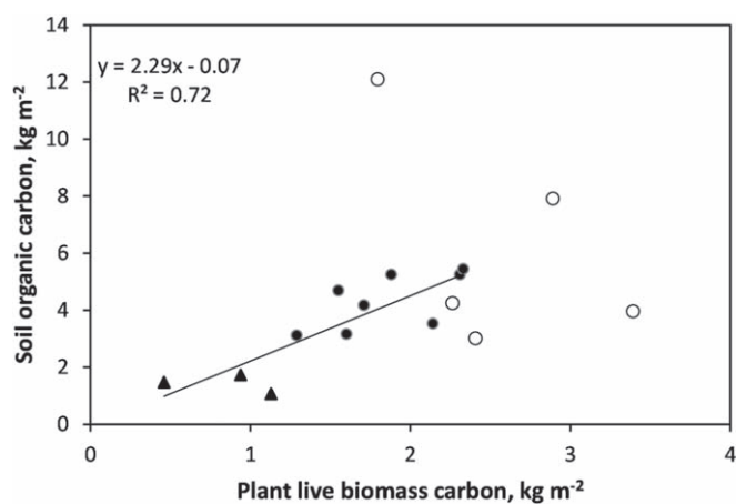
Figure 5. Relationship between soil organic carbon (SOC) content and plant live biomass carbon stock. Closed symbols represent plots sampled in the lichen tundra and in the medium shrub tundra vegetation type. Triangles are for lichen tundra and circles for medium shrub tundra. Open symbols represent plots sampled in the tall shrub tundra type. The regression line is based on data from the lichen tundra and medium shrub tundra plots. As the regression including also the tall shrub tundra was not significant, it is not shown here. Its equation is y = 1.49 x + 1.58 , R^2 = 0.17 .
