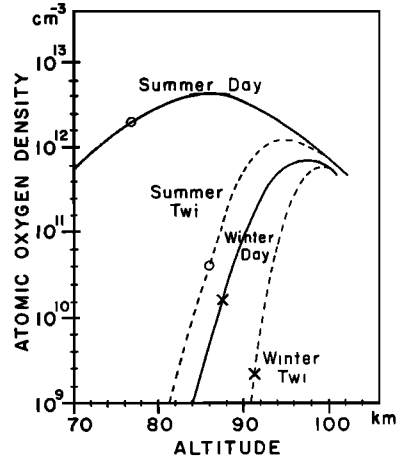
Fig. 24. Atomic oxygen densities required to produce seasonal and diurnal variation in free sodium on the basis of photochemistry alone.
