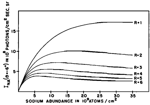
Fig. 15. Twilight glow intensity at 6° solar depression as a function of the twilight abundance for various ratios of day to twilight abundance.
