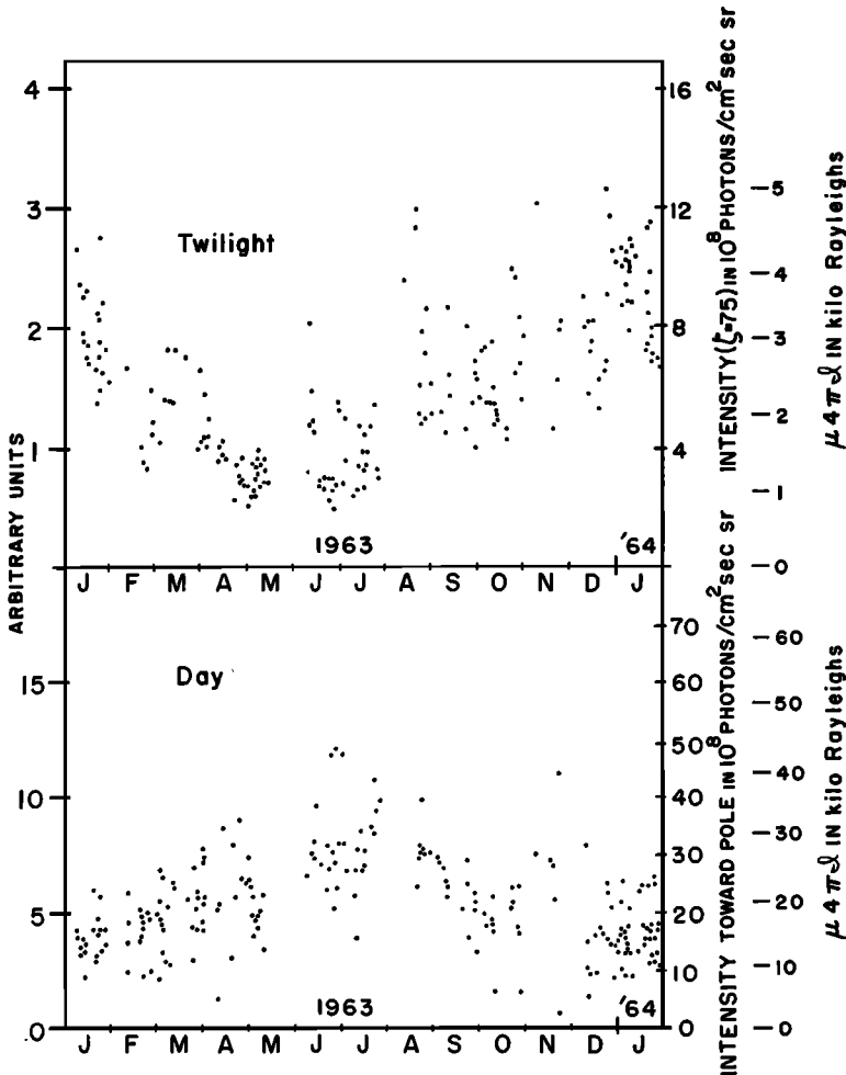
Fig. 12c. Sodium twilight-glow and dayglow intensities 1963, Haute Provence. Emission rate scale in kilorayleighs applies to zenith. Dayglow data are for a solar elevation angle of 30° except for November, December, and January, when they are for 20°.
