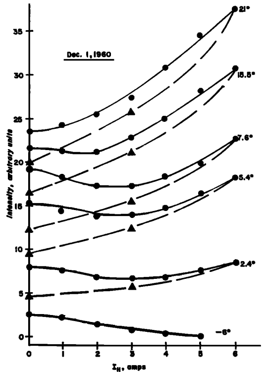
Fig. 10. Magnetic scans of Zeeman photometer from 0 to 4000 oersteds for various angles of solar elevation, December 1, 1960. Fraunhofer-line components in sky light fitted at 4000 oersteds are dashed lines.
