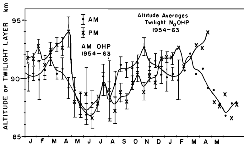
Fig. 20. Average altitude of twilight layer at Haute Provence 1954-1963, morning and evening. Standard deviations are indicated.
