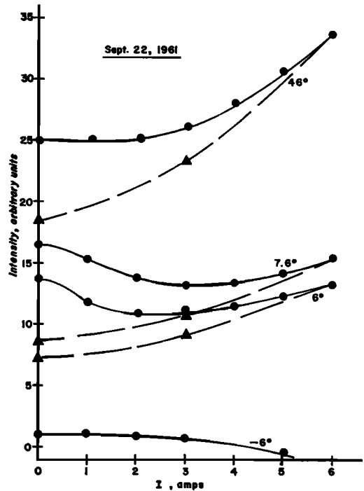
Fig. 9. Magnetic scans of Zeeman photometer from 0 to 4000 oersteds for various angles of solar elevation, September 22, 1961. Fraunhofer-line components in sky light fitted at 4000 oersteds are dashed lines.
