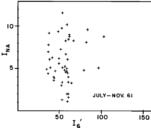
Fig. 4. Sodium dayglow signal plotted against total photometer response at 4000 oersteds July-November 1961, Haute Provence.
