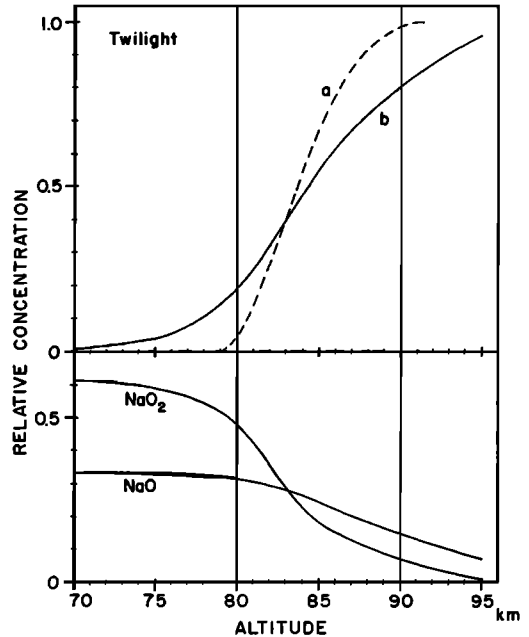
Fig. 27. Relative distribution of sodium with altitude in the absence of a gravitational field with total concentration of all forms of sodium independent of altitude. Curve a , chemical equilibrium; b , diffusion included.
