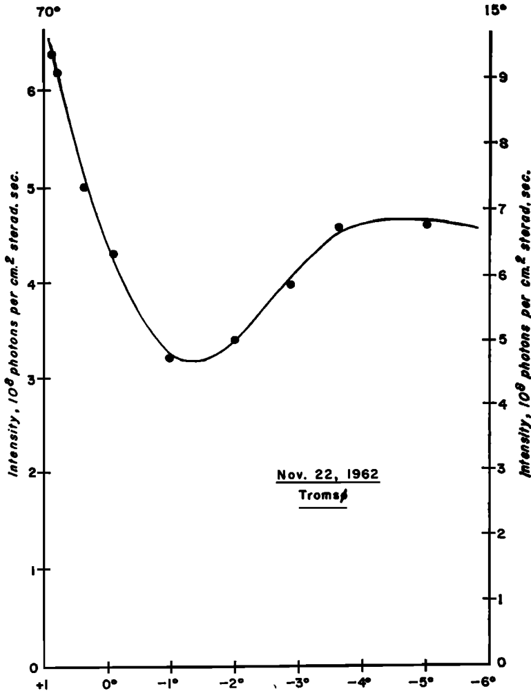
Fig. 3. Sodium twilight glow, November 22, 1962, Tromsø, Norway.
