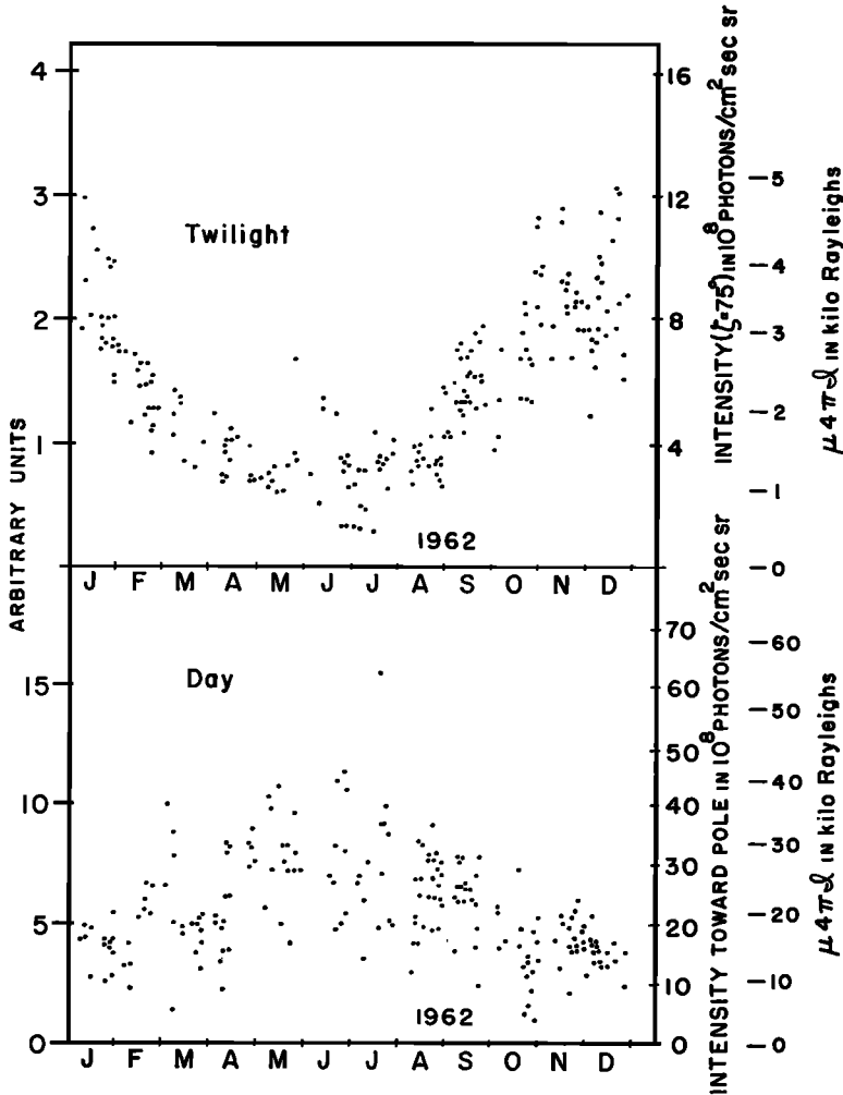
Fig. 12b. Sodium twilight-glow and dayglow intensities 1962, Haute Provence. Emission rate scale in kilorayleighs applies to zenith. Dayglow data are for a solar elevation angle of 30^\circ except for November, December, and January, when they are for 20^\circ .
