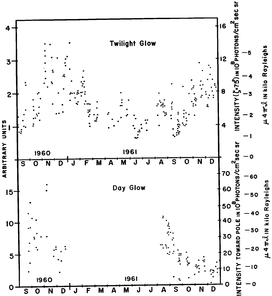
Fig. 12a. Sodium twilight-glow and dayglow intensities 1960, 1961, Haute Provence. Emission rate scale in kilorayleighs applies to zenith. Dayglow data are for a solar elevation angle of 30^\circ except for November, December, and January, when they are for 20^\circ .
