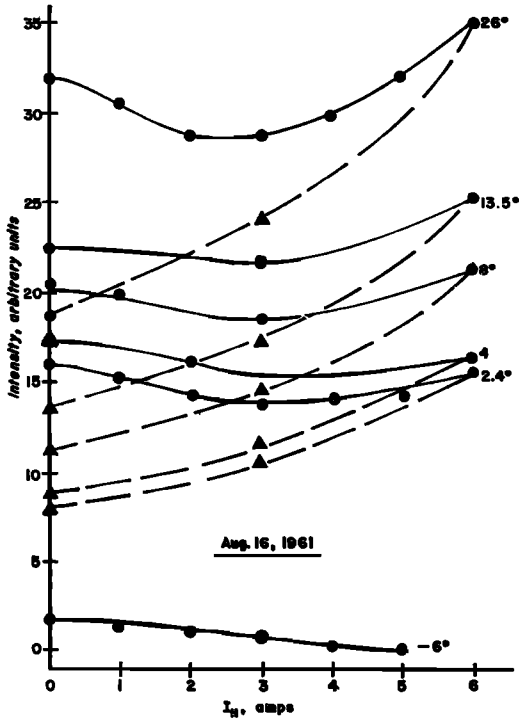
Fig. 8. Magnetic scans of Zeeman photometer from 0 to 4000 oersteds for various angles of solar elevation, August 16, 1961. Fraunhofer-line components in sky light fitted at 4000 oersteds are dashed lines.
