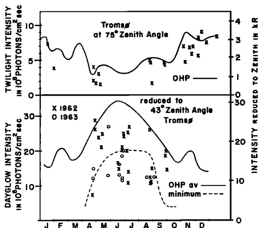
Fig. 19. Sodium twilight and dayglow intensities at Tromsø for 1962 and 1963 compared with the averages (solid lines) and minimum dayglow intensities at Haute Provence (dashed line).
