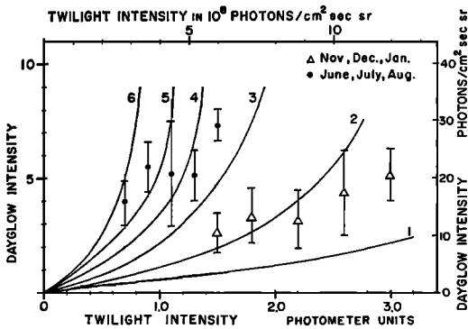
Fig. 17. The dayglow signal at 30^\circ solar elevation toward the pole plotted against the twilight signal at -6^\circ solar elevation for observation 15^\circ above the horizon. Averaged data for June, July, and August 1961–1963 are plotted. Theoretical curves to which the scales on the top and to the right apply are labeled with numbers representing the day to twilight abundance ratio.
