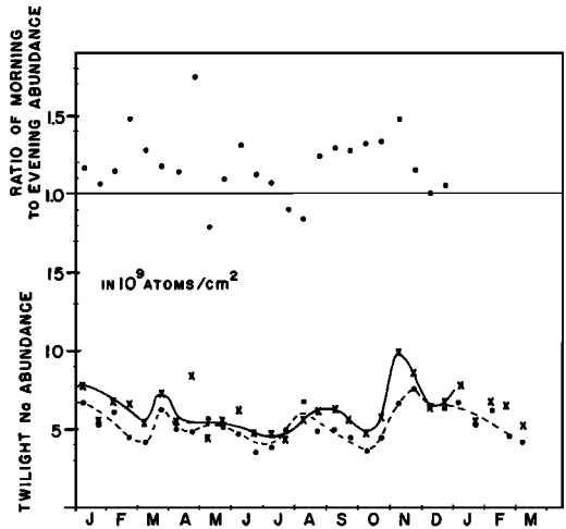
Fig. 18. Abundance of sodium in twilight at Haute Provence morning and evening. Ratio of morning to evening abundance is plotted at the top.
