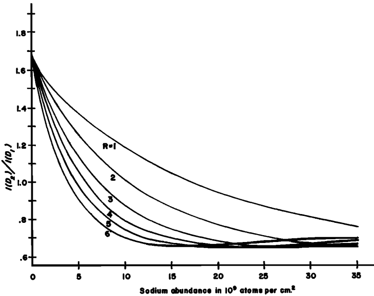
Fig. 16. The ratio of the fine structure component intensities in twilight as a function of twilight abundance for various ratios of day to twilight abundance.
