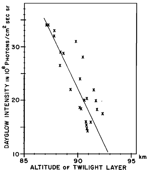
Fig. 22. Anticorrelation of dayglow intensity with altitude of twilight layer. Points are taken from semimonthly averages.
