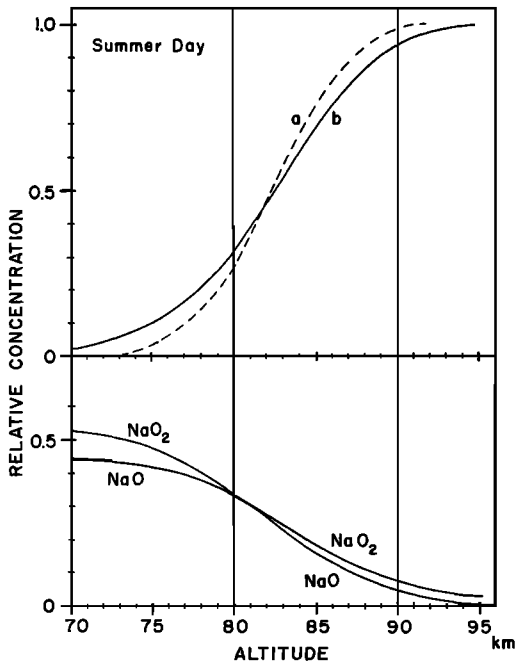
Fig. 26. Relative distribution of sodium with altitude in the absence of a gravitational field with total concentration of all forms of sodium independent of altitude. Curve a , chemical equilibrium; b , diffusion included.
