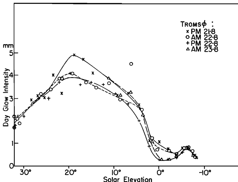
Fig. 2. Sodium day and twilight glow from noon August 21 to noon August 23, 1962, Tromsø, Norway. Units are arbitrary.
