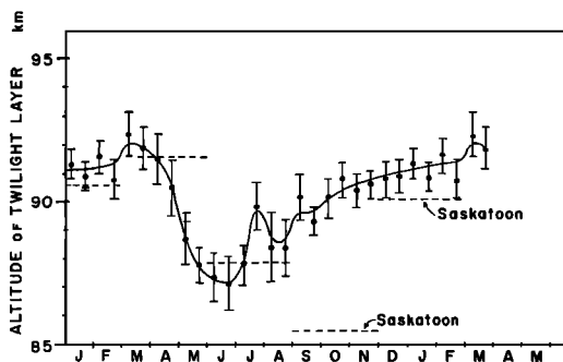
Fig. 21. Average altitude of twilight layer at Haute Provence 1954-1963, morning and evening data lumped. Results of Bullock and Hunten at Saskatoon are shown for comparison.
