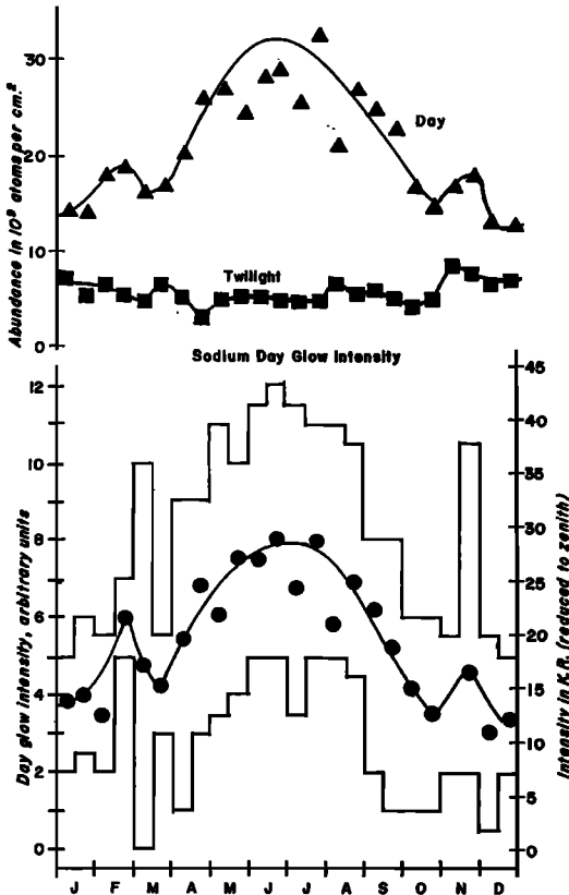
Fig. 14. Sodium dayglow intensity at Haute Provence for a solar elevation angle of 30° (20° November–February). Extreme readings are indicated as well as averages from August 1961 to January 1964. The daytime and twilight abundances are plotted at the top of the figure.
