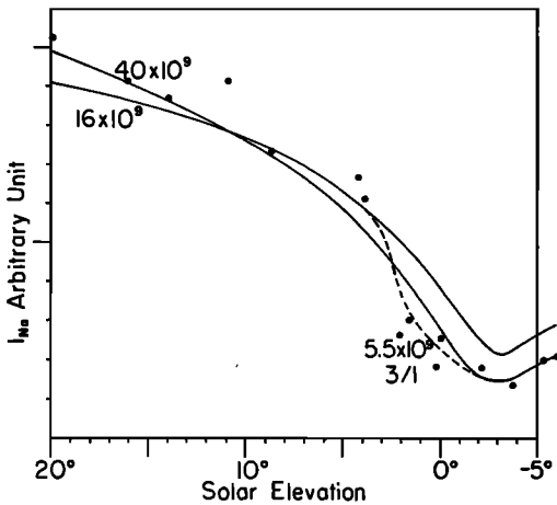
Fig. 1. Sodium day and twilight glow, May 10, 1962, Tromsø, Norway. Theoretical curves are for 40 \times 10^9 atoms/cm 2 and for 16 \times 10^9 atoms/cm 2 in the day followed by 5.5 \times 10^9 atoms/cm 2 in twilight.
