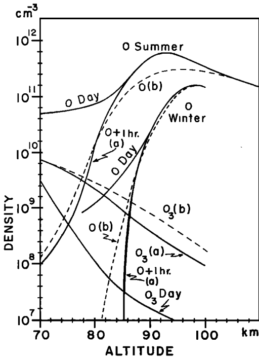
Fig. 23b. Distribution of O and O 3 with altitude. Solid curves for O 3 and O are calculated from photochemistry alone. Dashed curves show the effect of turbulent diffusion.
