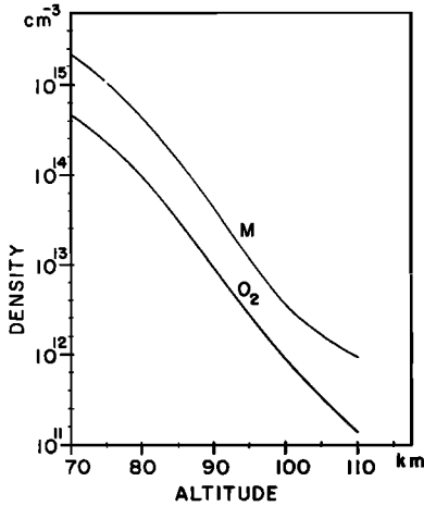
Fig. 23a. Distribution of total atmospheric constituents and O_2 with altitude.
