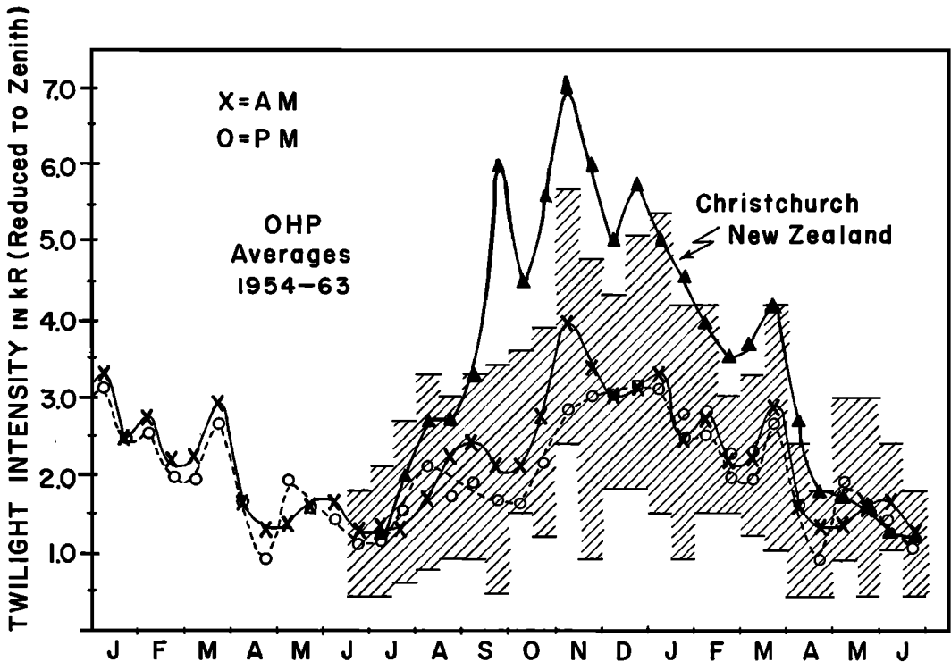
Fig. 13. Sodium twilight glow intensity at Haute Provence averaged from 1954 through 1963. Cross hatching indicates range of values observed. New Zealand data of Hunten et al. [1964] are plotted for comparison.
