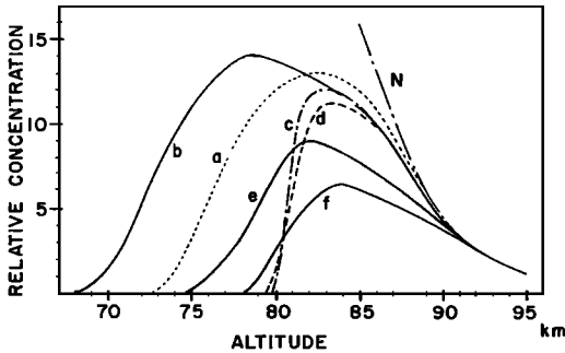
Fig. 25. Distribution of all sodium compounds in altitude ( N ) and distribution of atomic sodium. (a) Summer daytime, photochemistry alone; (b) summer daytime with turbulent diffusion accounted for; (c) summer twilight, photochemistry alone; (d) summer twilight, oxygen diffusion included; (e) summer twilight, oxygen and sodium diffusion included; (f) summer twilight, diffusion plus the ozone reaction included.
