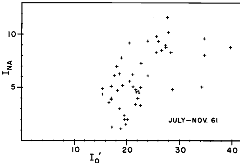
Fig. 5. Sodium dayglow signal plotted against photometer response at zero field, July-November 1961.
