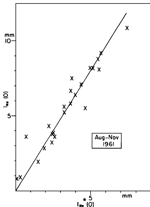
Fig. 7. Sodium dayglow signal at zero field obtained by using sky light signal at 4000 oersteds to determine the white-light signal at zero field compared with sodium dayglow signal at zero field obtained by using sky light signal at 2000 oersteds to determine the white-light component. Sky light at 2000 oersteds certainly has no water vapor contamination, but the evidence here is that it does contain a sodium emission component.
