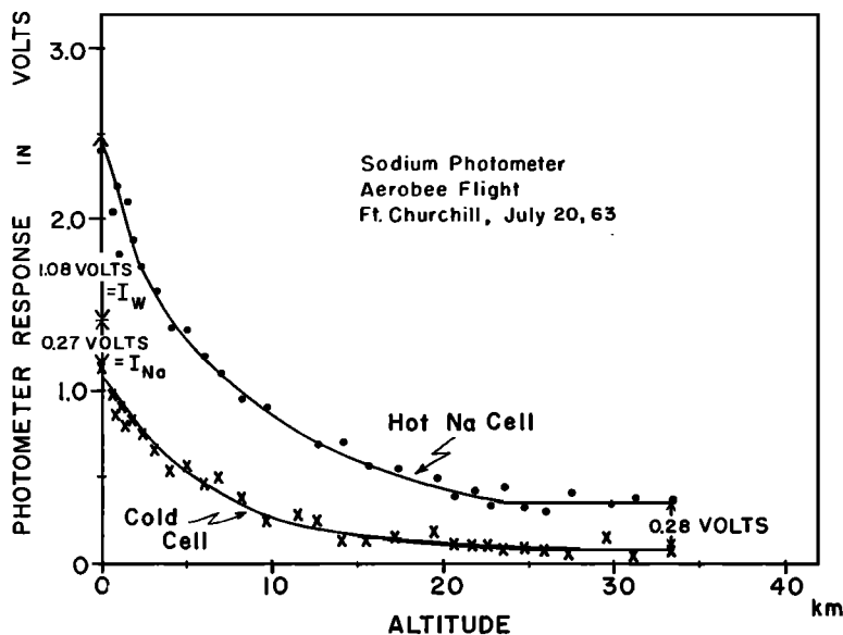
Fig. 11. Data from rocket sodium photometer flight, Fort Churchill, July 1963. Units are telemetered electrometer output signals. The ground-level decomposition into sodium emission I_{Na} , and white light I_w , is indicated along the ordinate scale.
