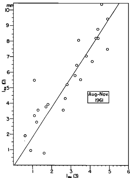
Fig. 6. Sodium dayglow signal at zero field plotted against sodium dayglow signal at 2000 oersteds.
