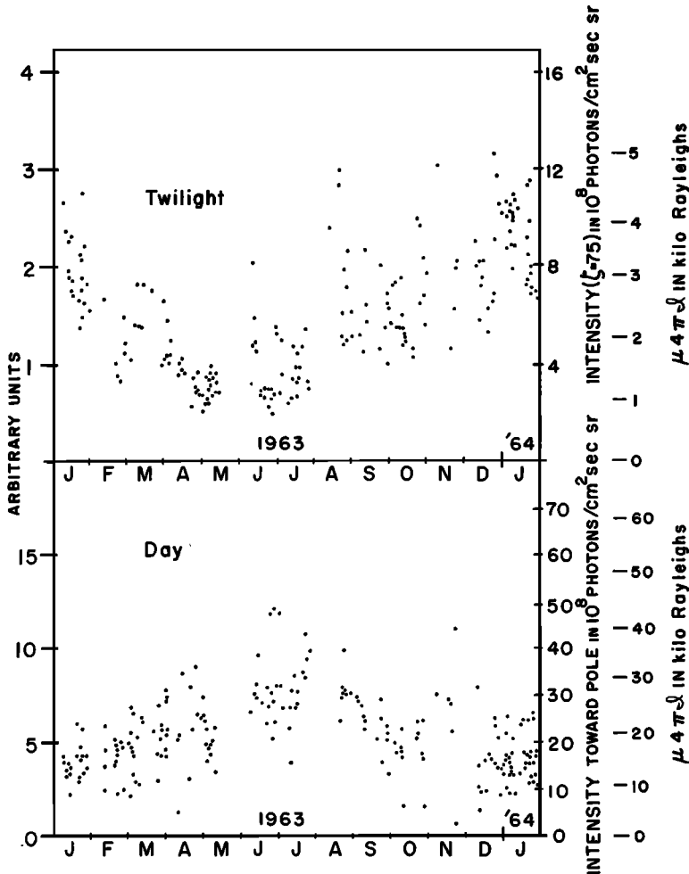
Fig. 12c. Sodium twilight-glow and dayglow intensities 1963, Haute Provence. Emission rate scale in kilorayleighs applies to zenith. Dayglow data are for a solar elevation angle of 30^\circ except for November, December, and January, when they are for 20^\circ .
