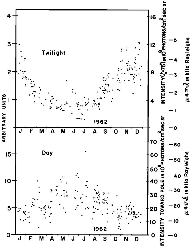
Fig. 12b. Sodium twilight-glow and dayglow intensities 1962, Haute Provence. Emission rate scale in kilorayleighs applies to zenith. Dayglow data are for a solar elevation angle of 30° except for November, December, and January, when they are for 20°.
