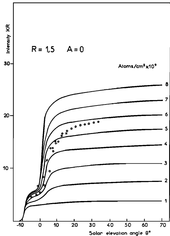
Fig. 7. Sodium intensity as a function of solar elevation angle and different abundances for R = 1.5 and A = 0 .
