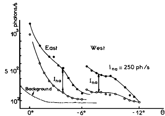
Fig. 3. Experimental twilight data for October 15, 1969.
