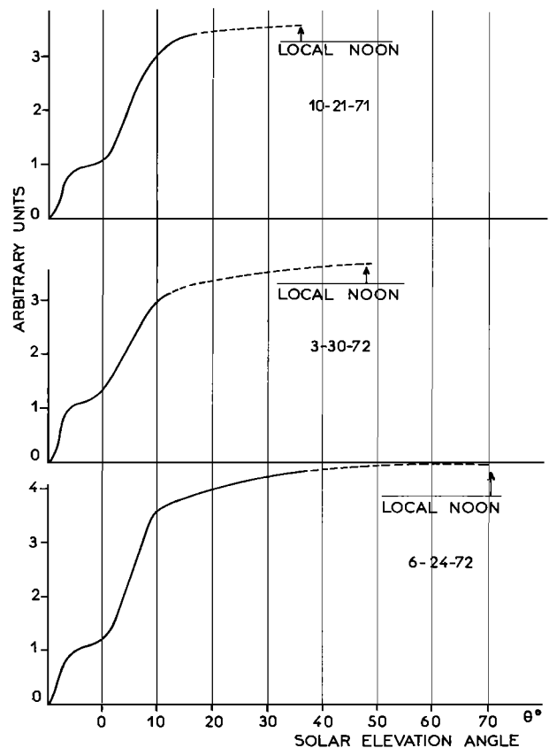
Fig. 5. Experimental results for the three flights. The dotted line is extrapolated.
