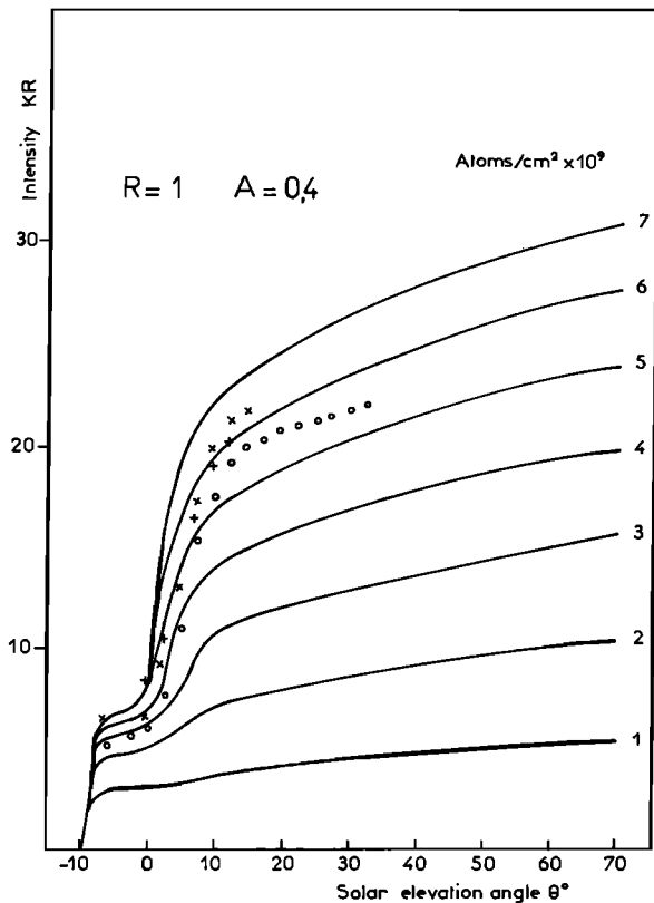
Fig. 8. Sodium intensity as a function of solar elevation angle and different abundances for R = 1 and A = 0.4 .
