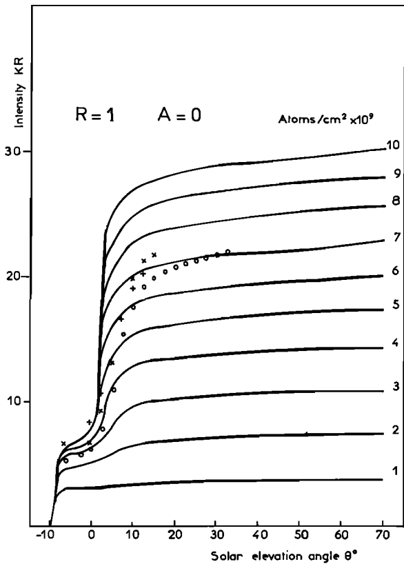
Fig. 6. Sodium intensity as a function of solar elevation angle and different abundances for R = 1 and A = 0 .
