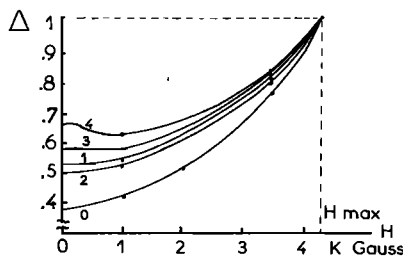
Fig. 1. Magnetic scanned profiles obtained on October 15, 1969: 0, direct sunlight; 1, dayglow at 1000 UT; 2, dayglow at 1200 UT; 3, dayglow at 1500 UT; and 4, dayglow at 1600 UT.
