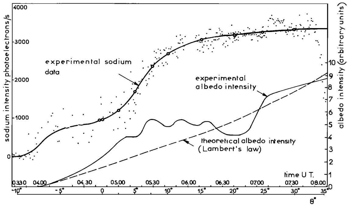
Fig. 4. Results of flight 3 on June 24, 1972. The points represent experimental sodium intensity data corrected for parasitic light and dark current. The heavy curve is the least mean squares fitting to the data. The light curve is the albedo intensity measurement. The dotted line is the theoretical albedo intensity according to Lambert's law.
