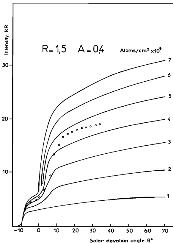
Fig. 9. Sodium intensity as a function of solar elevation angle and different abundances for R = 1.5 and A = 0.4 .
