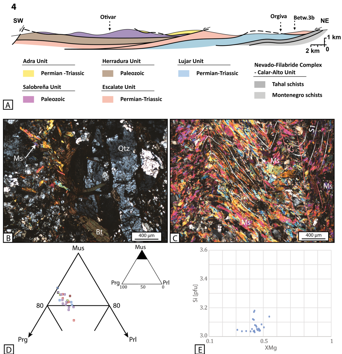
Figure 8. Summary of the structure, petrography and chemical composition for the sample Betw.3b. (a) Geological and tectonic cross-section of the sampled area and location of the sample, modified after Azañón et al. (1998). (b and c) Thin-section observations of the dated sample (polarized light). (d) Ternary composition plot for white micas. (e) Variation of X_{Mg} versus Si^{IV} contents in white micas.
