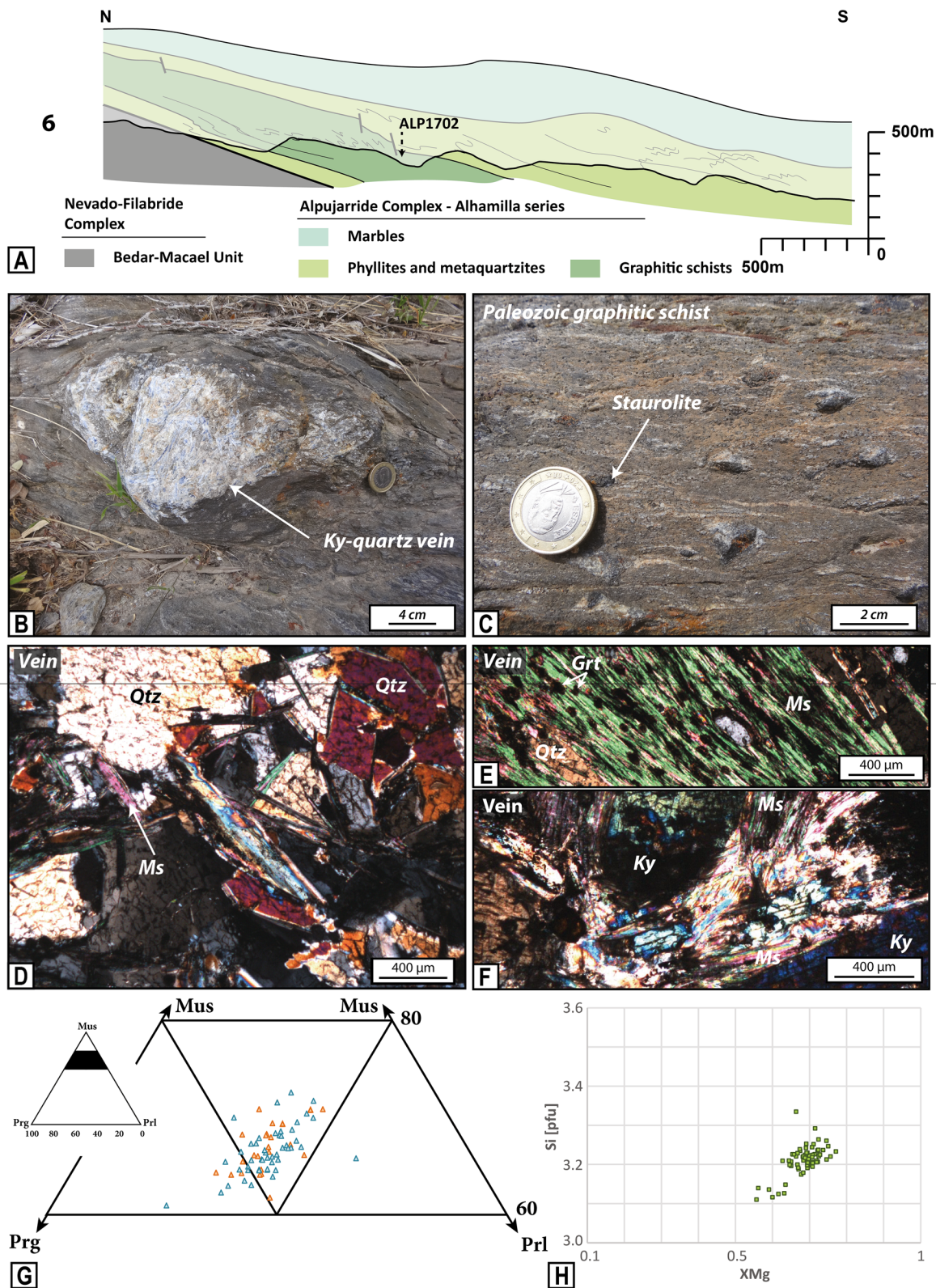
Figure 10. Summary of the structure, petrography and chemical composition for the sample ALP1702. (a) Geological and tectonic cross-section of the sampled area and location of the sample, modified after Platt et al. (1983). (b and c) Outcrop pictures showing a kyanite vein wrapped by the S2 within the host rock. (d–f) Thin section observations of the dated sample (polarized light). (g) Ternary composition plot for white micas. (h) Variation of X_{Mg} versus Si^{IV} contents in white micas.
