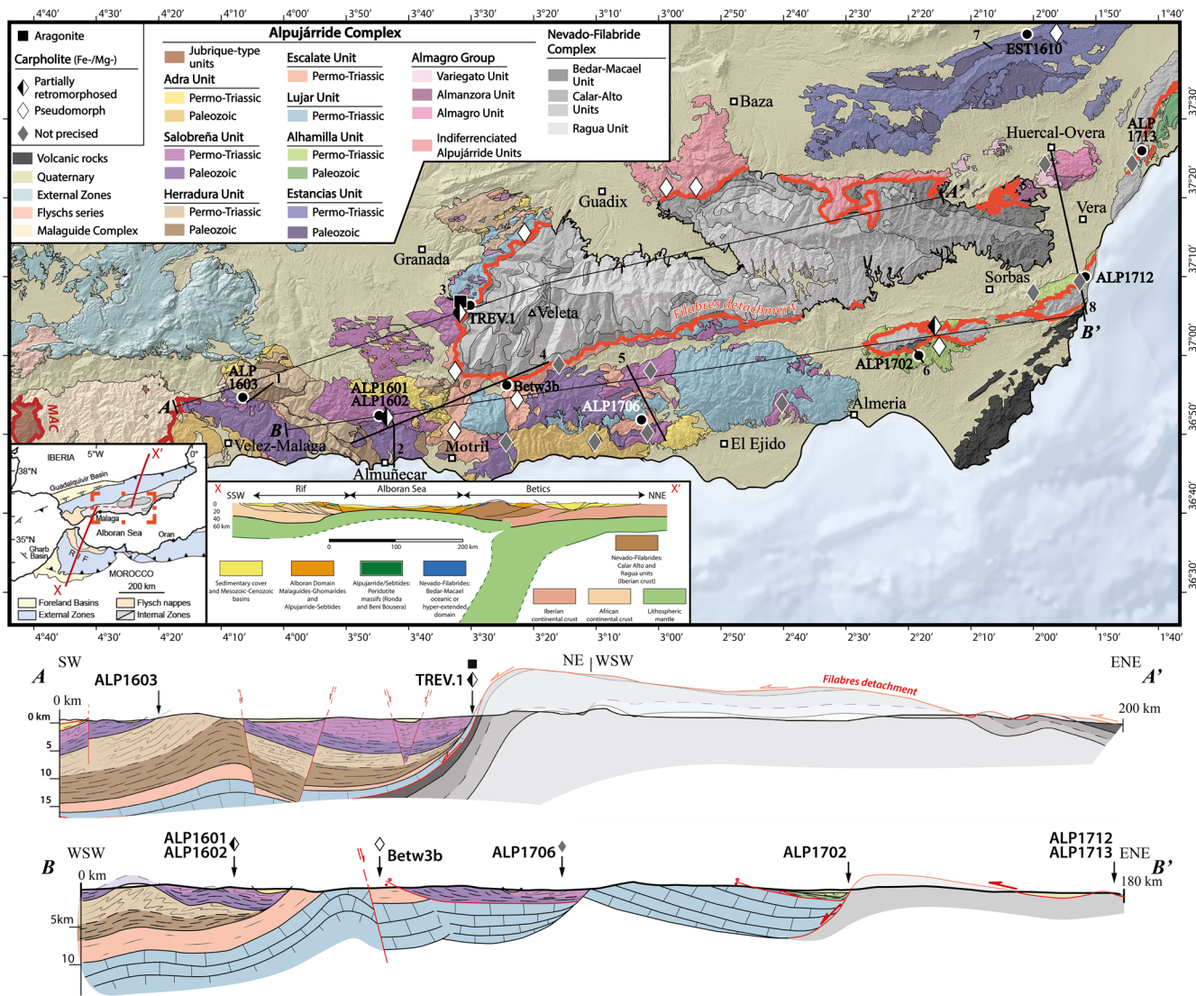
Figure 1. Geological and metamorphic map of the Betic Cordillera. Location of the Betic Cordillera belt within the Gibraltar arc. Detailed geological and tectono-metamorphic map of the Internal Zones of the Betic Cordillera, with the location of the studied area, and the location of the cross-sections. Regional cross-sections (A-A' and B-B') show the large-scale tectonic features of the study area. Position of the dated samples are projected, as well as the smaller-scale sections presented in Figures 5–12.
