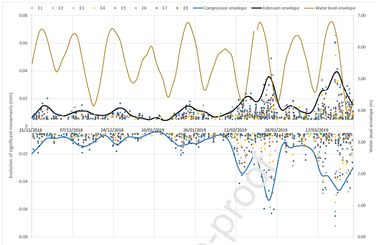
Figure 4: Extract of significant movement data from the eight extensometers (E, numbering from the middle (7 m IGN69) to the top of the cliff face (15 m IGN69) (Figure 2b)) from 21 November 2018 (00:00) to 31 March 2019 (22:00). The envelopes of the extension and the compression data considering all the extensometers are plotted in black and blue, respectively. The envelope of the water level data is plotted as well, to visualize the tidal cycles.
