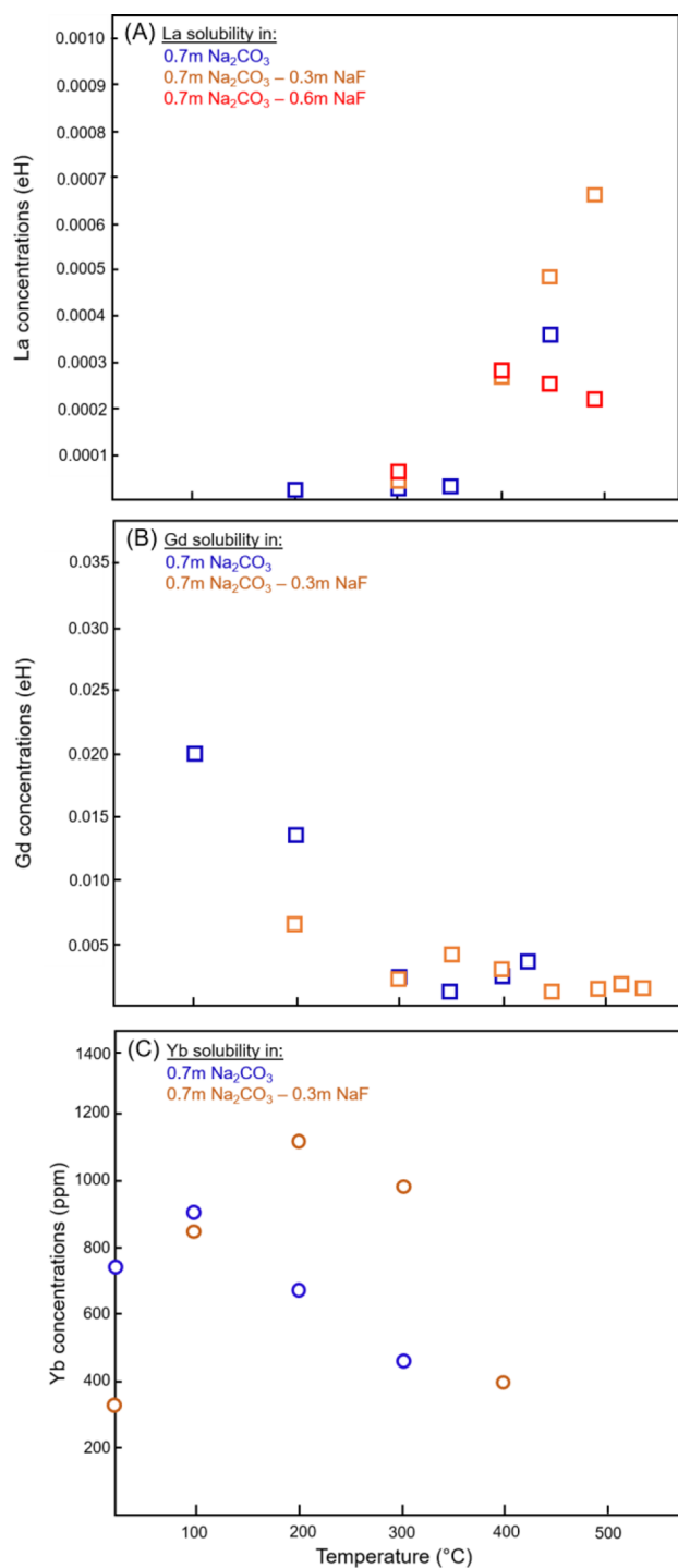
Fig. 2 Effect of temperature on the concentrations of La (A), Gd (B), and Yb (C) in Na 2 CO 3 ± NaF solutions. Solubility trends for La and Gd are here represented as the absorption edge height (eH) value from fluorescence spectra. This value is correlated to the concentration of the REE in solution, but may be affected by changes in density and absorption of the different solutions with increasing P-T (see “Methods” section). Therefore, it is only an indication of solubility behavior and cannot be used to directly calculate the concentration of La and Gd in the solution. For Yb, absolute concentrations could be calculated from the transmitted spectra, and are reported as ppm Yb in solution.
