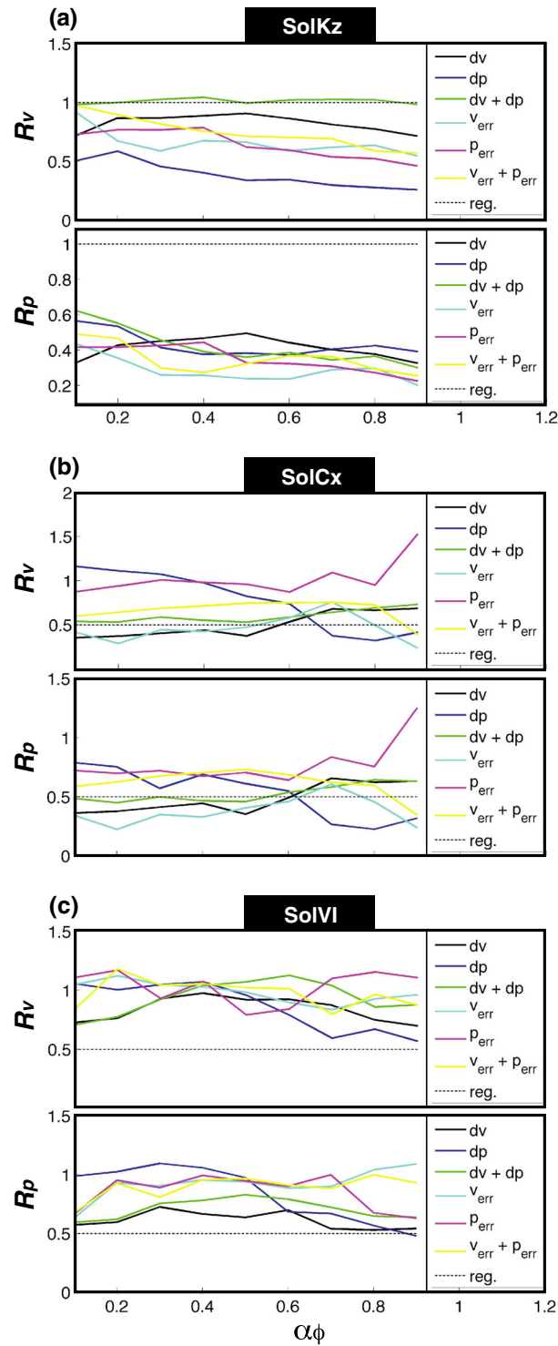
Figure 6. Error reduction rates for as a function of \alpha_\Phi (equation (47)). Color lines represent different refinement indicators ( \Phi = \{\Delta_v \Delta_p v_{\text{err}} p_{\text{err}}\} ). The dashed lines correspond to the nonadaptive solution L_1 error reduction rate which is constant for each given problem. (a) SOLKZ, (b) SOLCX, and the inclusion test (c) SOLVI.
