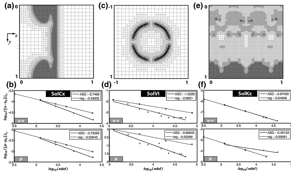
Figure 5. Mesh geometry and discretization errors using adaptivity based on the true discretization error. All tests employed both v_{err} and p_{err} as refinement criteria. (a, c, and e) The adaptive mesh geometry at the end of each test (up to eight levels). (b, d, and f) The decrease of L_1 discretization error with increasing N_{dof} . For comparison, nonrefined results using the standard staggered grid (reg) are shown for comparison (dashed lines). Figures 5a and 5b relate to SOLCX, Figures 5c and 5d relate to SOLVI, and Figures 5e and 5f relate to SOLKZ.
