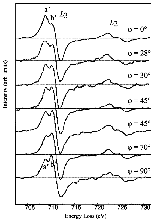
FIG. 5. Fe 2p EELS first derivative spectra for x=0.67 brownmillerite. The evolution of the a'/b' fine-structure ratio with the orientation of the crystal reflects the anisotropy due to the crystal-field interaction.
