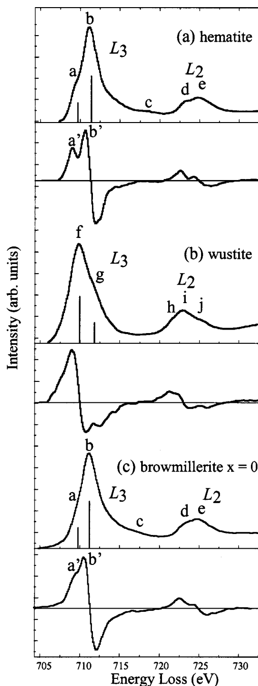
FIG. 3. Comparison between the Fe 2p EELS spectrum of (a) hematite, (b) wüstite, and (c) x=0 brownmillerite. The first derivative spectra are also shown in order to emphasize the fine-structure difference between the three compounds.
