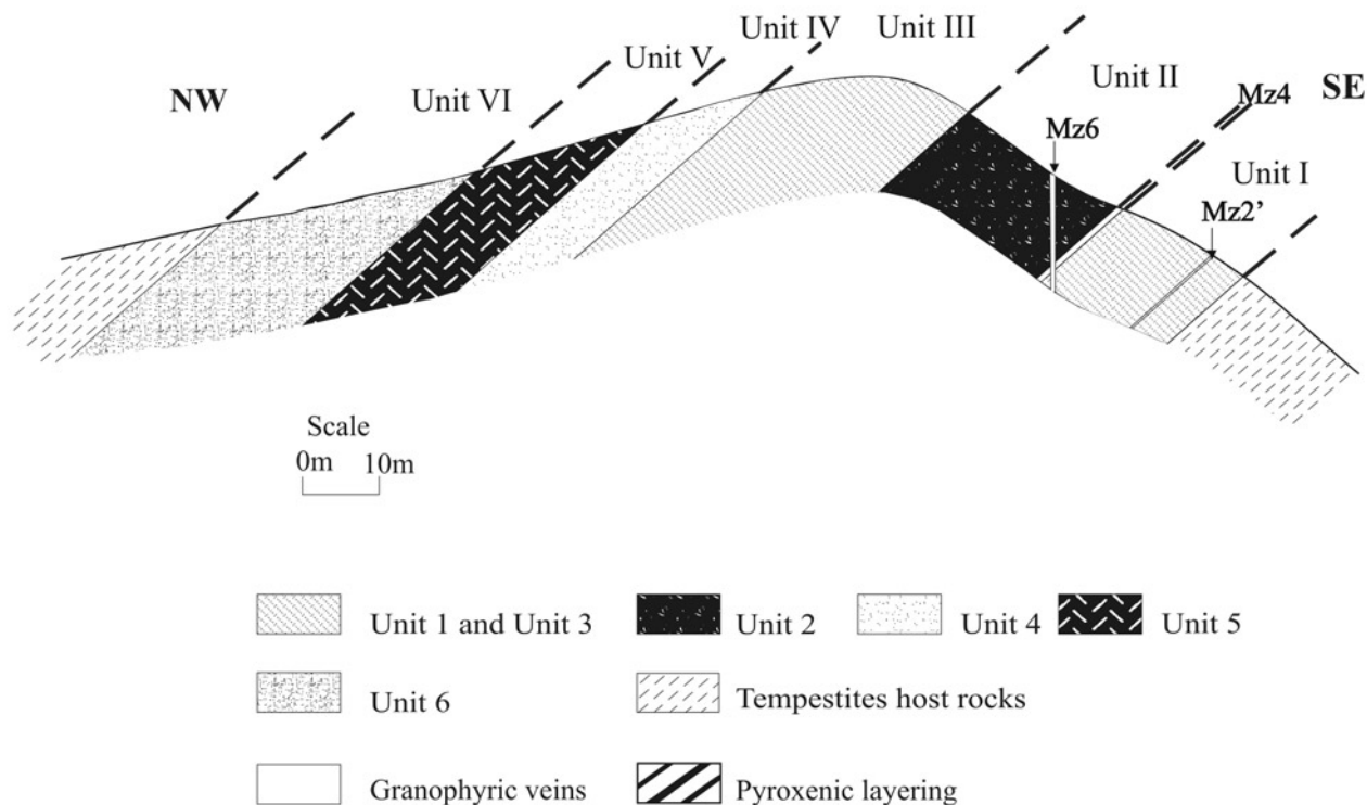
Figure 9. Simplified cross section of Marziqallal sill.
