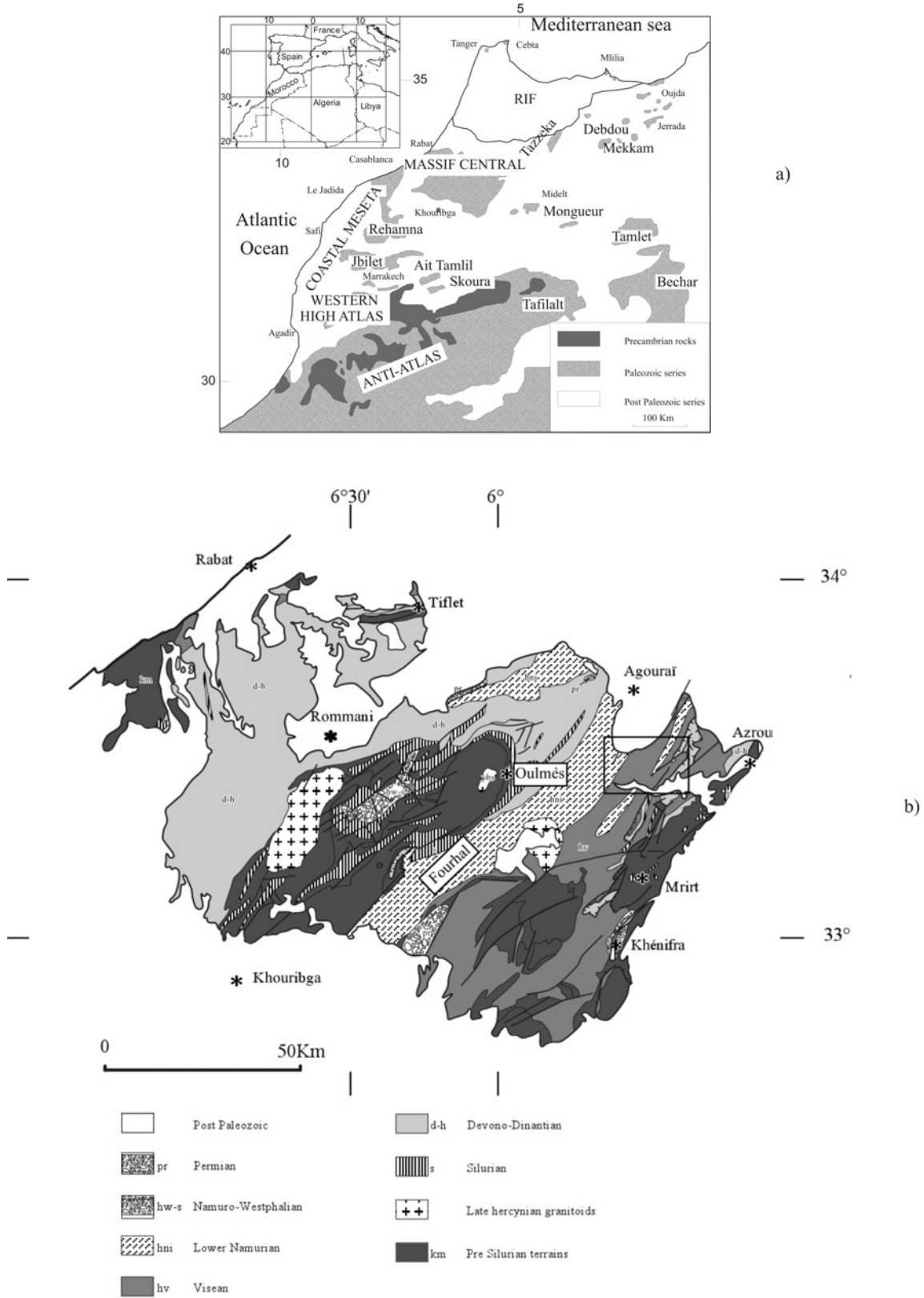
Figure 1. (a) Map of the Paleozoic outcrops in Morocco (modified from Piqué and Michard [1989]; reprinted by permission of American Journal of Science). (b) Geological map of the Moroccan Massif Central. The rectangle delineates the area shown in Figure 3.
