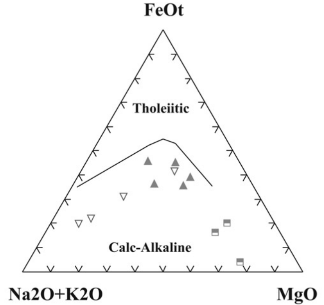
Figure 6. AFM diagram of Irvine and Baragar [1971]. Symbols are as follows: ▲ : basalts; ▽ : granophyric vein; ■ : basalts analyzed by Kharbouch [1994].
