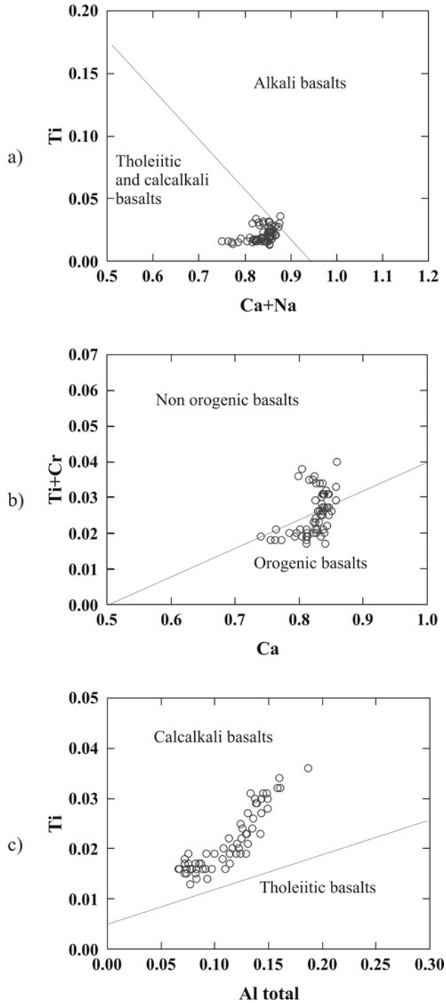
Figure 5. Discrimination diagrams of Leterrier et al. [1982] (reprinted with permission from Elsevier Science). (a) First discrimination diagram for clinopyroxene phenocrysts from alkali basalt and other basalts. (b) Second discrimination diagram for nonalkali basalts between nonorogenic tholeiites and orogenic basalts. (c) Third discrimination diagram for orogenic basalts between calcalkali basalts and tholeiitic basalts.
