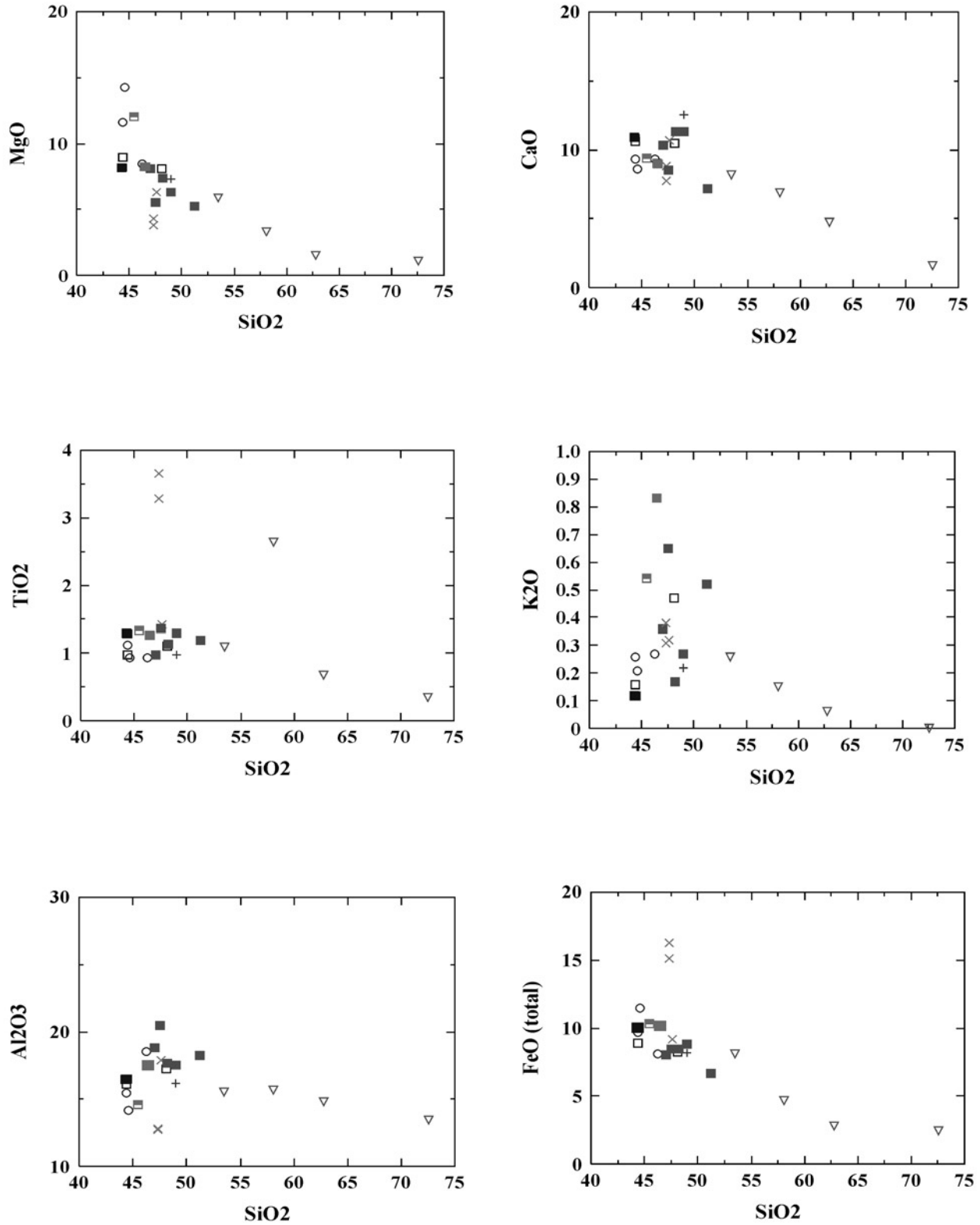
Figure 11. Plot of MgO, CaO, TiO 2 , K 2 O, Al 2 O 3 , FeO t vs. SiO 2 (in wt %) for Marziqallal rocks. See Figures 6 and 7 for symbols.
