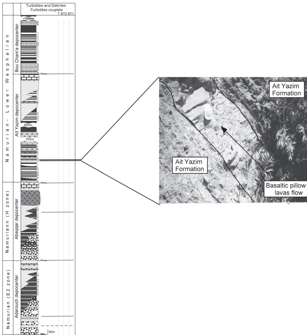
Figure 4. Simplified sedimentary column (modified from Ben Abbou et al. [2001]; reprinted with permission from Life Sciences).
