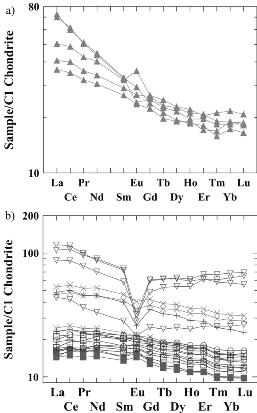
Figure 7. Concentrations of the rare earth elements (REE) for the Fourhal volcanic sequence (a) and the Marziqallal rocks (b). C1 chondrite values of Sun and Mc Donough [1989]. Symbols are as follows: \square : Unit 1 (Marziqallal sill); \blacksquare : Unit 2; + : Unit 3; \diamond : Unit 4; \times : Unit 5; \circ Unit 6; See Figure 6 for other symbols.
