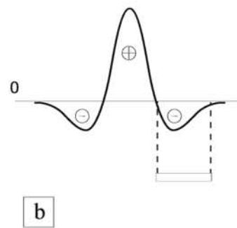
Negative Wavelet Coefficient
