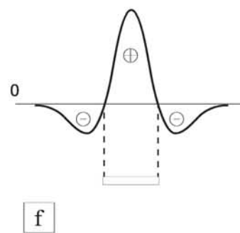
Maximum Wavelet Coefficient
