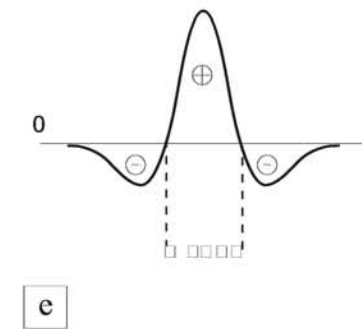
Strong Wavelet Coefficient
