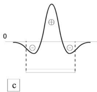
Weak Wavelet Coefficient
