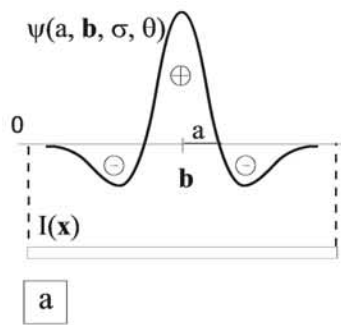
Null Wavelet Coefficient
