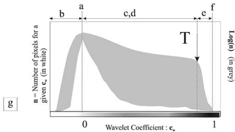
Strong Wavelet Coefficient
