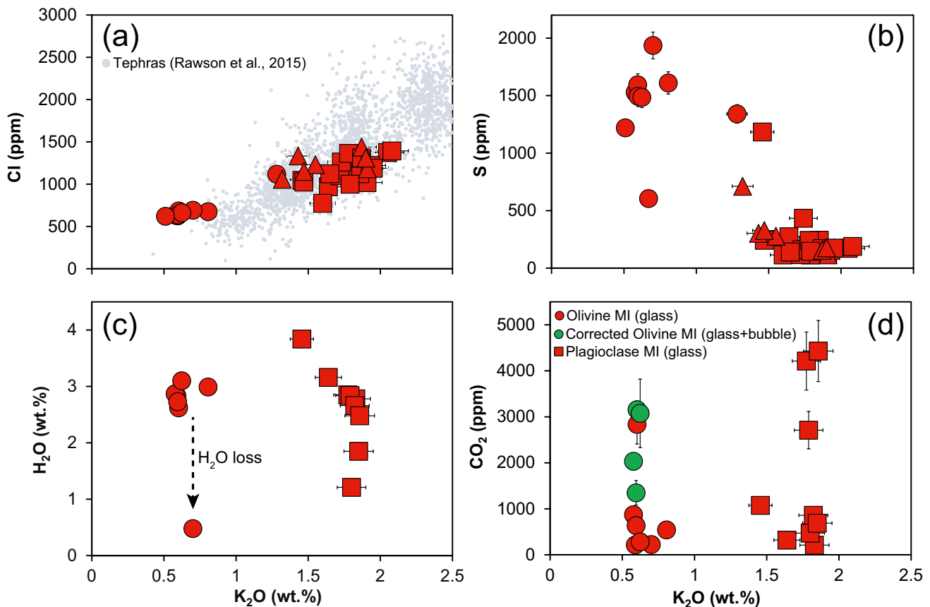
Fig. 4 a–d Volatile contents relative to K 2 O contents of the studied MIs. For four olivine-hosted MIs, both corrected (bubble + glass) and uncorrected (only glass) CO 2 contents are reported. The variability of S, H 2 O, and CO 2 observed for a given K 2 O value is an evidence of
