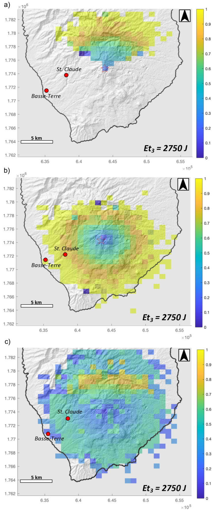
Fig. 8. Probability maps \theta^{cc}_{A_{ij,m}} to exceed E_{t3} (2750 J) considering the hypothetical scenario of a single vent located at a) 643820 E; 1,774,748 N (altitude: 1416 m), and b) 643,451 E; 1,774,316 N (altitude: 1273 m); c) Probability map \theta^f_{A_{ij,m}} to exceed E_{t3} (2750 J) considering the uncertainty on vent opening through the combination of more vents on the dome area.
