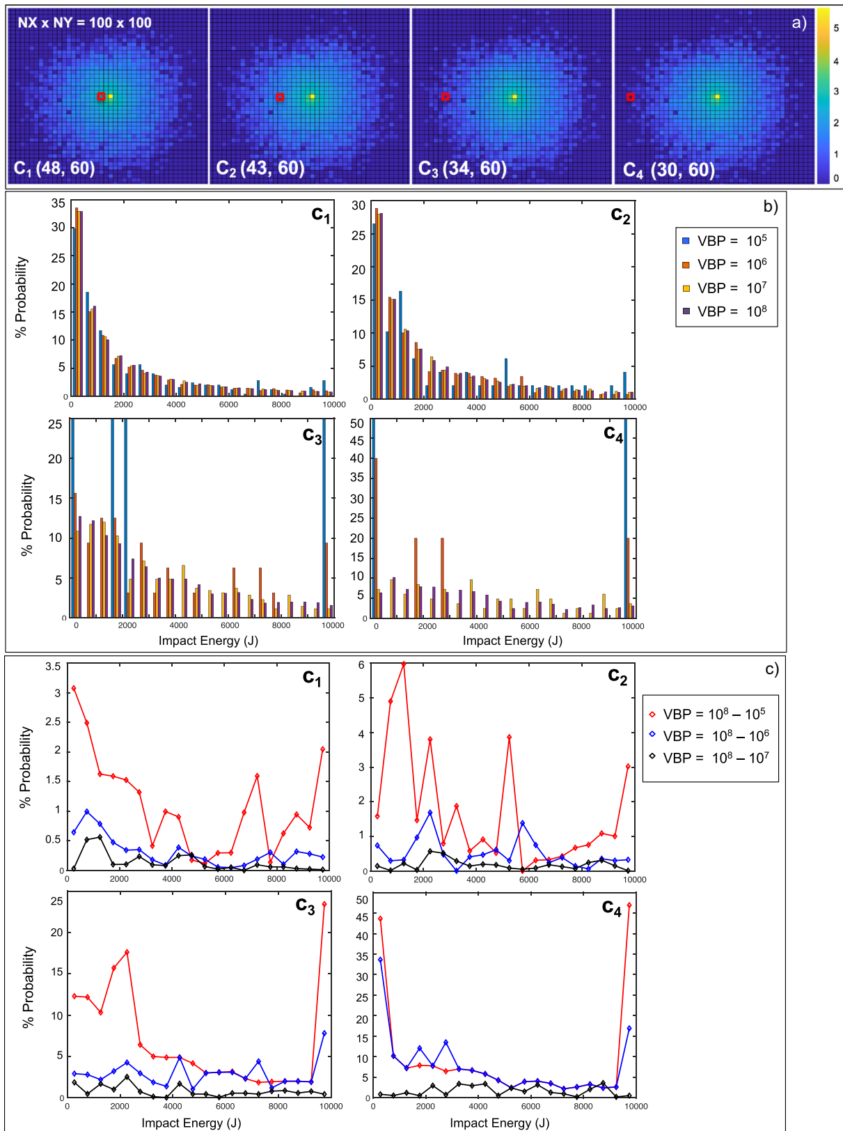
Fig. 5. a) Map showing the \text{Log}_{10} of the number of VBPs fallen in each cell of the domain, in the case of 10^7 clasts ejected. ESPs are from Table 3. In red the location of the four cells ( C_1 , C_2 , C_3 , C_4 ) selected for the sensitivity analysis. b) Probability (%) of ballistic impact energy for 20 energy classes for different numbers of VBPs launched in simulations: cell C_1 , dome area, ca. 500 m from vent; cell C_2 , Hospital, ca. 2600 m from vent; cell C_3 , centre of St. Claude, ca. 4000 m from vent; d) cell C_4 , point at ca. 5200 m from the vent. The cell coordinates referred to the grid with resolution of 100 \times 100 are reported in bracket; c) Probability (%) curves showing the absolute difference between the probability associated to different numbers of released VBPs ( 10^8 - 10^5 red line, 10^8 - 10^6 blue line, and 10^8 - 10^7 black line), for cells C_1 , C_2 , C_3 , C_4 . The cell coordinates referred to the grid with resolution of 100 \times 100 are reported in brackets.
