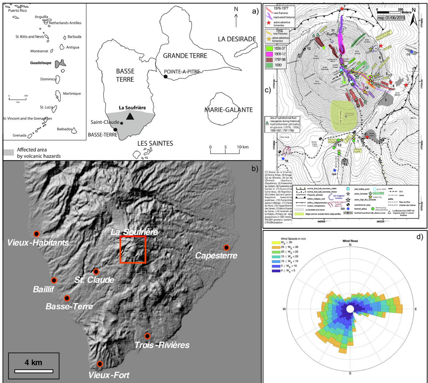
Fig. 1. a) Map of Guadeloupe showing the active volcano La Soufrière, and the major towns (St. Claude, Basse-Terre, Pointe-à-Pitre). Inset map showing the location of Guadeloupe in the Antilles region (modified from Chenet et al., 2014). b) Digital Elevation Model (DEM) of the computational domain, including the southern part of the Basse-Terre island. The main urban centres are indicated with black-red dots. The DEM resolution is set to 10 m; c) Location map of the main structures, historical eruptive vents, observed fumarolic activity on La Soufrière lava dome (modified from the OVSIG-IPGP report, October 2018); d) Windrose diagram showing the daily wind conditions at La Soufrière during 2017–2018 from the “Piton Sanner” meteorological station located on the top of the dome.
