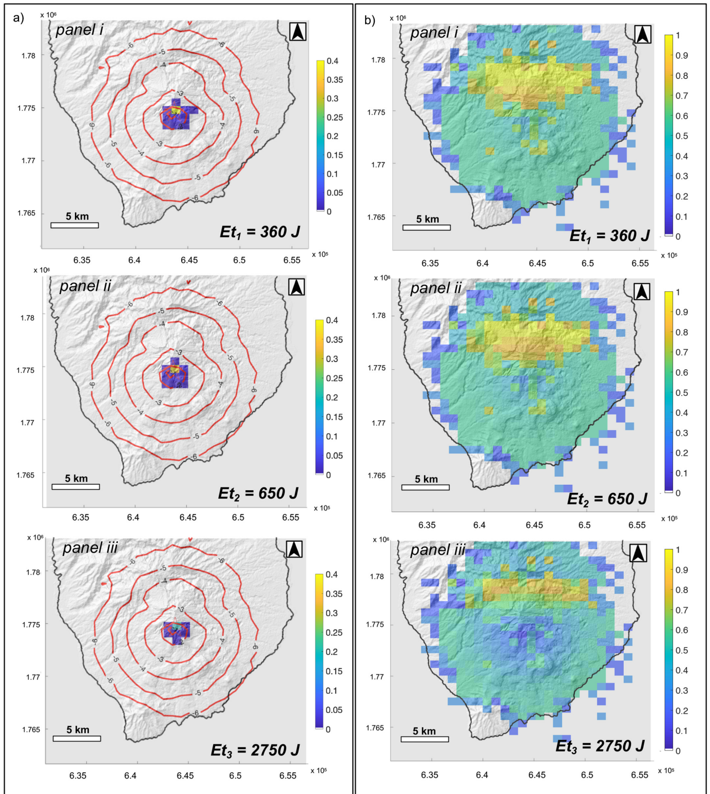
Fig. 9. a) Probability maps \theta^c_{A_{ij},m} of VBPs exceeding energy thresholds (Table 3; panels i-ii-iii) in absence of wind, according to the eq. (10). Red contours represent the \text{Log}_{10} of the component \theta^c_{A_{ij}} which is the probability that a VBP reaches the cell A_{ij} weighted for \omega'_k . All probabilities are conditional to the ejection of a clast during an eruption within the adopted scenario and from the dome; b) Probability maps \theta^{pc}_{A_{ij},m} of VBPs exceeding energies thresholds (Table 3; panels i-ii-iii) in absence of wind, according to eq. (9).
