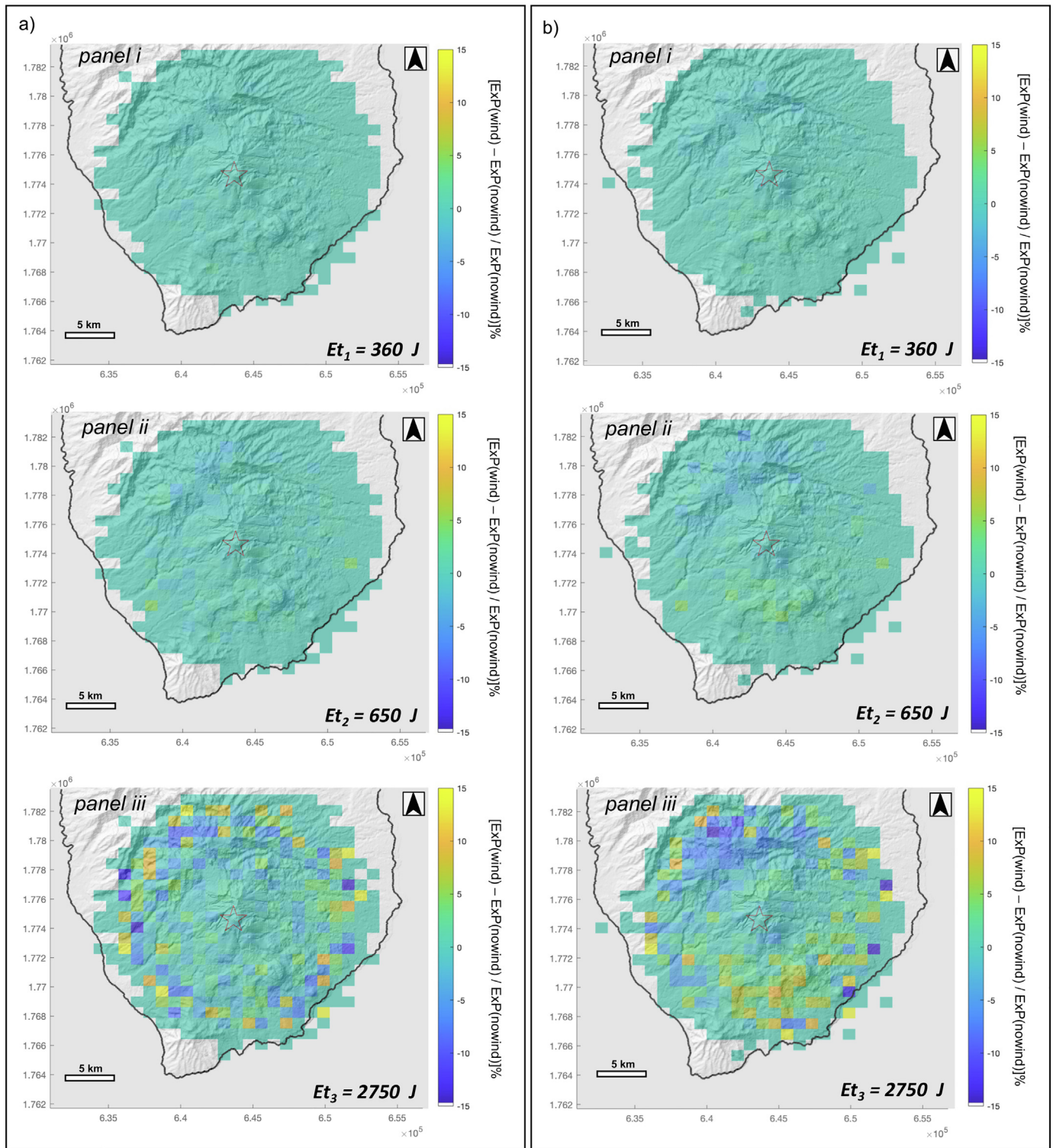
Fig. 7. Sensitivity analysis on wind conditions showing the relative difference between the exceedance probabilities P_{A_{i,j,m}}^{EC} referred to E_{t1} = 360 J (panel i), E_{t2} = 650 J (panel ii), and E_{t3} = 2750 J (panel iii), in case of a) minimum ( W_s = 2 m s -1 , W_d = 279^\circ ) and absent wind conditions. The same test was carried out in considering b) maximum ( W_s = 25 m s -1 ; W_d = 343^\circ ) and absent wind conditions. For all tests, the vent is located at the centre of the dome area (star).
