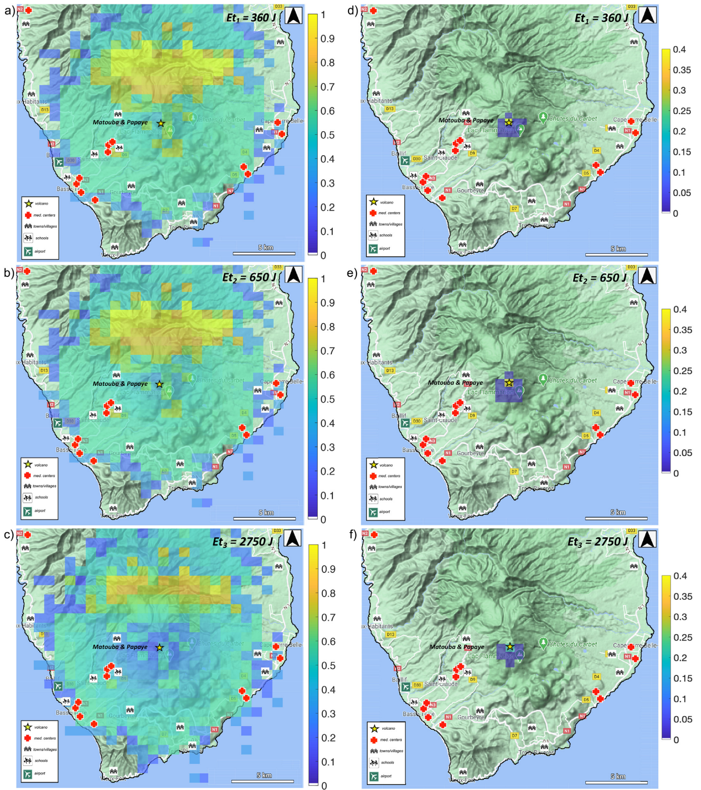
Fig. 10. Exposure-based risk analysis considering the conditional probability \theta^{c}_{A_{ij,m}} (a-b-c) and the overall probability \theta^{o}_{A_{ij,m}} (d-e-f) of VBPs exceeding selected energy thresholds (Table 3). All probabilities are conditional to the ejection of a clast during an eruption within the adopted scenario and from the dome, in absence of wind. Symbols in legend: yellow star: La Soufrière volcano; red cross: hospitals and clinics; two-houses: towns (i.e., St. Claude, Basse-Terre) and villages (i.e., Matouba and Papaye); running children: schools; airplane: airport). The location of each element has been identified at https://www.google.it/maps .
