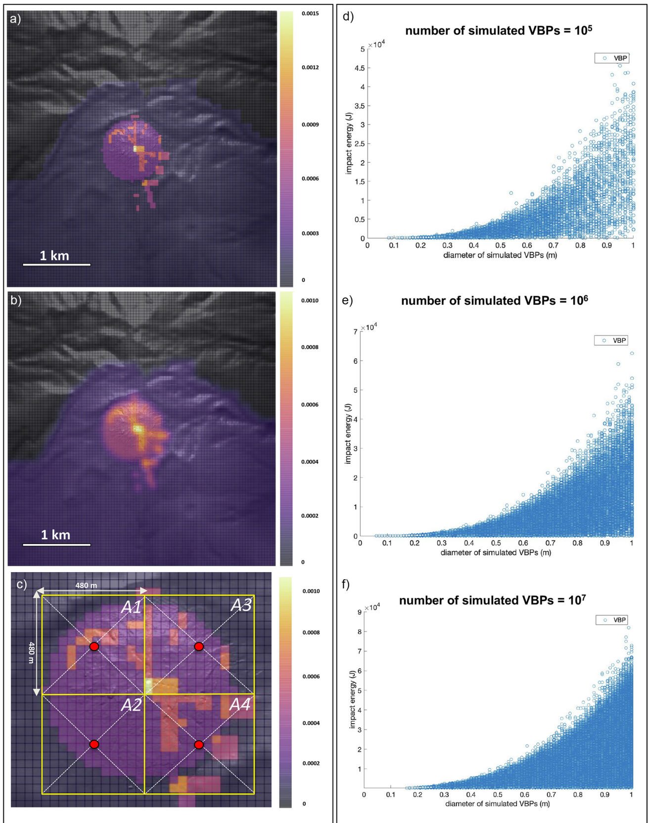
Fig. 2. a) Best-guess probability map of vent opening; b) Gaussian filter with \sigma = 40 m applied to consider the spatial uncertainty of the data and to avoid a scattered spatial distribution due to the limited sampling; c) Magnification of the spatial map displaying the probability of vent opening within four regular macroareas (A1, A2, A3, A4). The corresponding vents are located in the centre of each macroarea (red dots; A1: 643451 E, 1774608 N, altitude: 1344 m; A2: 643451 E, 1774316 N, altitude: 1273 m; A3: 643820 E, 1774748 N, altitude: 1426 m; A4: 643820 E, 1774316 N, altitude: 1345 m). Plots of the VBPs diameter vs impact energy are shown in: d) fixed VBPs = 10^5 ; e) fixed VBPs = 10^6 ; f) fixed VBPs = 10^7 . The diameter of the simulated clasts ranges between -9.89 1.66 \phi .
