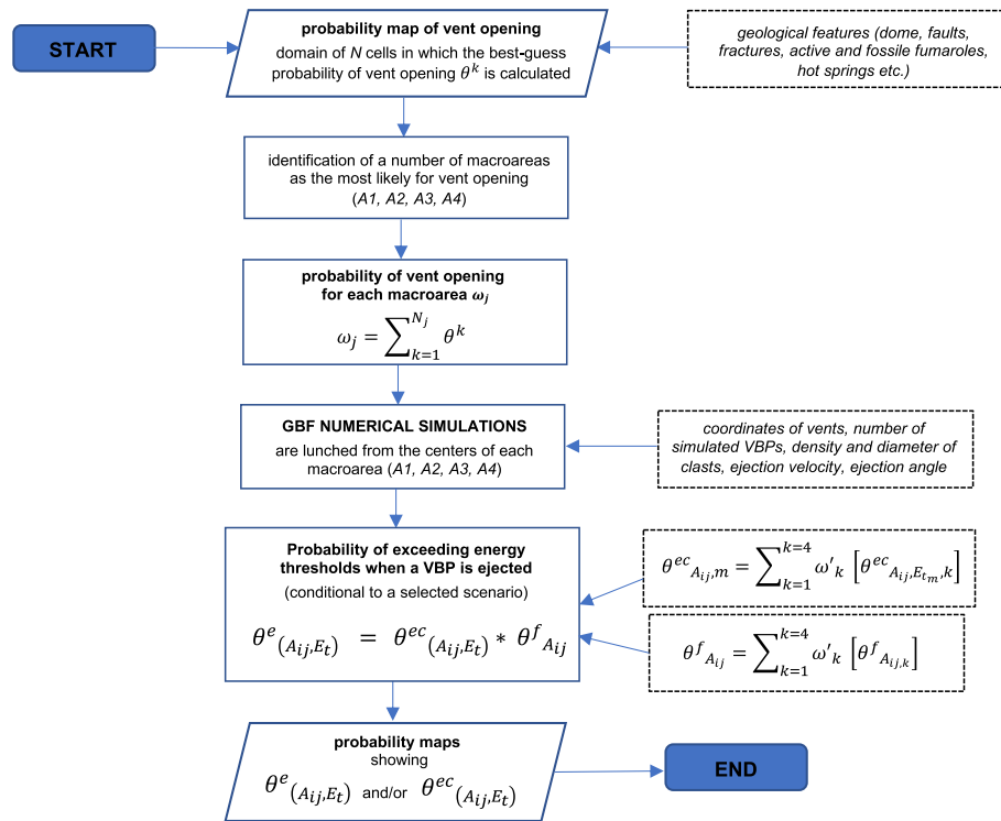
Fig. 3. Flowchart of the logical process describing how to calculate the overall exceedance probability accounting for the vent position uncertainty.
