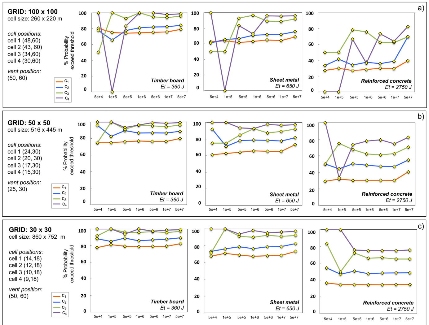
Fig. 6. Sensitivity of the probabilistic hazard assessment strategy for the number of released VBPs with respect to the resolution of the grid used to quantify the probability (%) of VBPs exceeding a given energy threshold E_t : a) 100 \times 100 cells; b) 50 \times 50 cells; c) 30 \times 30 cells. The four lines represent the four cells on which probabilities were calculated (cell c_1 , orange, cell c_2 , blue, cell c_3 , green, cell c_4 , violet) at different grid resolutions. The cell coordinates referred to a)-b)-c) resolution grids are reported in brackets.
