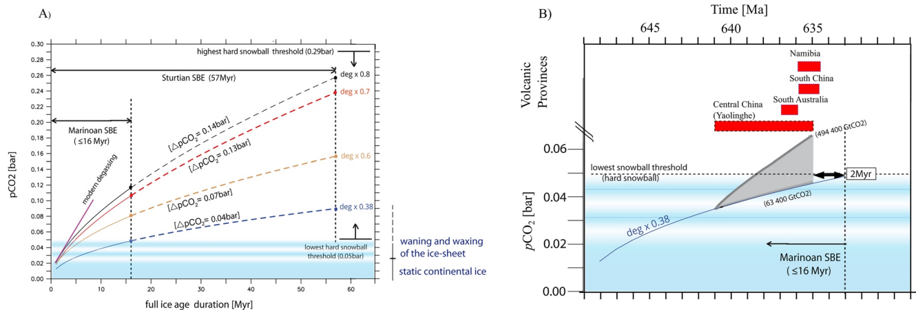
Figure 3. p\text{CO}_2 simulated by a biogeochemical model (GEOCLIM) forced by a climate model coupled with an ice-sheet model (Benn et al., 2015) (a) Temporal p\text{CO}_2 evolution with different background degassing rates in the context of a hard snowball Earth. Dashed lines represent the amount of carbon between short and long snowball events. Melting thresholds for short and long snowball events are based on their duration (16 and 57 Myr, respectively), all being encompassed within thresholds estimated by climate models from 0.29 (Pierrehumbert, 2004) to 0.05 bars (Benn et al., 2015) assuming a white surface (snow and ice). Melting thresholds for a mudball earth (Abbot & Pierrehumbert, 2010) can be estimated to be at least 1/3 of a clean snowball earth (i.e., 0.1 instead of 0.29 bar) while de Vrese et al. (2021) suggests lower p\text{CO}_2 for initiating melting. Ice-sheet behavior is based on climate-ice-sheet model simulations (Benn et al., 2015). (b) Influence of the Yaolinghe rift system and other volcanic provinces on the snowball Earth duration for deg038 experiment (aerial volcanic flux \sim 0.38 modern conditions). The emplacement has been integrated over 6 Myr to cover all volcanic provinces. Our simulations show how a speed-up in degassing would have foreshortened the Marinoan snowball Earth by 2–5 Myr (i.e., 11–14 Myr duration instead of 16 Myr) under various volcanic emission intensities (gray band).
