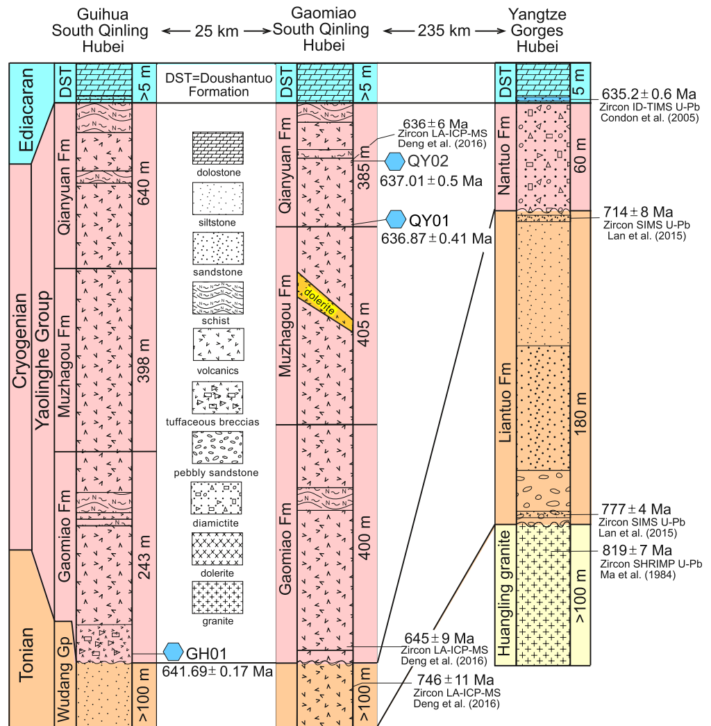
Figure 1. Lithostratigraphy of the Guihua and Gaomiao sections and sampling horizons. The Wudang and Yaolinghe groups in the South Qinling terrane correlate with the Liantuo and Nantuo formations, respectively, from the northern margin of the Yangtze block. Early Cryogenian and interglacial (720–650 Ma) sedimentary successions are absent due to uplift and erosion (e.g., Mitchell et al., 2019). Blue hexagons mark the sampling horizons, with sample names and zircon dates. Fm—formation. Gp—group.
