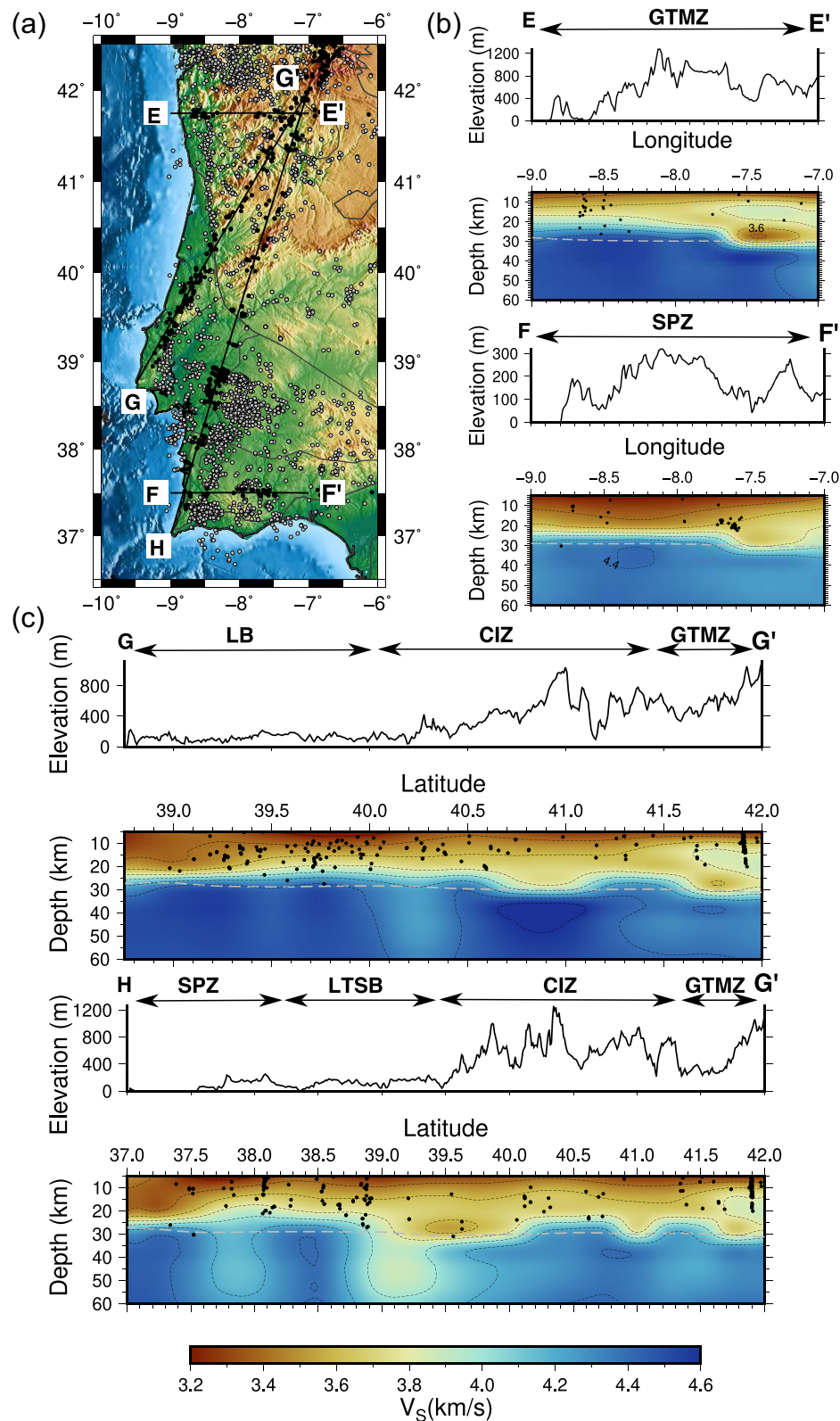
Figure 9. Vertical profiles through the 3-D S-wave velocity model. (a) Topographic map with the position of the four vertical profiles. Earthquakes recorded between 1995 and 2013 are plotted in grey or black dots if they are close to the selected profiles. (b) Profiles crossing the GTMZ (E–E') and the SPZ (F–F') zones. (c) Profiles along the contact between the LB and LTSE basins (G–G') and crossing all of Portugal from southwest to northeast (H–G'). S-wave velocities are plotted as absolute values. Earthquakes, relocated by Veludo et al. (2017), are plotted around the plotted profiles within an interval of \pm 0.05^\circ .
