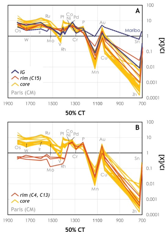
Fig. 8. Concentrations normalized to CI chondrites in CM chondrite metal grains from Paris and Maribo plotted against the 50% condensation temperature of siderophile and chalcophile elements (Lodders, 2003). (A) Core ( n = 24 ), rim (C15, n = 3 ) and isolated metal grains ( n = 2 ). Each line corresponds to a single grain. The data encompasses grains from 13 chondrule cores, 1 chondrule rim and 1 isolated grain. (B) Core and rim (C4, C13; n = 3 ) compositions from Paris.
