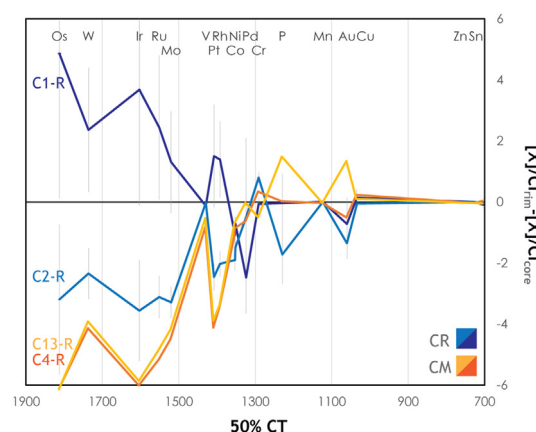
Fig. 16. Volatility patterns of rim metal grains from CR and CM chondrules, with the [X]/CI relative to the average core compositions plotted against 50% condensation temperature of elements. Zero on the y-axis represents the chondrule core metal composition. The rim labels correspond to those in Fig. 13e and f.
