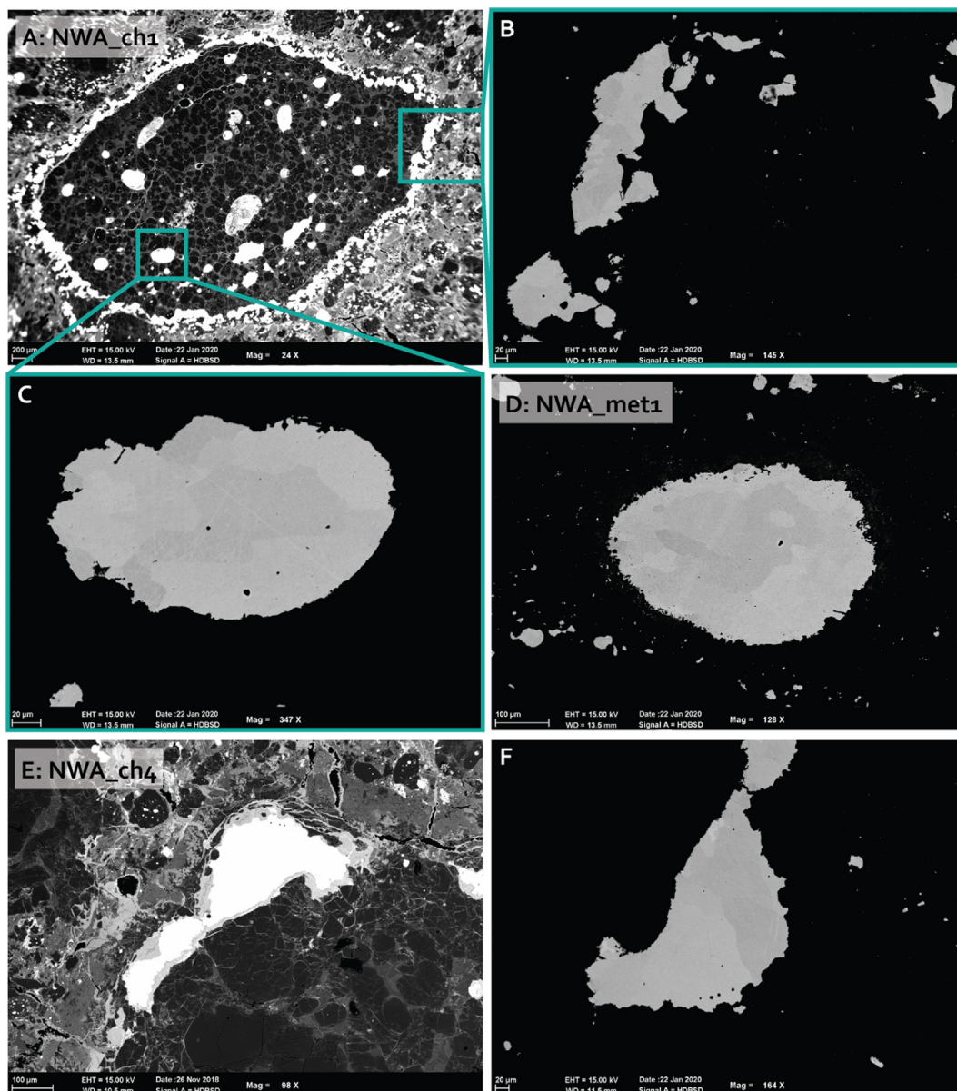
Fig. 1. Back scattered electron images of representative NWA801 CR chondrite metal grains. B and C are zoom-ins of A: NWA_ch1. Metal grains are shown with increased contrast (B, C, D, F) to highlight compositional zoning of Ni-poor (kamacite) and Ni-rich (taenite) regions. High resolution BSE images of all NWA801 metal grains used in this study can be found in Fig. S5.
