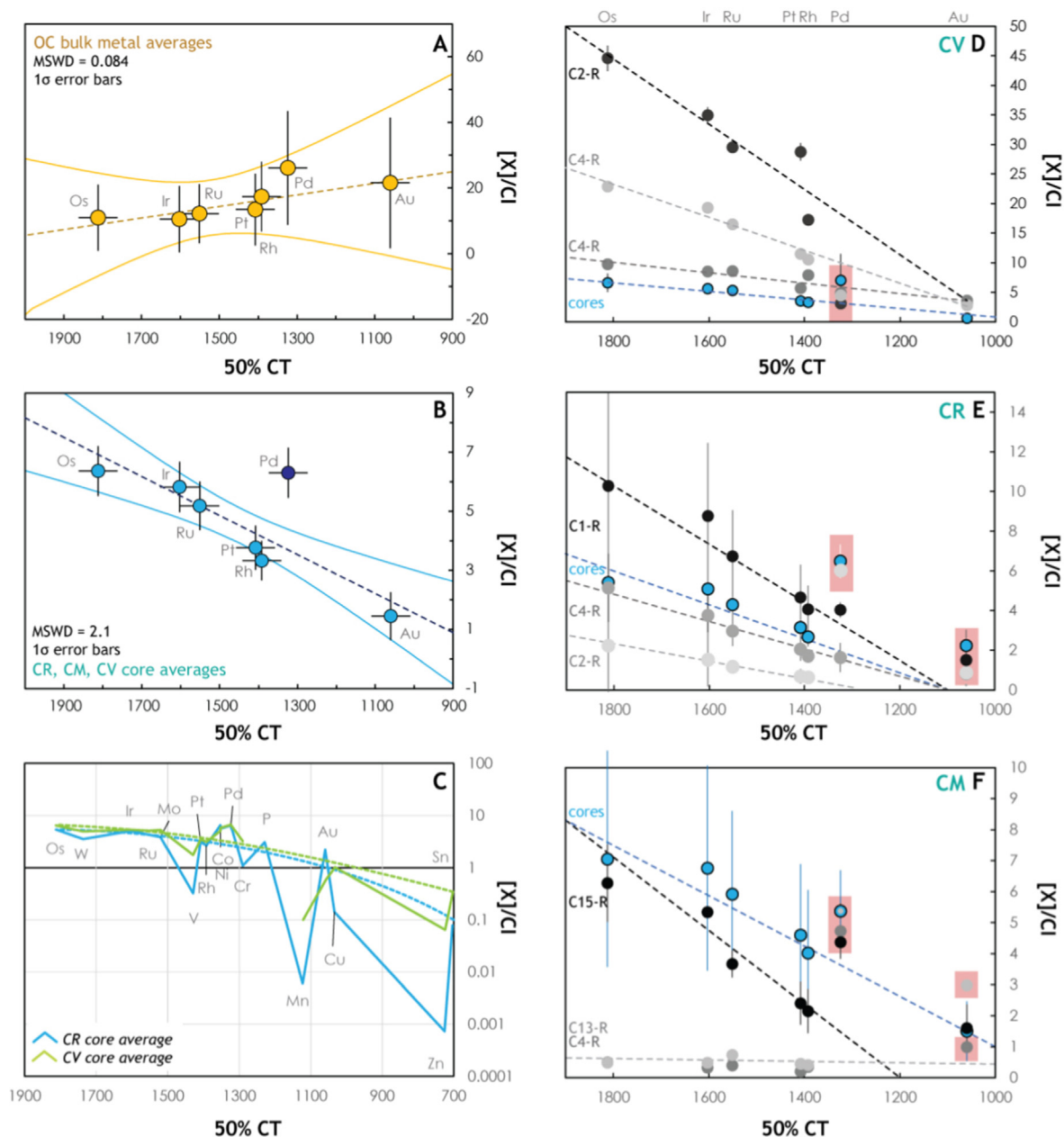
Fig. 13. Volatility patterns of HSE: HSE concentrations normalized to CI chondrites versus 50% condensation temperatures. Note the linear y-axis scale in panels A, B, D–F. (A) Ordinary chondrite (OC) bulk metal compositions from (Okabayashi et al., 2019). A Yorkfit regression is used, plotted with error envelope. The errors shown are 1SD of the mean. (B) Same figure as A, but with CV, CR and CM chondrite metal grains from chondrule cores averages in this study. The regression is taken through all HSE, but Pd is rejected as an outlier. (C) Metal grain volatility patterns from averaged CV and CR chondrule cores (solid lines) plotted with CV and CR chondrule core regression lines from panels D and E (dashed lines). (D–F) HSE from CV, CR and CM chondrule core (blue) and rim metal (grey tones). Errors are 1SD. CV rim metals correspond to single grains, whereas CR and CM contain rim averages of multiple grains. Dashed lines are regressions through the most refractory HSE: Os, Ir, Ru, Pt and Rh. The red boxes denote where Pd and Au deviate from these regressions.
