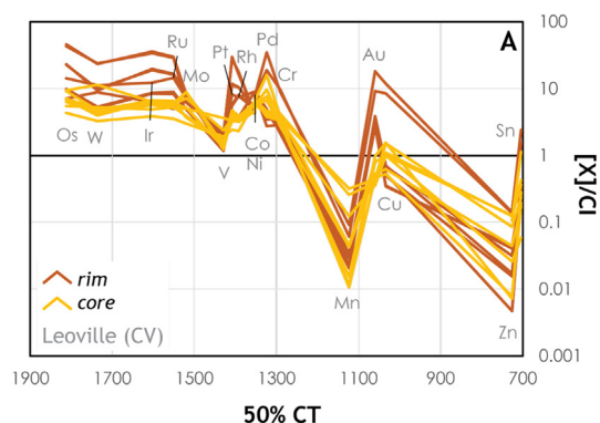
Fig. 10. Concentrations normalized to CI chondrites in CV chondrite metal grains from Leoville plotted against the 50% condensation temperature of siderophile and chalcophile elements (Lodders, 2003). (A) Core ( n = 7 ) and rim metal grains ( n = 8 ). Each line corresponds to a single grain. The data encompasses grains from 2 chondrule cores and 3 rim grains.
