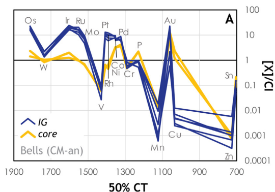
Fig. 9. Concentrations normalized to CI chondrites in CM-an chondrite metal grains from Bells plotted against the 50% condensation temperature of siderophile and chalcophile elements (Lodders, 2003). Core ( n = 2 ) and isolated metal grains ( n = 6 ). Each line corresponds to a single grain. The data encompasses grains from 2 chondrule cores and 6 isolated grains.
