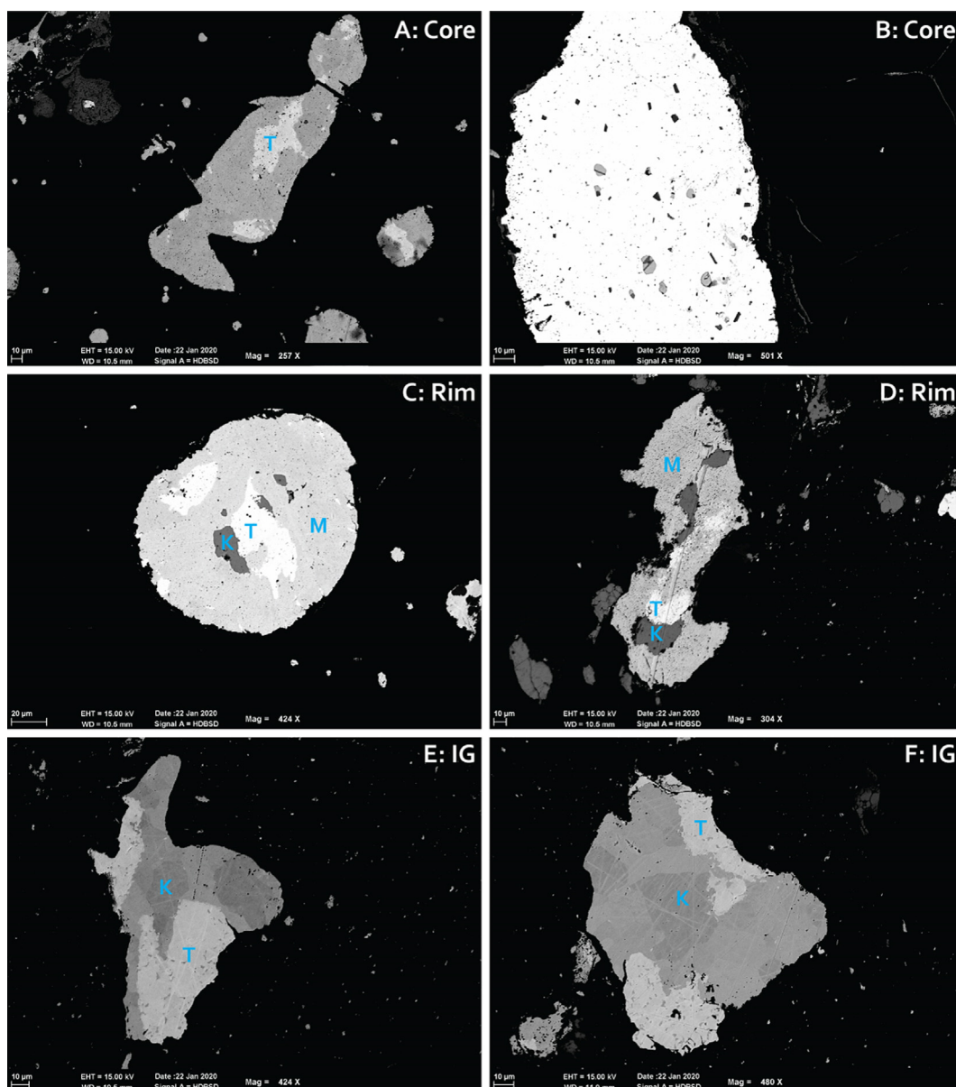
Fig. 4. Back scattered electron images of representative Leoville metal grains. A and B are grains from chondrule cores (ch3 and ch1), with taenite (T) exsolutions, black inclusions and grey silica inclusions in the case of ch1 (panel b). C and D are rim grains (c5 and met1), with kamacite (K) and taenite exsolutions in a martensite (M) host metal. E and F are isolated grains (IG). High resolution BSE images of all Leoville metal grains used in this study can be found in Fig. 8.
