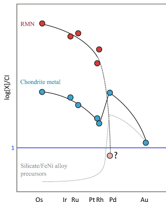
Fig. 15. A sketch of HSE concentrations normalized to CI chondrites of chondritic metal and potential precursors lined up according to their volatility. In red: RMN = the average composition of refractory metal nuggets in carbonaceous chondrites (Daly et al., 2017). The Pd concentration is estimated from RMN condensation models (Campbell et al., 2003); in blue: the averaged chondrite core metal composition from Fig. 13b; grey dashed line: estimated pattern of FeNi alloy and silicate chondrule precursors with 50% condensation temperatures <1350 K.
