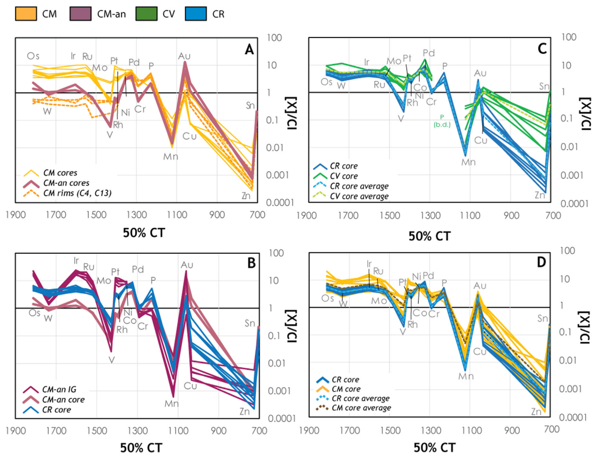
Fig. 11. Concentrations normalized to CI chondrites in CM, CM-an, CV and CR chondrite metal grains plotted against the 50% condensation temperature of siderophile and chalcophile elements (Lodders, 2003). (A) Compositions from CM core metal, CM rim metal (C4, C13) and CM-an core metal. (B) Bells IG and core metal grains versus NWA 801 core metal grains. (C) Leoville versus NWA801 core metal grains and their averages. (D) Paris versus NWA 801 core metal grains and their averaged compositions.
