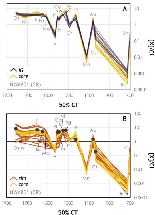
Fig. 7. Concentrations normalized to CI chondrites in CR chondrite metal grains from NWA 801 plotted against the 50% condensation temperature of siderophile and chalcophile elements (Lodders, 2003). (A) Core metal grains versus isolated grains (IG) and (B) core metal grains versus rim grains. Black dots are averaged core compositions from Jacquet et al. (2013). Each line corresponds to a single grain. The data encompasses grains from 3 chondrule cores, 4 chondrule rims (of which one chondrule-rim pair ch1, see Appendix Table S4) and 3 isolated grains.
