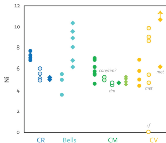
Fig. 6. Ni of core (solid spheres), rim (open spheres) and isolated metal (diamonds) from CR, Bells, CM (light green for Maribo) and CV chondrites.
