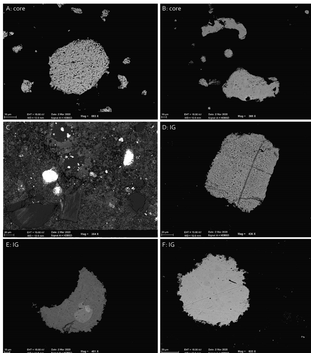
Fig. 3. Back scattered electron images of representative Bells metal grains. A and B are grains from chondrule cores ch1 and ch2, with and without black inclusions. C is an overview of the Bells chondrite section, showing a high-porosity altered matrix with metal-rich chondrules and isolated chondrule grains. D, E and F are isolated grains (IG: met3, met6, met7) within the matrix with irregular boundaries due to oxidation and with or without black inclusions. High resolution BSE images of all Bells metal grains used in this study can be found in Fig. S7.
