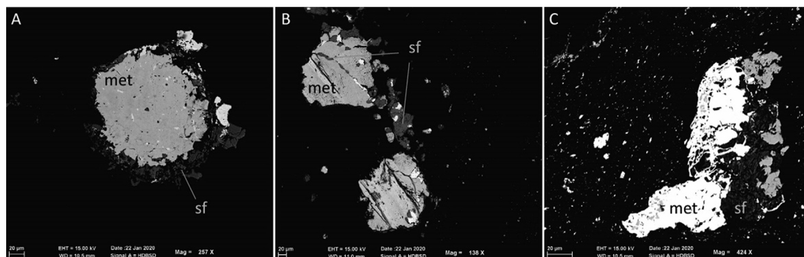
Fig. 12. Metal grains from Leoville that show secondary alteration features of metal being modified to sulfide. (A) Chondrule C5 core grain with sulfide rim, (B) Chondrule Ch4 rim grains intersected by sulfide veins and (C) Isolated metal grain (not analyzed in this study) partially altered to micron sized sulfide grains.
