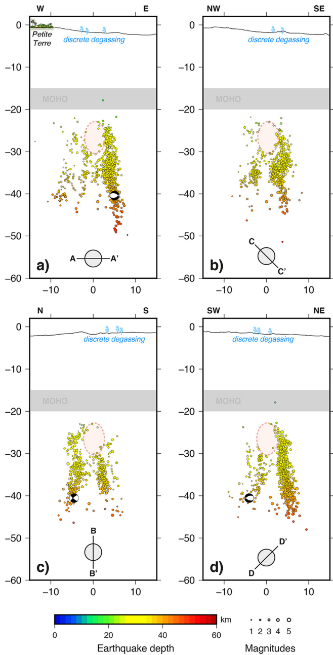
Fig. 7. 1.5 km-wide cross-sections across the proximal cluster with a) profile AA', b) profile CC', c) profile BB' and d) profile DD'. The earthquakes are colour-coded by depth and scaled by magnitude. The symbol at the bottom of each section represents the line of cross-section (line) through the cluster (circle). The Moho interface from the ALav velocity model is indicated in gray. The focal mechanism of the May 14th, 2019 M_w 4.9 event, relocated with the new velocity model, is indicated. The structure highlighted in light red is discussed in the text. Note that 0 depth is the sea level.
