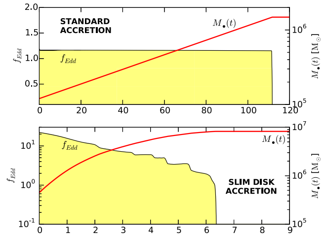
Figure 1. Time evolution of the Eddington factor f_{\text{Edd}} and of the black hole mass M_\bullet , in the standard accretion – LDP (top) and the slim disc accretion – LDP (bottom) scenarios. The Eddington ratio is reported as a running average over periods of \sim 0.1 \text{ Myr} .
