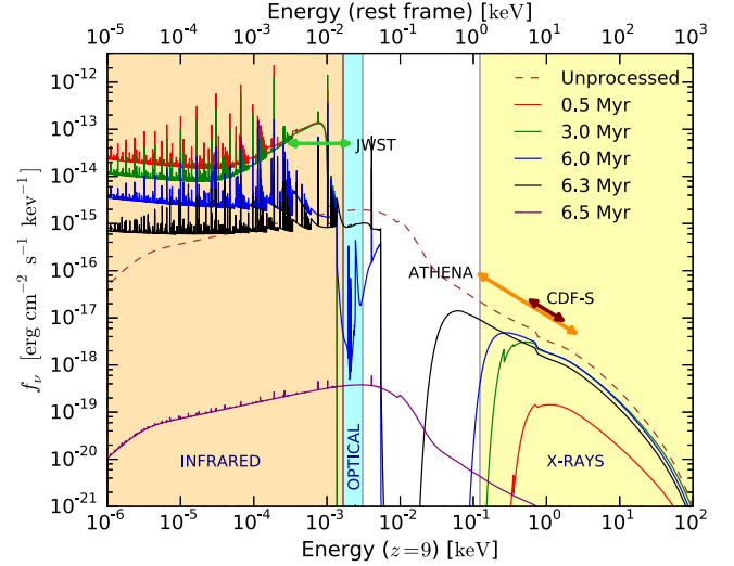
Figure 4. As in Fig. 3, but for the slim disc accretion – LDP case.
