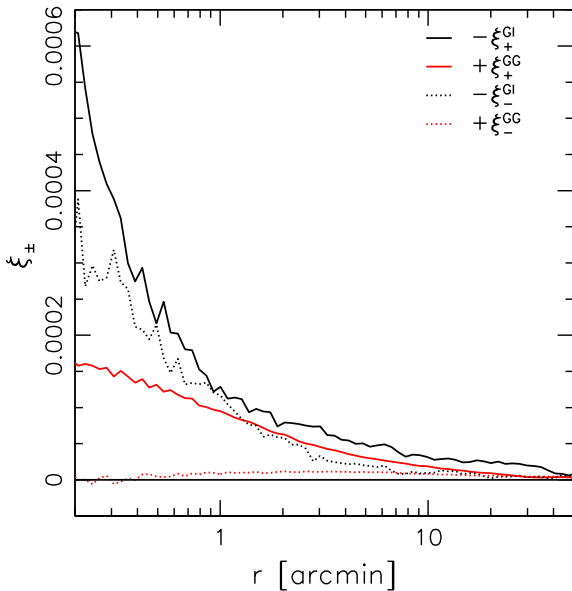
Figure 8. Shear–shear and shape–shear correlation functions \xi_{\pm}^{\text{GG}} and -\xi_{\pm}^{\text{GI}} for the aligned early-type galaxies in the Millennium Simulation at 0.4 < z_1 < 0.6 with 10.5 < \log_{10} M_* < 11 . For these lenses r_{200c} equals 0.98 arcmin.
