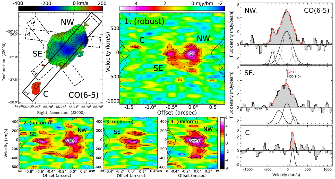
Fig. 3. CO(6–5) kinematics. All velocities are with respect to z = 1.9212 (EM11). Top left: 1st moment velocity map of the CO(6–5) emission, with overlaid contours of the CO(6–5) total intensity at the same levels as those shown in Fig. 2. Also indicated are four pseudo-slits along which we extracted the position-velocity plots shown in the middle and bottom (solid for the robust +0.5 weighted data and dashed for the uniform weighted data). The width of the pseudo-slits indicates the spatial resolution. Top middle: position-velocity plot of the robust +0.5 weighted CO(6–5) data set, which highlights the bridge-like structures between NW and SE at v < -250 \text{ km s}^{-1} and v \sim 0 \text{ km s}^{-1} (PA = -41^\circ ; direction SE to NW). Contour levels: -4, -3, 3, 4, 5, 6, 7, 8, 9\sigma , with \sigma = 0.54 \text{ mJy beam}^{-1} . For guidance, along the y -axis we plot the velocity coverage of the Gaussian model components shown in the spectra on the right. Bottom: position-velocity plots derived from the uniform weighted CO(6–5) data, which best show the kinematic details (beamsize 0.27'' \times 0.23'' at \text{PA}_{\text{beam}} = 57^\circ ). The PV-plots are taken along the dashed axes indicated in the top-left plot and all offsets are shown from (north/south)-east to (south/north)-west. Contour levels: -3, -2, 2, 3, 4, 5, 6, 7\sigma , with \sigma = 0.88 \text{ mJy beam}^{-1} . Right: CO(6–5) spectra of the three components (NW, SE and C). The redshifts z_{\text{CO}(1-0)} (EM11) and z_{\text{HeII}} (EM15), and their uncertainty, are indicated with an arrow + bar. Also shown are the best-fit model (solid red line) and corresponding individual components (solid black Gaussian lines), as well as an alternative model for NW (dotted lines); see text for details.
