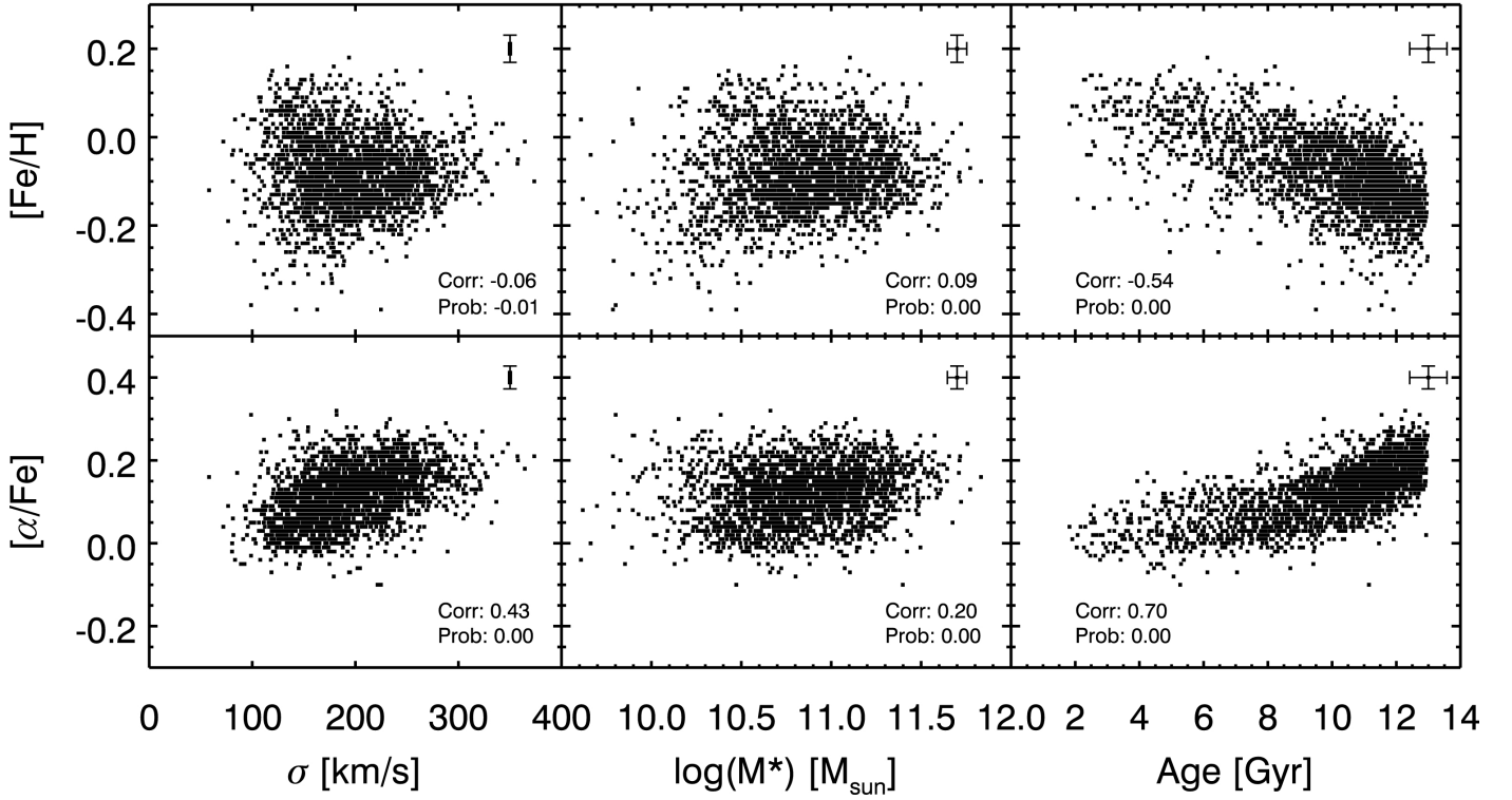
Fig. 12. Correlations of [\text{Fe}/\text{H}] and [\alpha/\text{Fe}] with velocity dispersion, stellar mass and mean light-weighted age for our sample galaxies. It is clear that the tightest relations are those with age. Note also the change of slope in the relation between age and [\alpha/\text{Fe}] \sim 9 Gyr. Average error bars are given in the upper right corner of each panel and spearman rank correlation coefficients are also noted.
