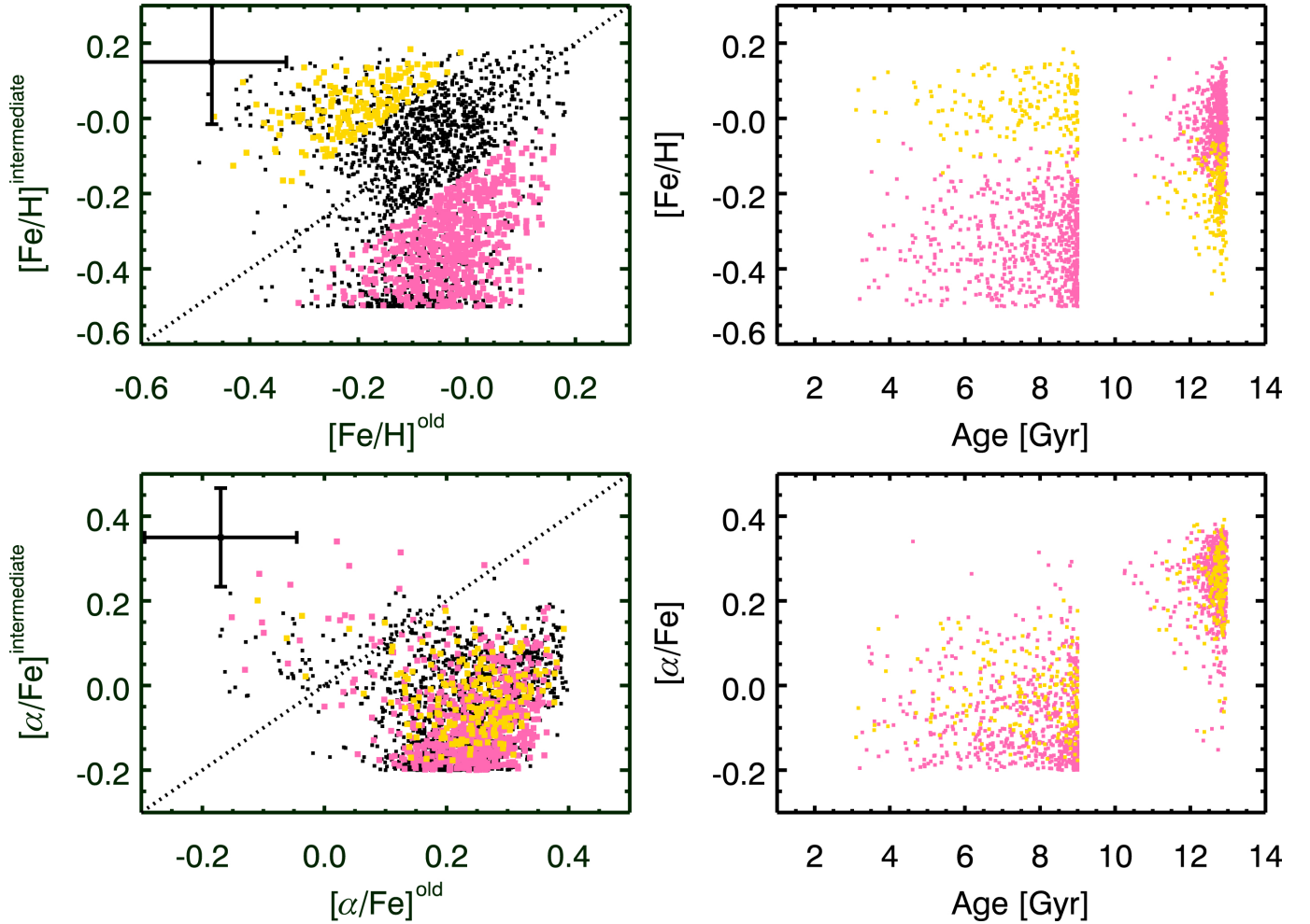
Fig. 17. Left panels: distribution of mean light-weighted [Fe/H] and [alpha/Fe] for the old vs. intermediate sub-populations. Galaxies in yellow are those where [\text{Fe}/\text{H}]_o < [\text{Fe}/\text{H}]_i - 0.15 (SLF-ETGs), pink where [\text{Fe}/\text{H}]_o > [\text{Fe}/\text{H}]_i + 0.15 (ACC-ETGs). Galaxies with uncertain classification are shown in black. Average uncertainties including all degeneracies are shown in the upper left corners. Right panels: age dependence of [Fe/H] and [alpha/Fe] within each galaxy, i.e. their enrichment history. Galaxies with uncertain classification have been omitted for clarity.
