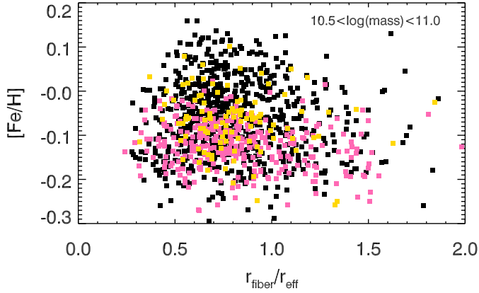
Fig. 21. Dependence of [\text{Fe}/\text{H}] on coverage fraction at fixed mass. No bias is obvious. Colors reproduce the classification from Fig. 17 into SLF-ETGs (yellow) and ACC-ETGs (pink).
