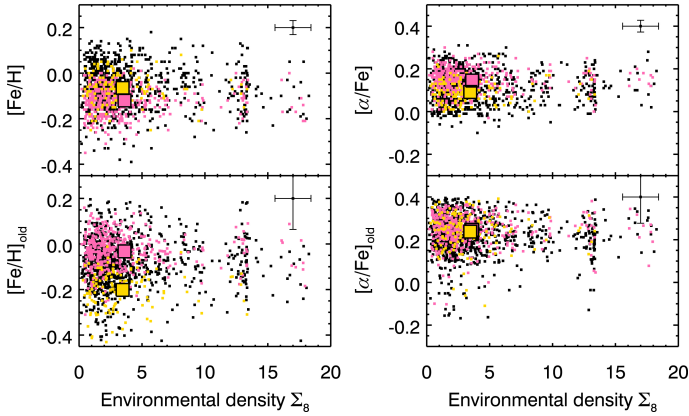
Fig. 19. Environmental density vs. light-weighted [\text{Fe}/\text{H}] and [\alpha/\text{Fe}] (upper panels) and vs. [\text{Fe}/\text{H}]_{\text{old}} and [\alpha/\text{Fe}]_{\text{old}} of only the old stars in each galaxy. The mean for each subpopulation is also shown as a large square with black borders.
