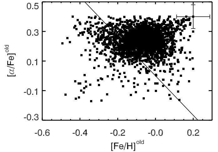
Fig. 16. Relation between [\text{Fe}/\text{H}]_{\text{old}} vs. [\alpha/\text{Fe}]_{\text{old}} , the thick line is a line of constant, solar metallicity ( Z = 0.017 ). This is the same as Fig. 13, but only for the stars older than 9.5 Gyr in each galaxy. The old stars in early-type galaxies, have on average high total metallicity, significantly super-solar. Average error bars are shown in the upper right corner.
