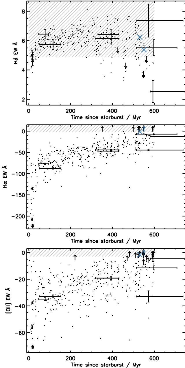
Figure A1. EWs of the H\delta_A , H\alpha and [O II] emission lines as a function of starburst age for the SDSS bulge-dominated PSB parent sample (dots) and the 11 PSBs studied in this paper (thick points with error bars). The grey areas denote the equivalent width at which a galaxy would be identified as a PSB galaxy by Goto et al. (2003). The blue crosses indicate galaxies which meet all three criteria required by Goto et al. (2003) to be classified as a PSB. Upper limits at the 3\sigma level are shown for galaxies with SNR < 3 , sources with blue upper limits have SNR < 3 in either H\alpha or [O II] EW and meet the Goto et al. (2003) criteria at the 3\sigma level.
