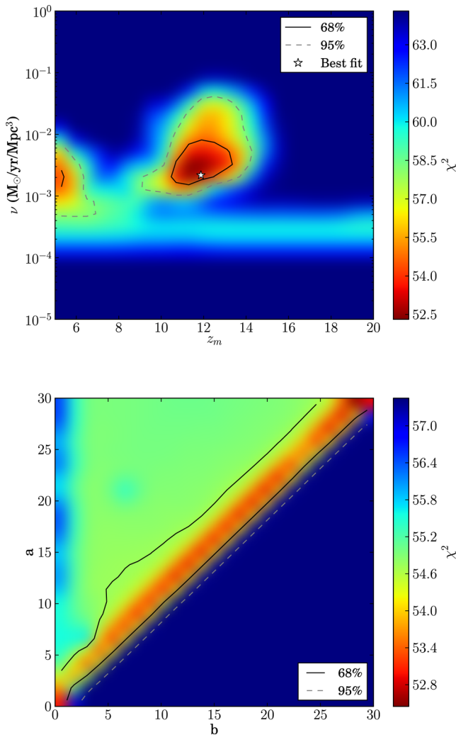
Figure 5. (a) 2D maps of \chi^2 in the \nu , z_m parameter plane (upper) and a , b parameter plane (lower). 68 per cent (solid) and 95 per cent (dashed) frequentist confidence intervals are shown, calculated using \Delta\chi^2 values of 2.30 and 5.99, respectively. The location of the best-fitting point in the upper panel is shown by a star. In the lower panel, the \chi^2 is nearly constant along the diagonal a \gtrsim b .
