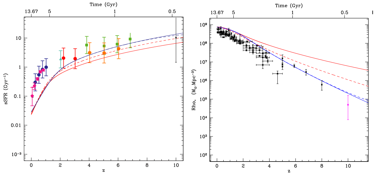
Figure 12. (a) The evolution of the mean sSFR as a function of the redshift for the four models under consideration. Stellar mass of galaxies are in the range of 10^{9.4}-10^{10} M_{\odot} . Data points come from the literature (Daddi et al. 2007; Noeske et al. 2007; Damen et al. 2009; Reddy et al. 2012; Stark et al. 2013; González et al. 2014) and have been compiled in Madau & Dickinson (2014). The z = 10 data point comes from Oesch et al. (2014a). (b) The evolution of stellar mass density as a function of the redshift for the four models under consideration is also shown. The data points are taken from a compilation made by Madau & Dickinson (2014, their table 2) using UV and IR data. The magenta z = 10 data point comes from Oesch et al. (2014a).
