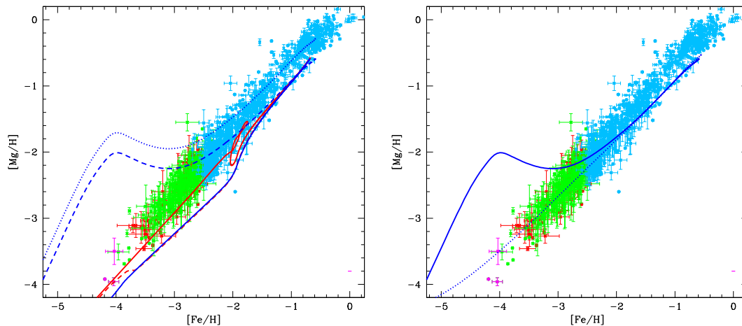
Figure 10. As in Fig. 9, the evolution of the magnesium abundance as a function of the iron abundance for the four models under consideration. In the left-hand panel, we use a Mg yield coming from Woosley & Weaver (1995). The blue dotted curve shows the evolution of Mg using an alternate enhanced yield in the case of model 4, multiplying the yield by a factor 2. In the right-hand panel, we use another yield, coming from Heger & Woosley (2010, blue dotted line) compared with the result from model 4 (solid blue line). Magnesium data points come from the SAGA DataBase (Suda et al. 2008, 2011).
