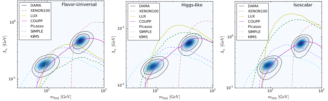
FIG. 1 (color online). Two-dimensional credible regions for DAMA (shaded area and black solid lines, 90% and 99% C.L.) and exclusion limits (99.5% C.L.) in the (m_{\text{DM}}, \Lambda_a) plane, for flavor-universal (left), Higgs-like (center), and isoscalar (right) couplings.
