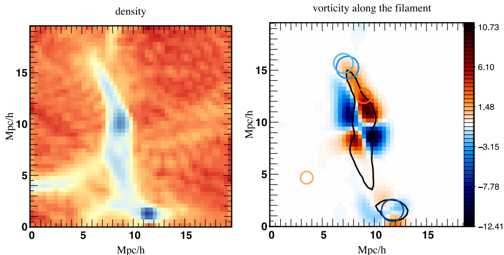
Figure 3. Geometry/kinematics of a typical multi-flow region across a filament. Left: density map of a section perpendicular to a given filament in logarithmic scale. Right: projected vorticity along the filament within that section (towards observer in red and away from the observer in blue) in units of h \text{ km s}^{-1} \text{ Mpc}^{-1} on which is plotted in dark a contour of the density. Circles are haloes with their corresponding virial radius. The colour of the circles matches to the values of \cos \theta between the haloes spins and the normal of the section, positively oriented towards us. S_{100}^{\text{HDM}} is used here, and for this figure only, vorticity is computed after smoothing the velocity field with a Gaussian filter of 1.6 h^{-1} \text{ Mpc} .
