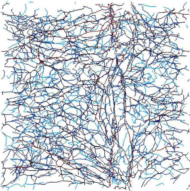
Figure C2. The skeleton measured in \mathcal{S}_{20}^{\text{cool}}(0.7) for increasing persistence threshold, 0.06, 0.12, . . . , 2, from light blue to red; the skeleton has tree-like structure where the main branches correspond to the most persistent ones. The level of persistence of the main text corresponds to the dark blue and red branches.
