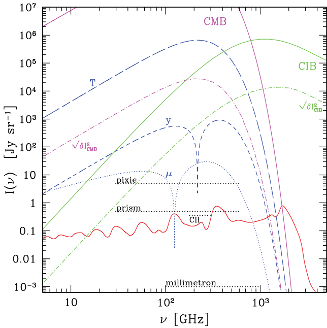
Figure 3. Average intensity as a function of frequency. The various curves represent the CMB and CIB monopole, the T , \mu and y distortions and the recombination spectrum. The dott-dashed curves labelled as \sqrt{\delta I_{\text{CMB}}^2} and \sqrt{\delta I_{\text{CIB}}^2} indicate the rms variance of CMB and CIB fluctuations measured in a 16 \text{ deg}^2 patch of the sky with a beam FWHM of 0.5 arcmin. The horizontal dotted lines show the frequency coverage and sensitivity expected for the PIXIE, PRISM and MILLIMETRON space experiments, as well as for a ground-based C II experiment. Note that the galactic dust monopole (not shown on this figure) is a grey-body similar to, though usually brighter than, the CIB (see Fig. 2).
